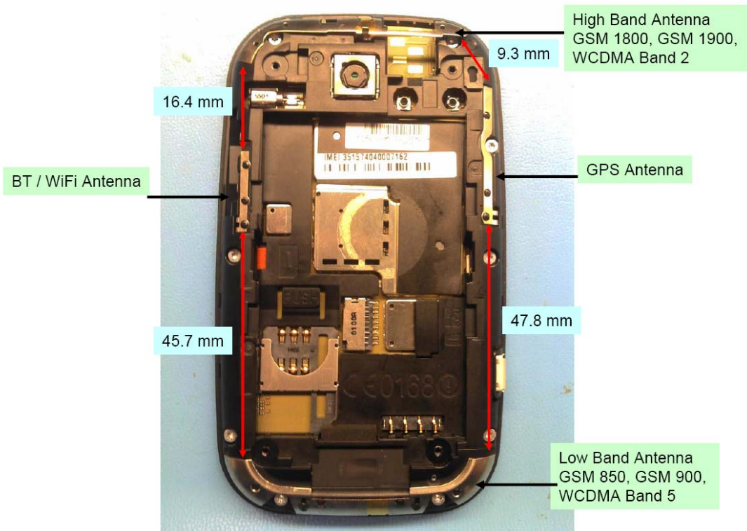
Figure 2: Antenna Separation Distances
