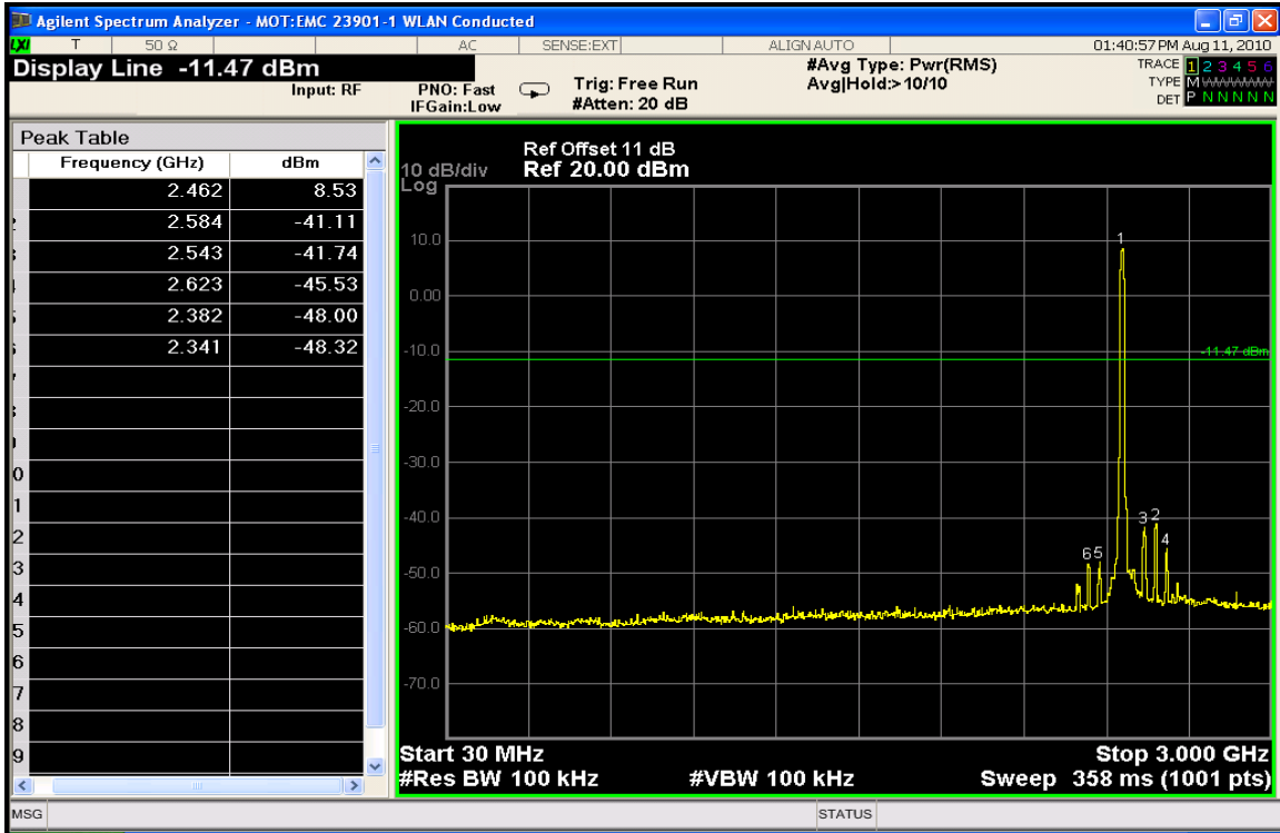
Conducted Spurious Emissions 30-3000 MHz (High Channel)
