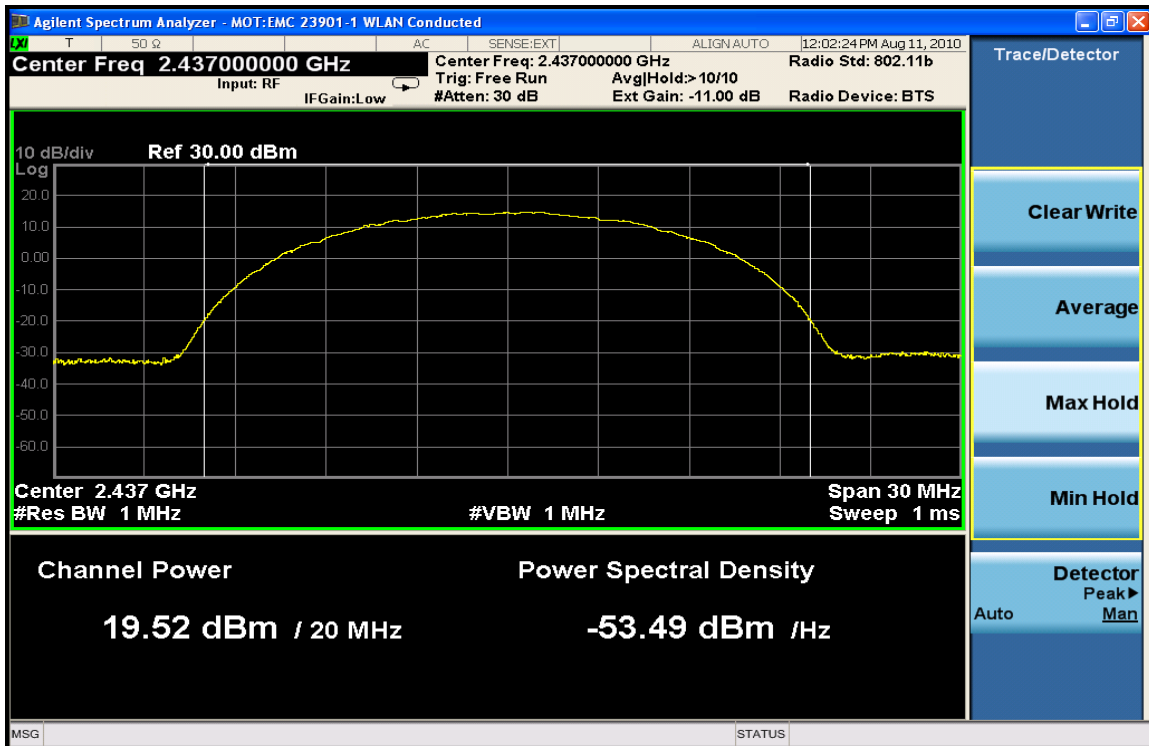
Max. Power Channel 6 @ 11 Mbps
