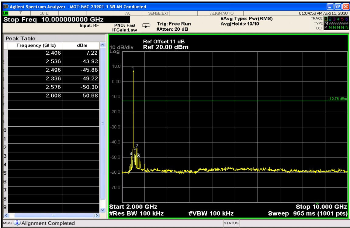
Conducted Spurious Emissions 2-10 GHz (Low Channel)
