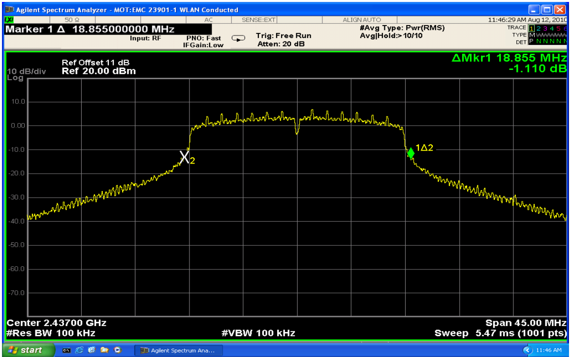
20 dB Bandwidth Channel 6 @ 6.5 Mbps
