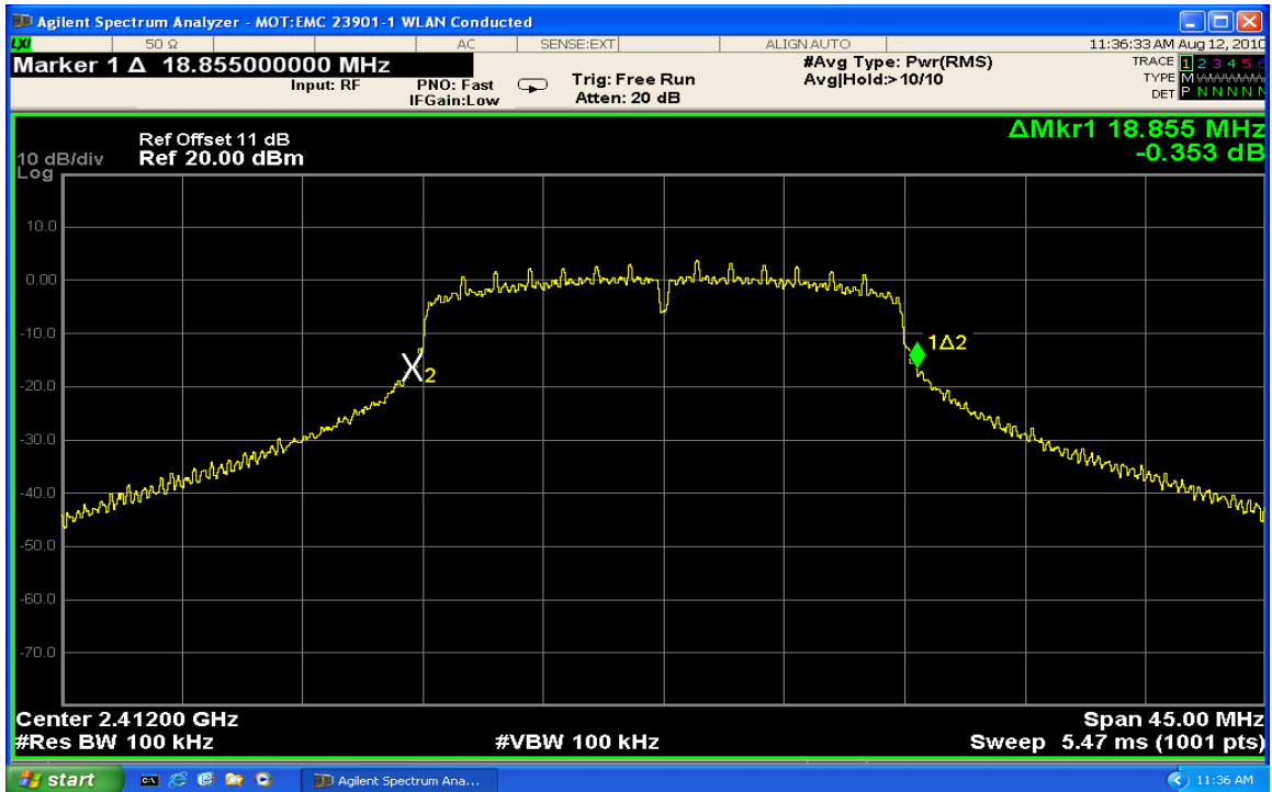
20 dB Bandwidth Channel 1 @ 6.5 Mbps
