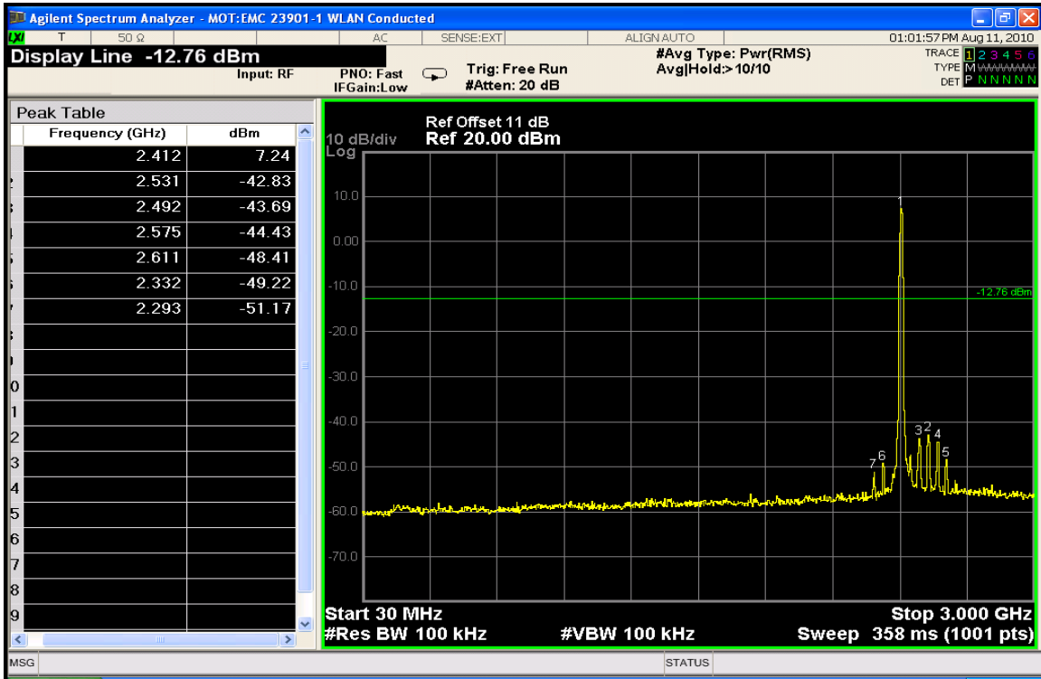
Conducted Spurious Emissions 30-3000 MHz (Low Channel)
