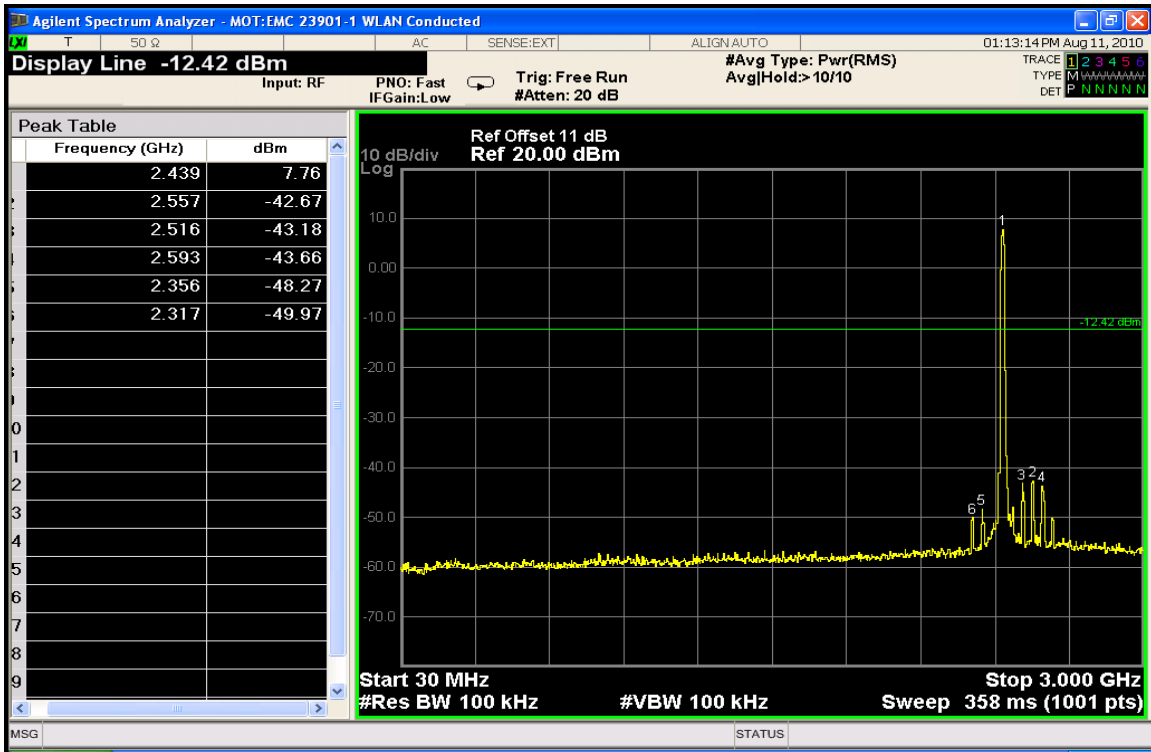
Conducted Spurious Emissions 30-3000 MHz (Mid Channel)
