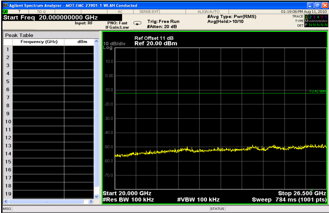
Conducted Spurious Emissions 20-26.5 GHz (Mid Channel)
