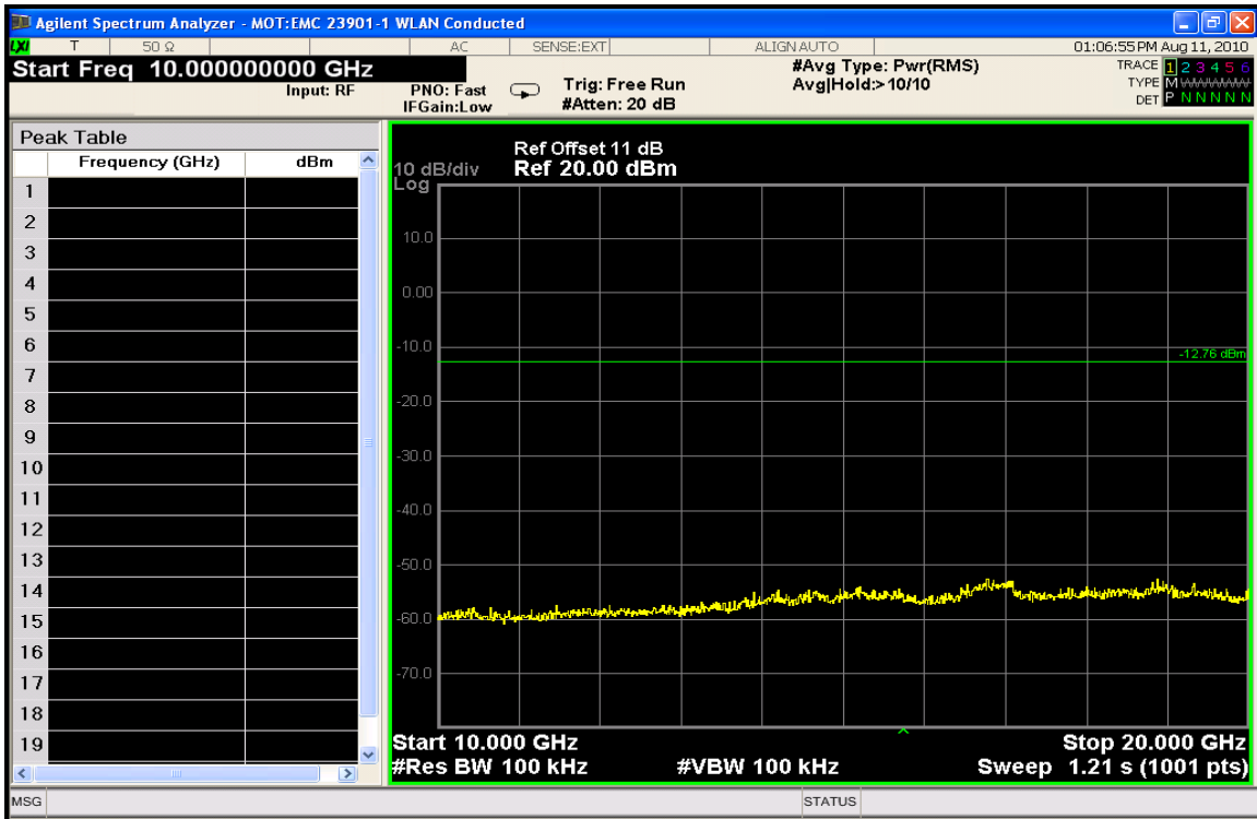
Conducted Spurious Emissions 10-20 GHz (Low Channel)
