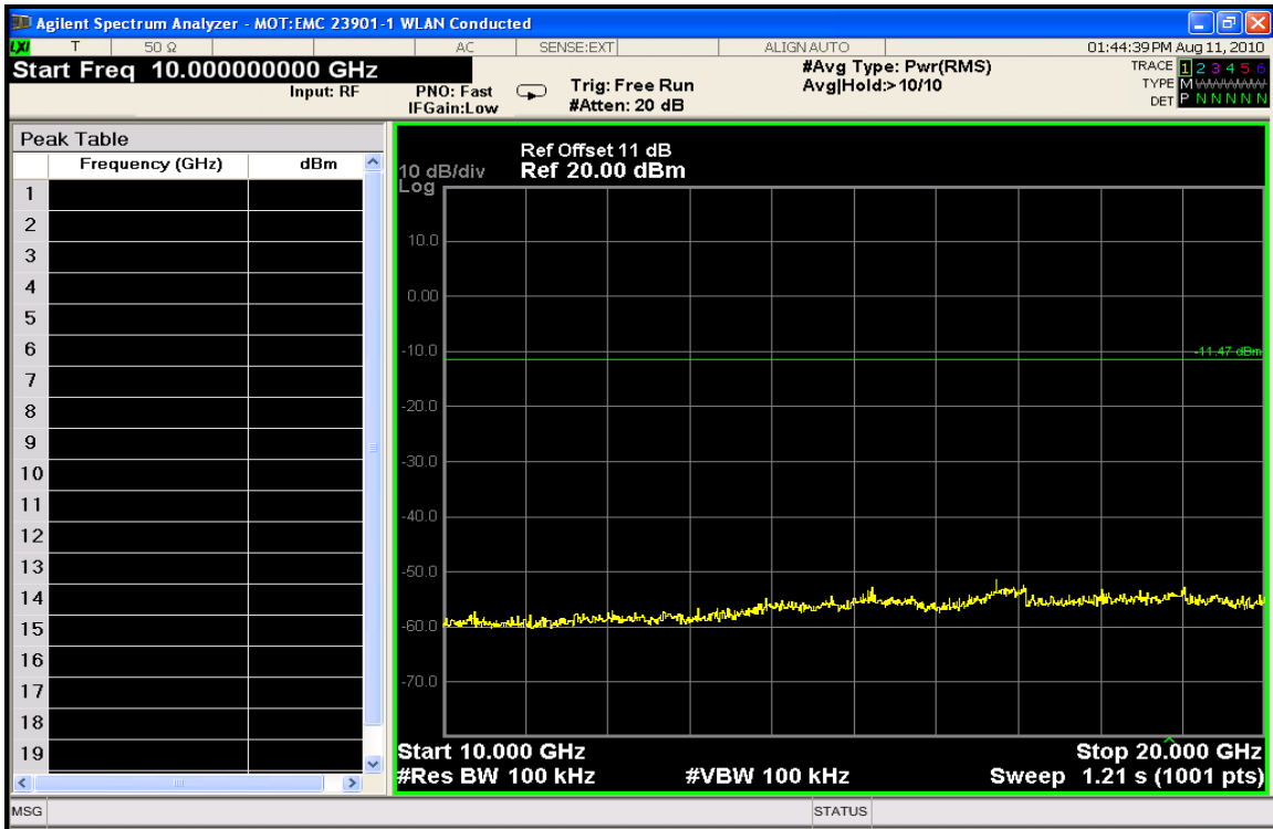
Conducted Spurious Emissions 10-20 GHz (High Channel)
