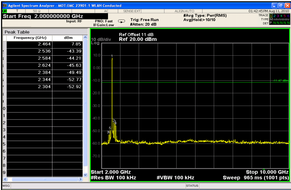
Conducted Spurious Emissions 2-10 GHz (High Channel)
