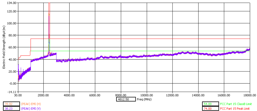
30 - 18000MHz Low Channel Dual Polarization X
