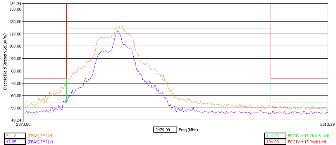
Low Band Edge X Orientation Peak Detector
