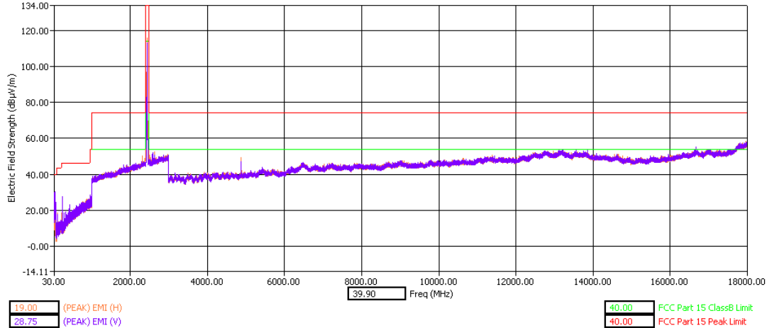
30 - 18000MHz Middle Channel Dual Polarization X
