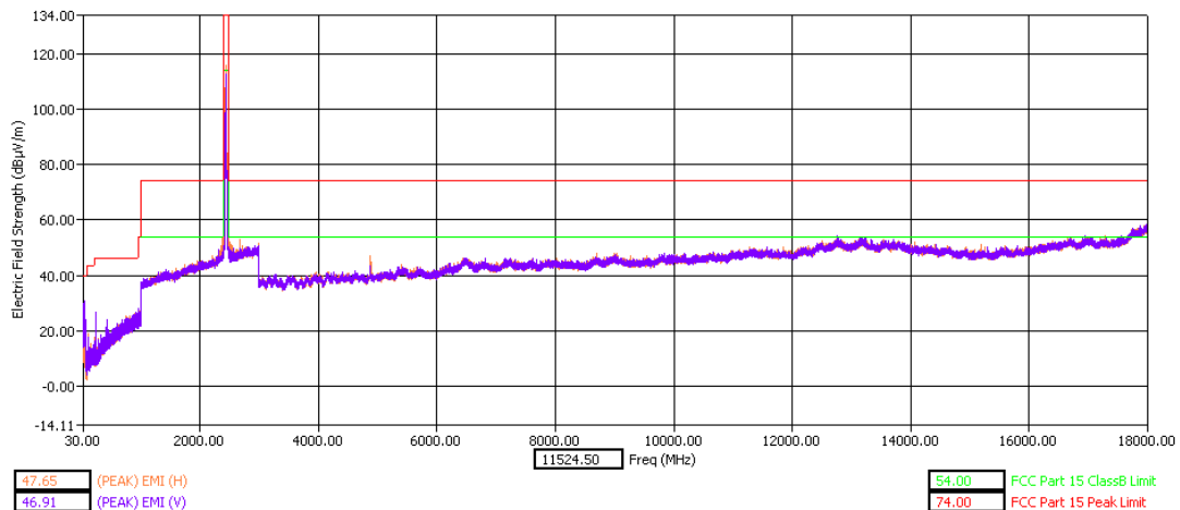
30 - 18000MHz Middle Channel Dual Polarization Z
