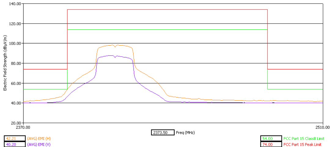
Low Band Edge X Orientation Average Detector
