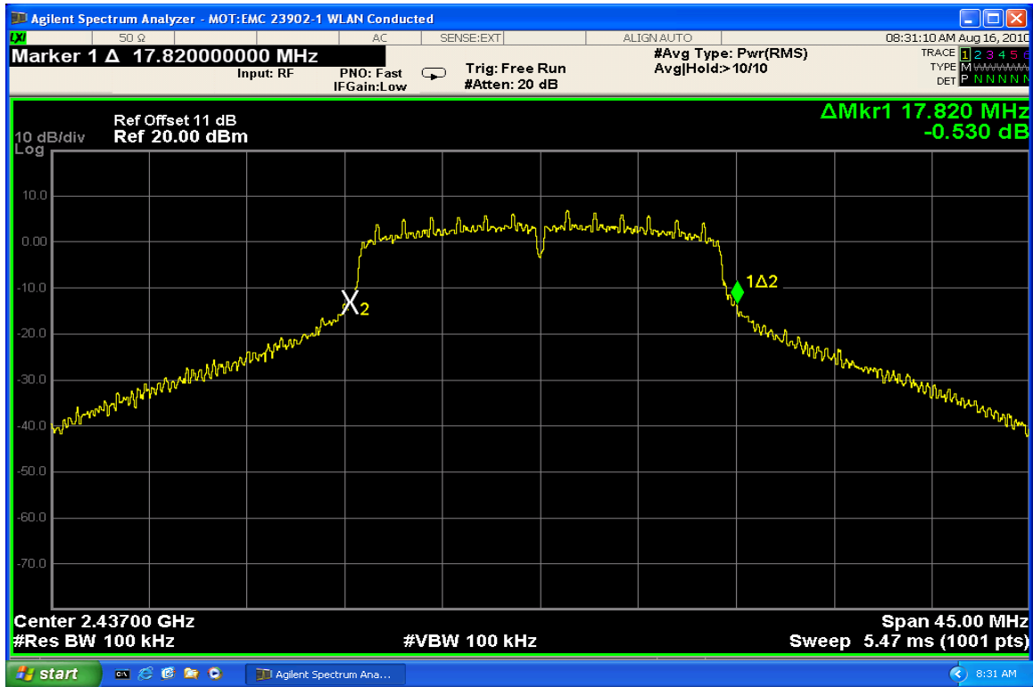
dB Bandwidth Channel 6 @ 9Mbps
