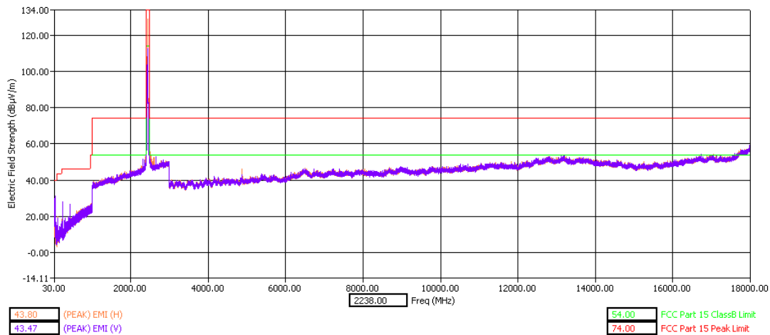
30 - 18000MHz Middle Channel Dual Polarization Y
