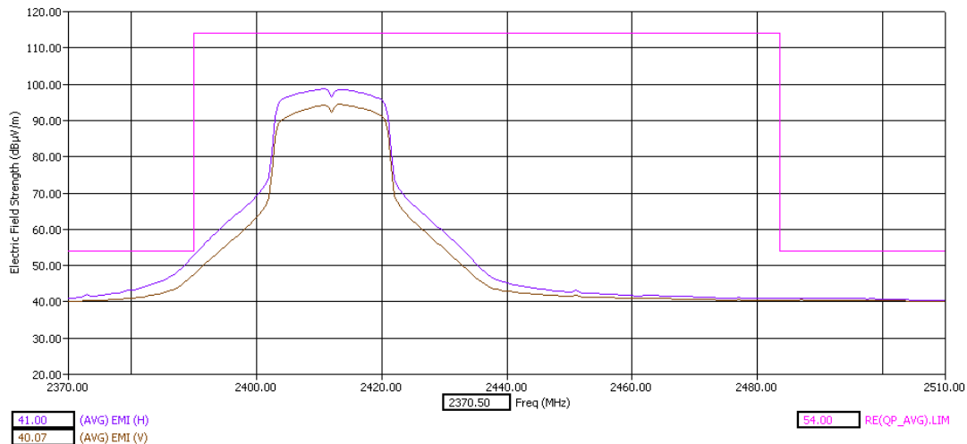
Low Band Edge Z Orientation Average Detector
