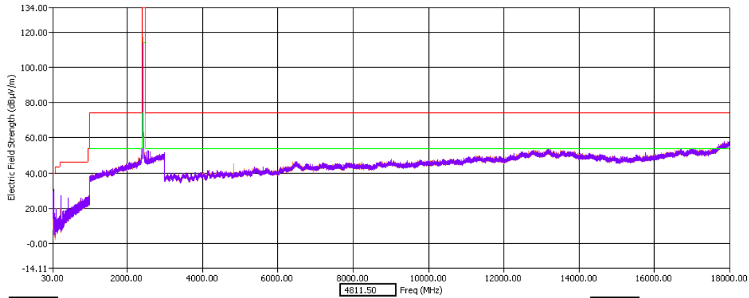
30 - 18000MHz Low Channel Dual Polarization Z
