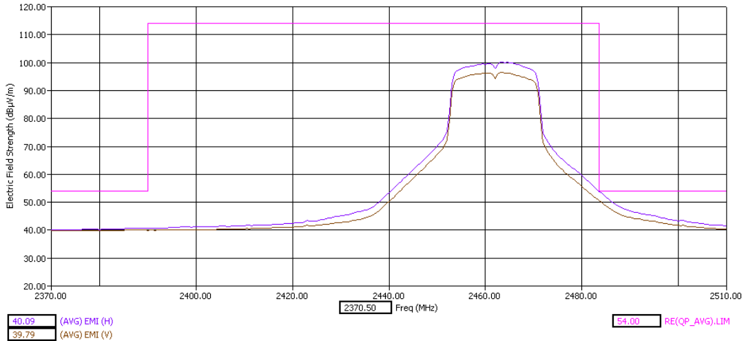
High Band Edge Z Orientation Average Detector
