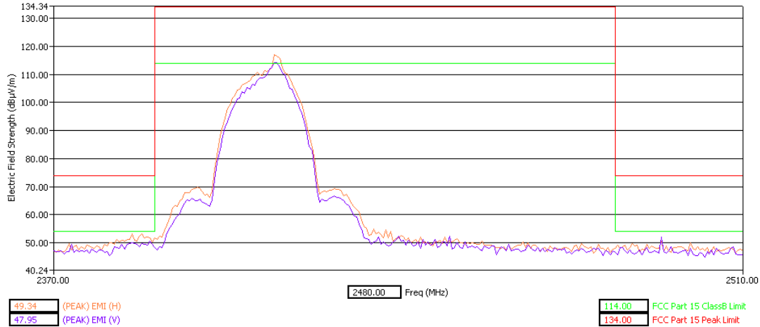
Low Band Edge Z Orientation Peak Detector
