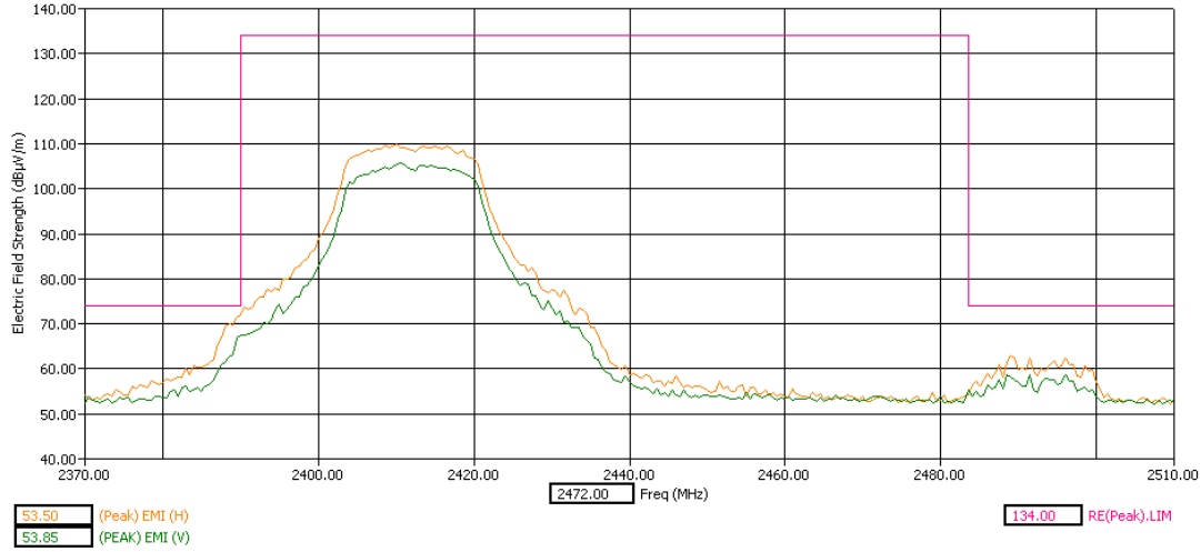
Low Band Edge Z Orientation Peak Detector
