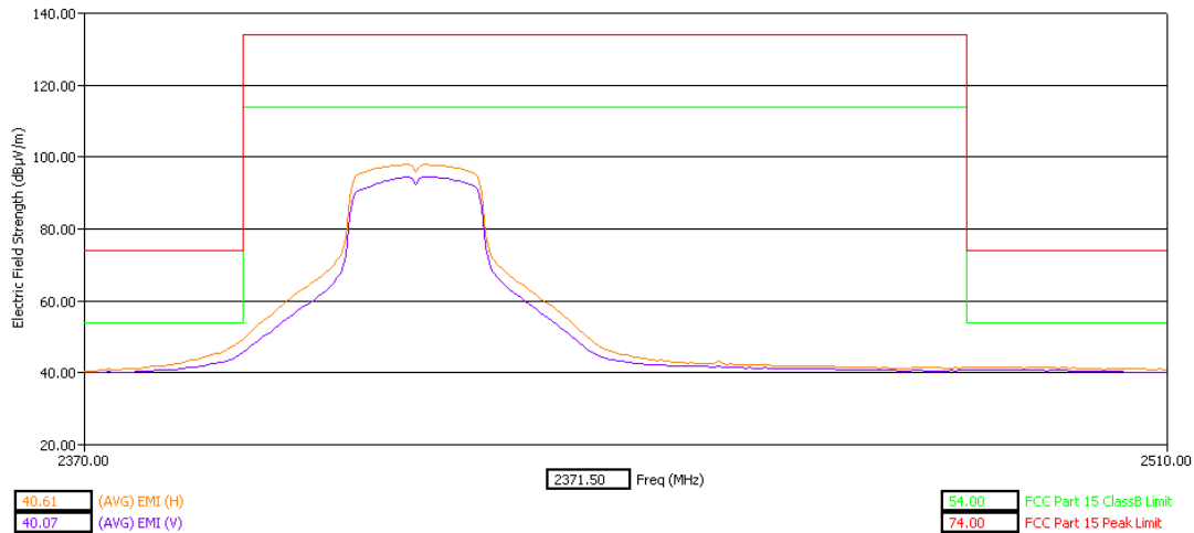
Low Band Edge Z Orientation Average Detector
