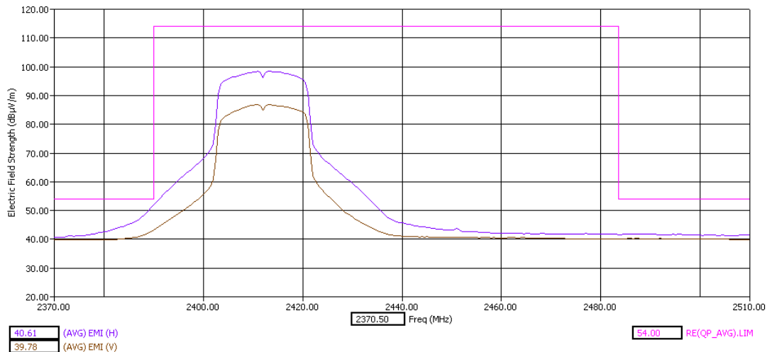
Low Band Edge X Orientation Average Detector
