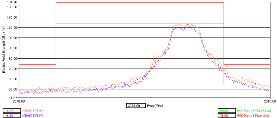
High Band Edge Z Orientation Peak Detector
