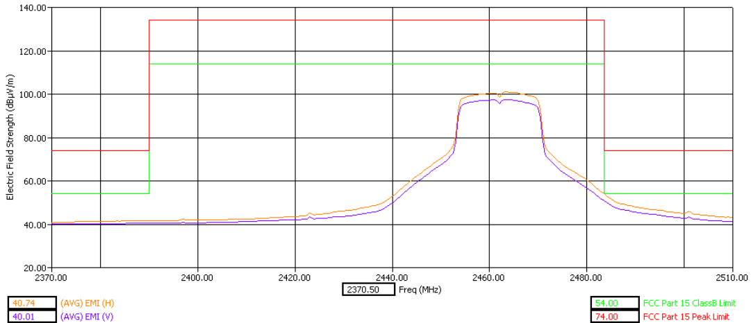
High Band Edge X Orientation Average Detector
