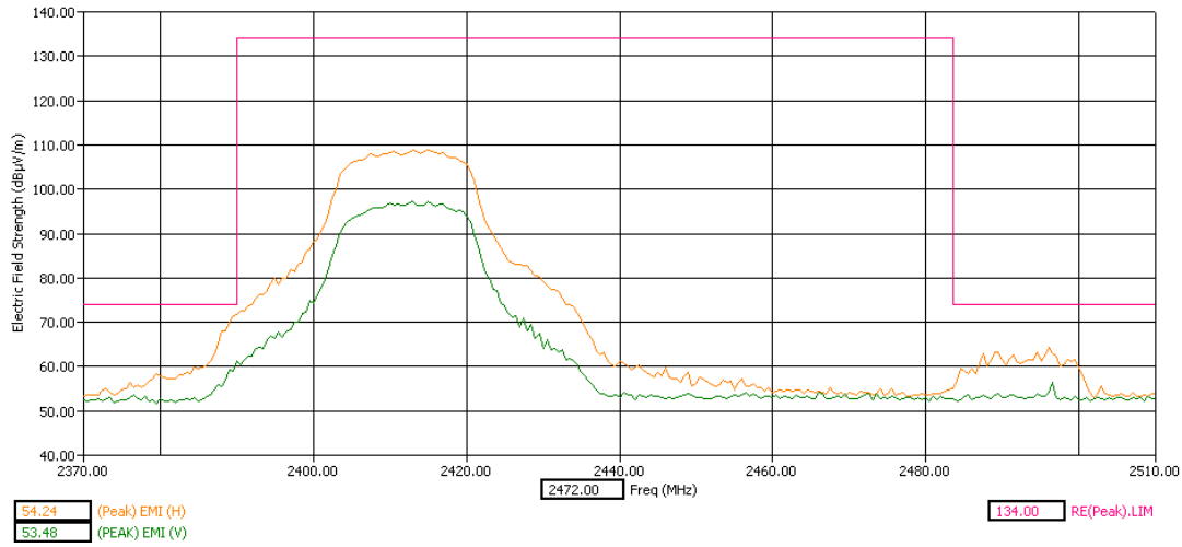
Low Band Edge X Orientation Peak Detector
