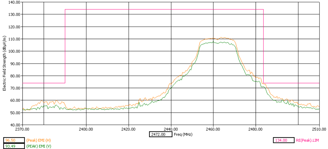
High Band Edge Z Orientation Peak Detector
