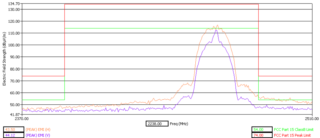
High Band Edge X Orientation Peak Detector
