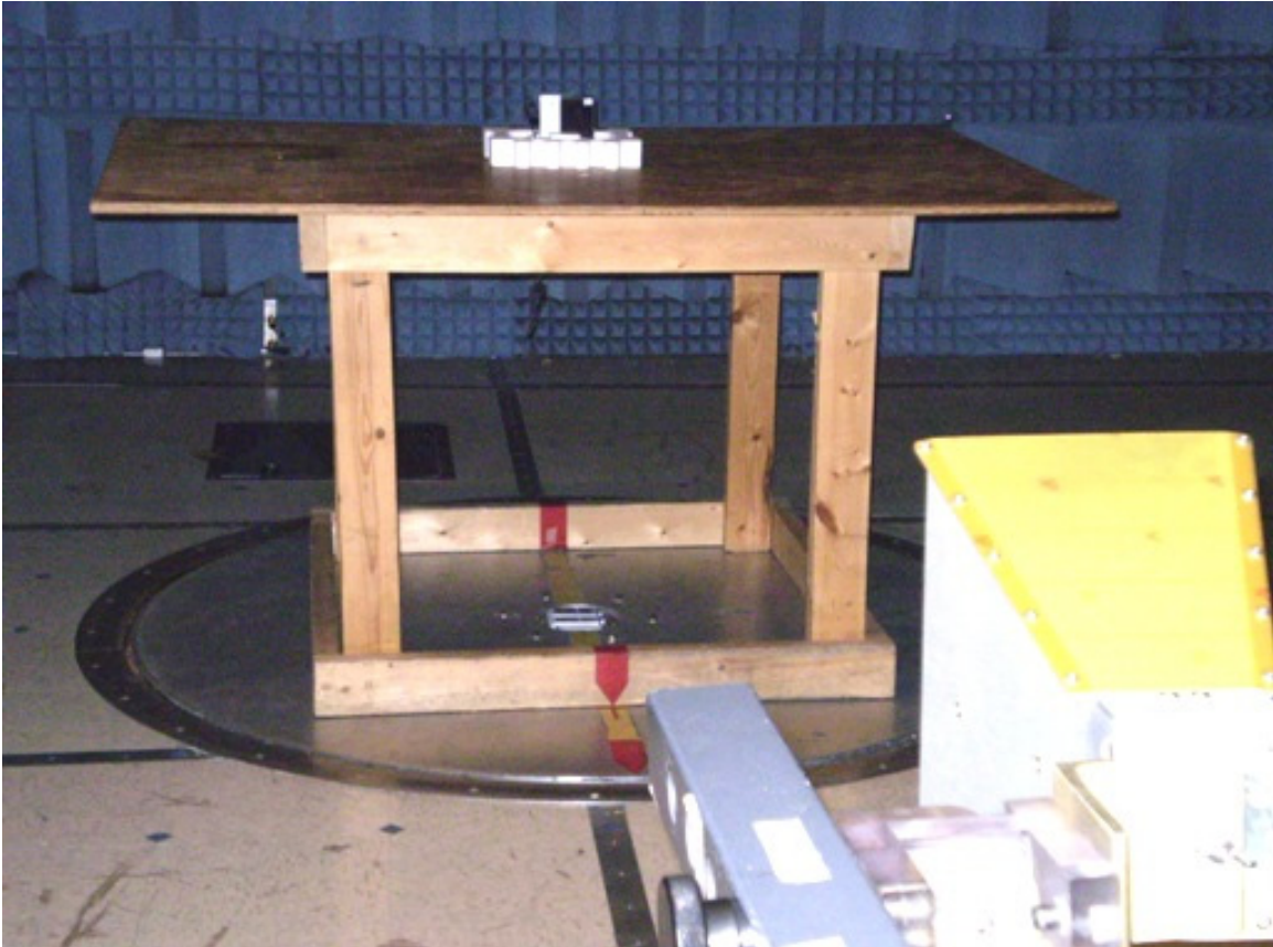
Tx Radiated
