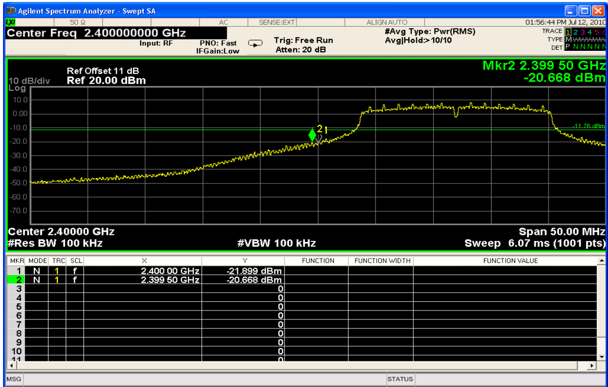
Channel 1 @ 9 Mbps – Lower Band Edge
