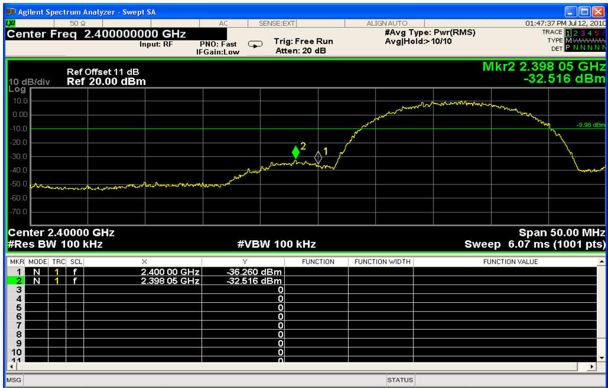
Channel 1 @ 11 Mbps – Lower Band Edge
