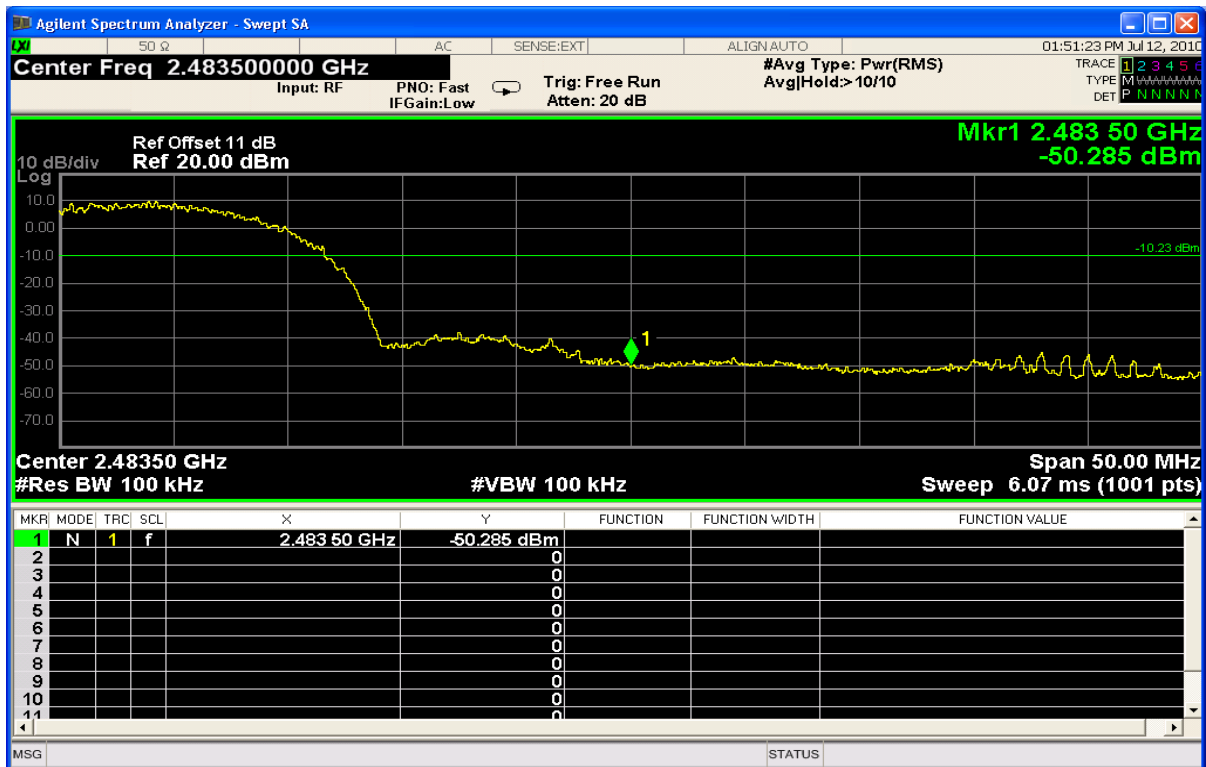
Channel 11 @ 11 Mbps – Upper Band Edge
