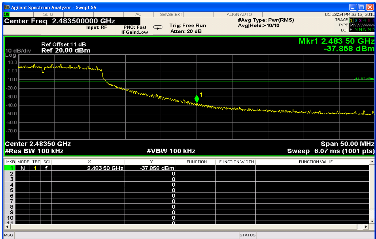
Channel 11 @ 9 Mbps – Upper Band Edge
