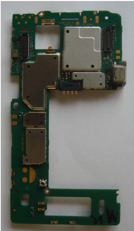
Main Board Top With Shield
