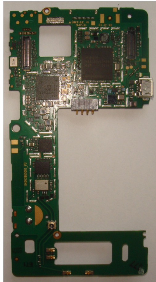
Main Board Top Without Shield
