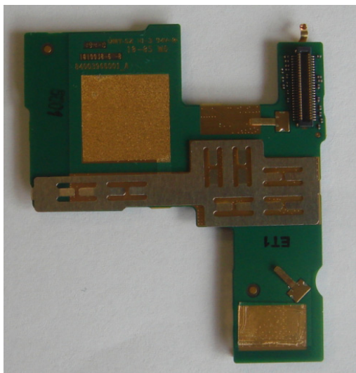
Daughter PCB Back
