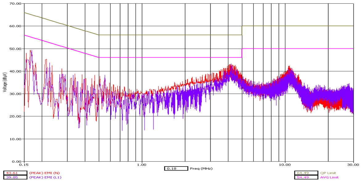
WLAN Channel 6 - Tx Mode - Peak Detector
