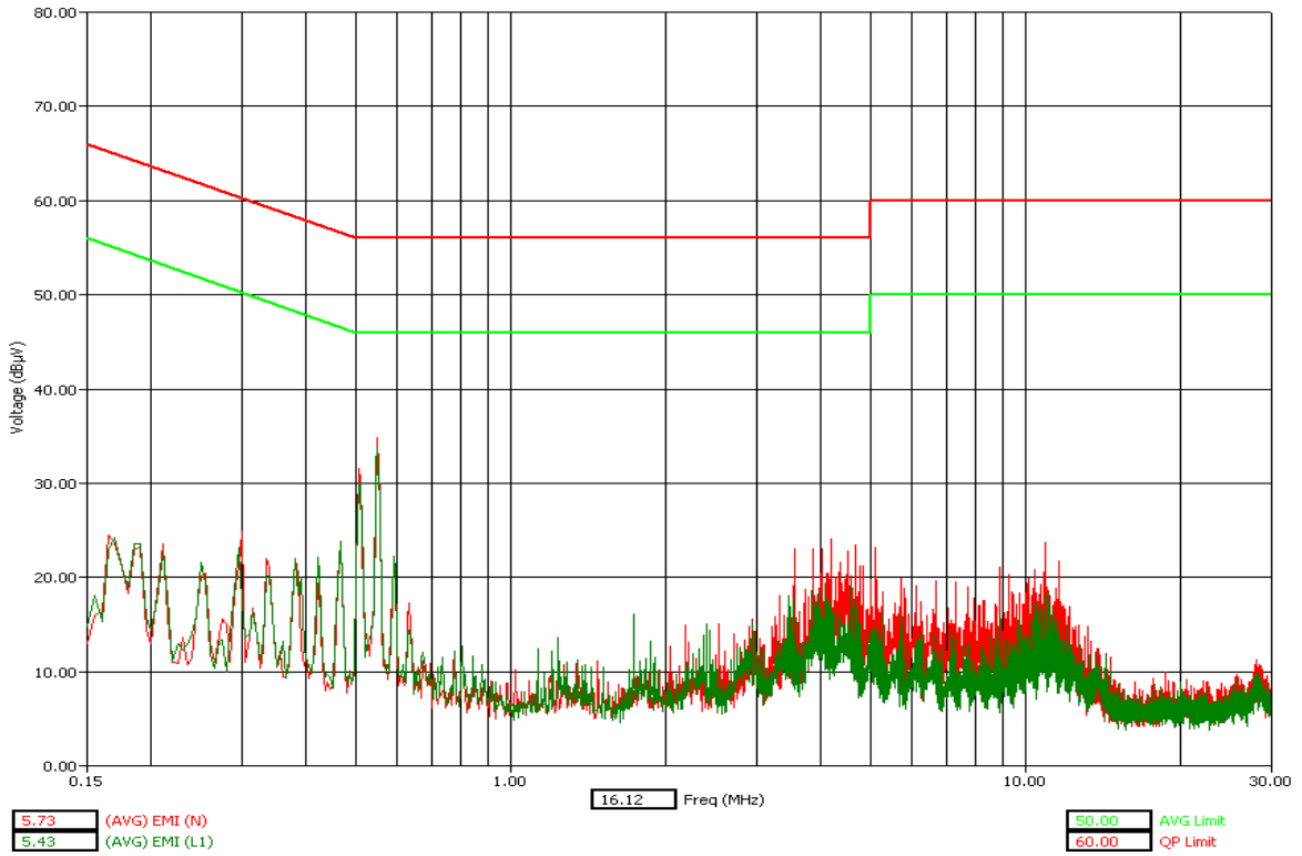
WLAN Channel 11 - Tx Mode - AVG Detector
