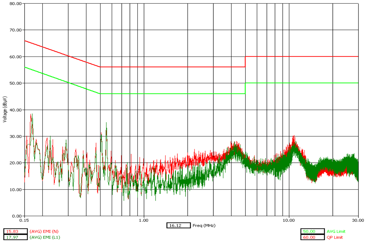
WLAN Channel 6 - Tx Mode - AVG Detector
