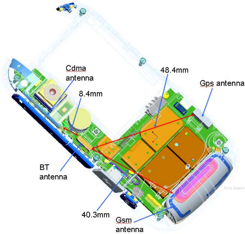
Figure 7: Antenna Separation Distances
