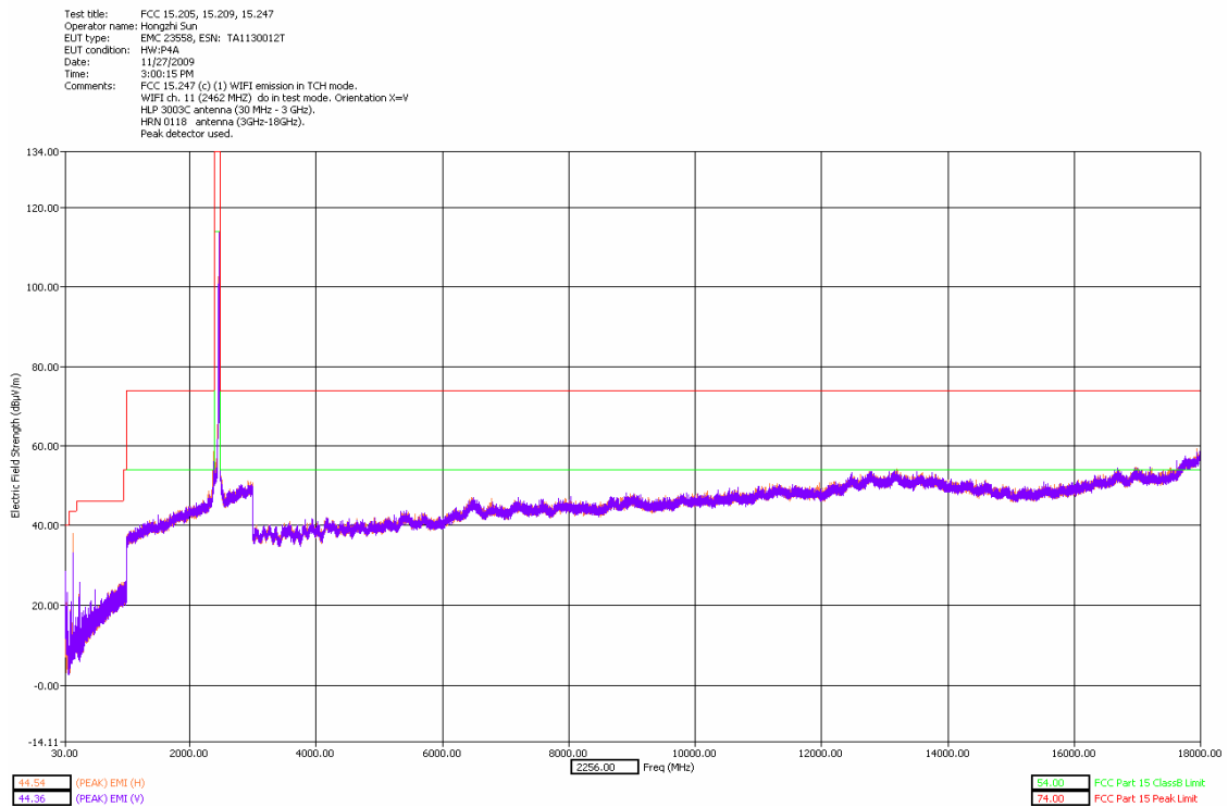
30 - 18000MHz High Channel Dual Polarization X
