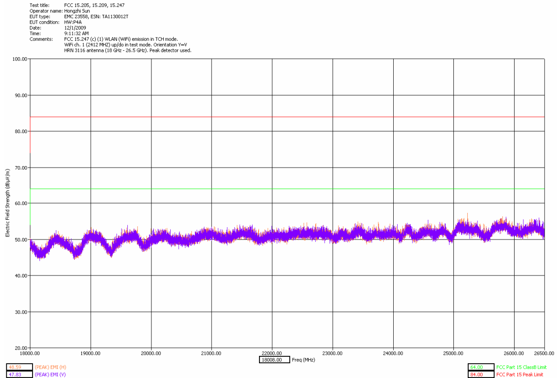
18-26.5GHz Low Channel Y Orientation
