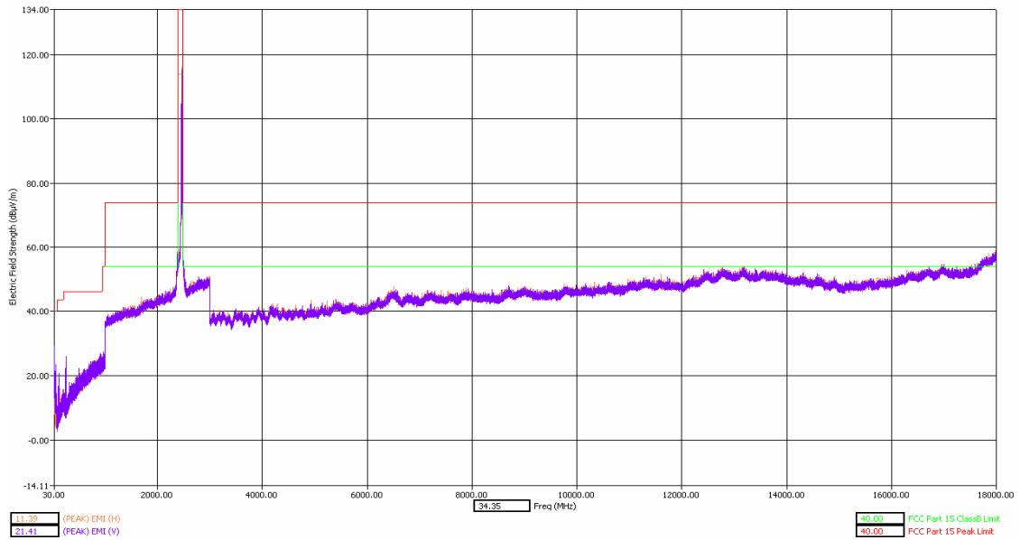
30 - 18000MHz High Channel Dual Polarization Z
