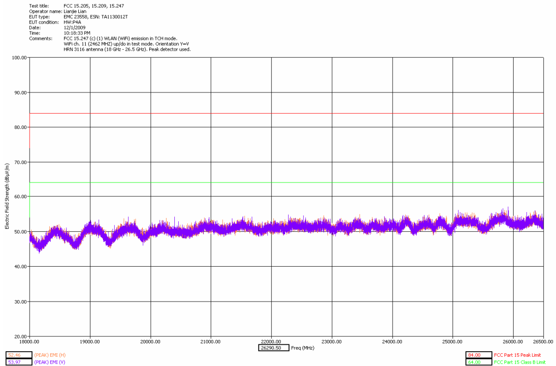
18-26.5GHz High Channel Y Orientation
