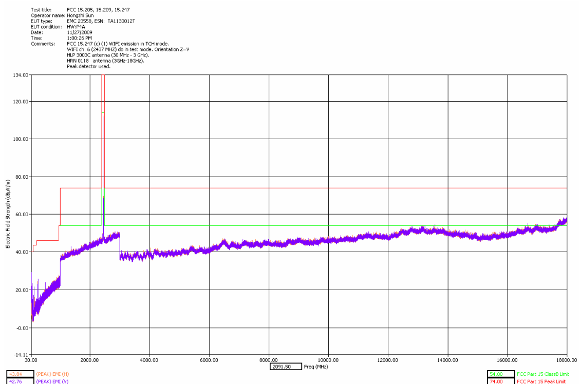
30 - 18000MHz Middle Channel Dual Polarization Z
