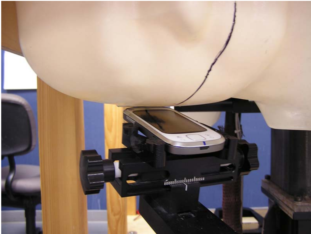
Figure 4: Tilt Position
