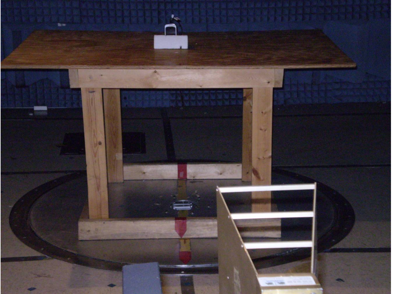
Radiated Emissions
