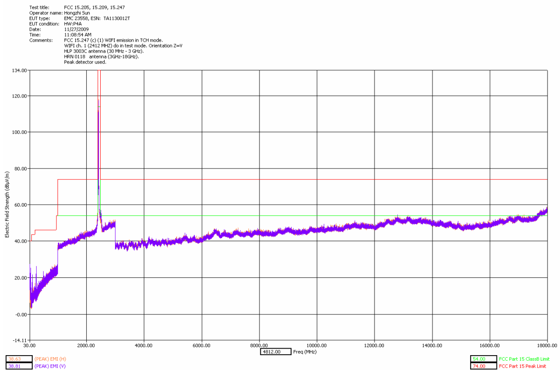
30 - 18000MHz Low Channel Dual Polarization Z
