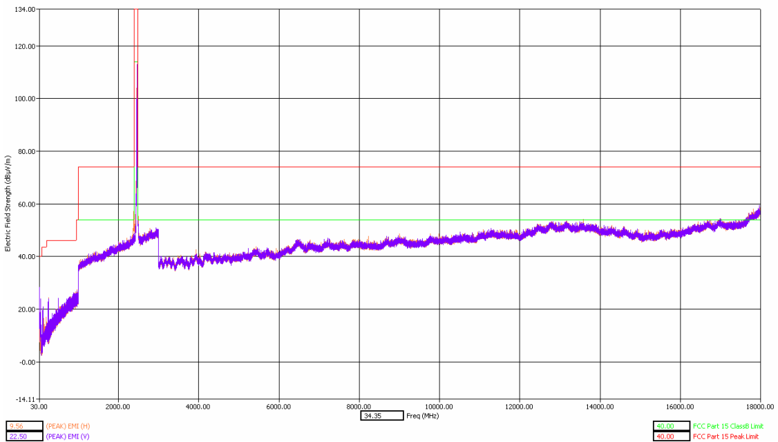
30 - 18000MHz High Channel Dual Polarization X
