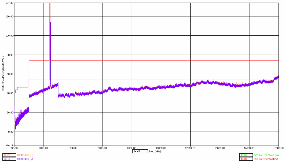
30 - 18000MHz High Channel Dual Polarization Z
