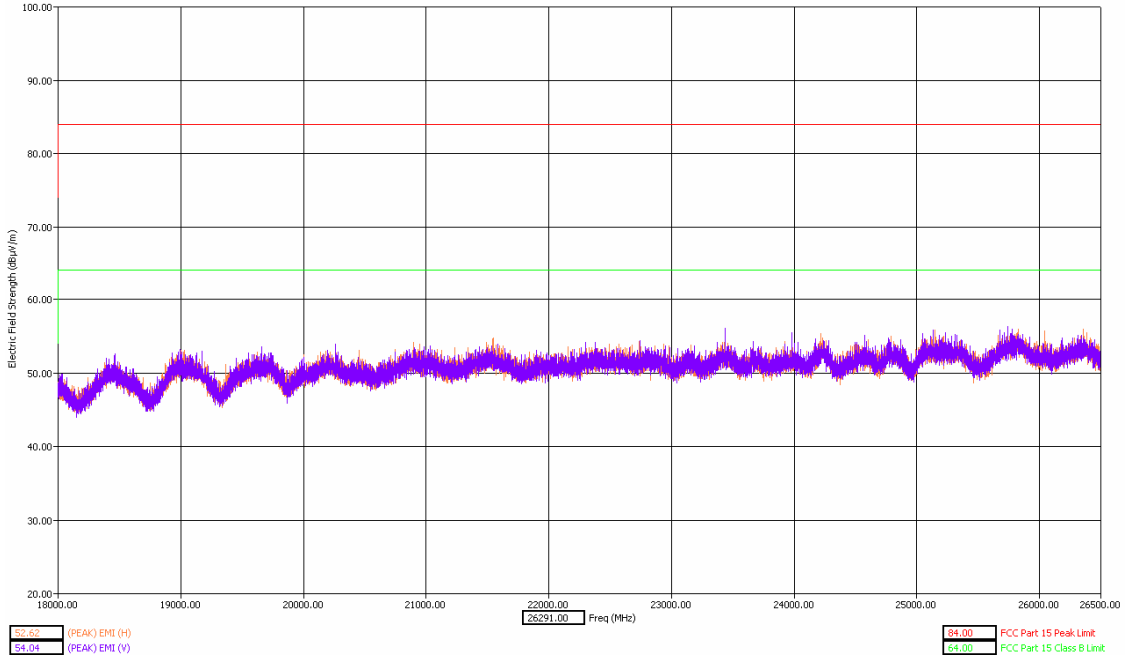
18 – 26.5 GHz Middle Channel Dual Polarization Y
