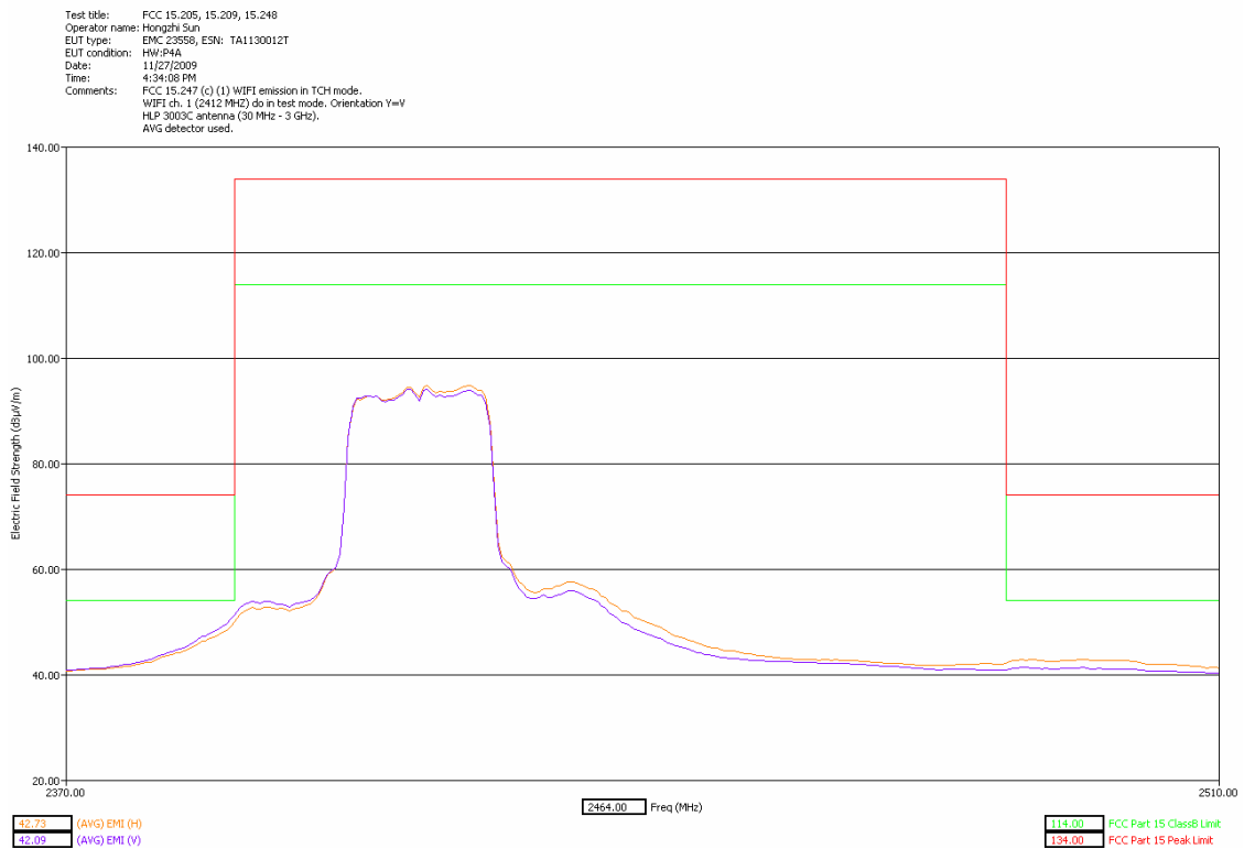
Low Band Edge Y Orientation
