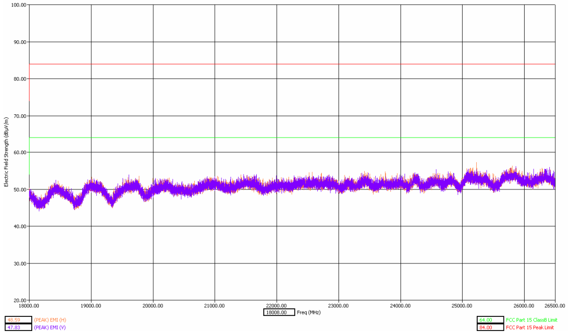
18-26.5GHz Low Channel Y Orientation
