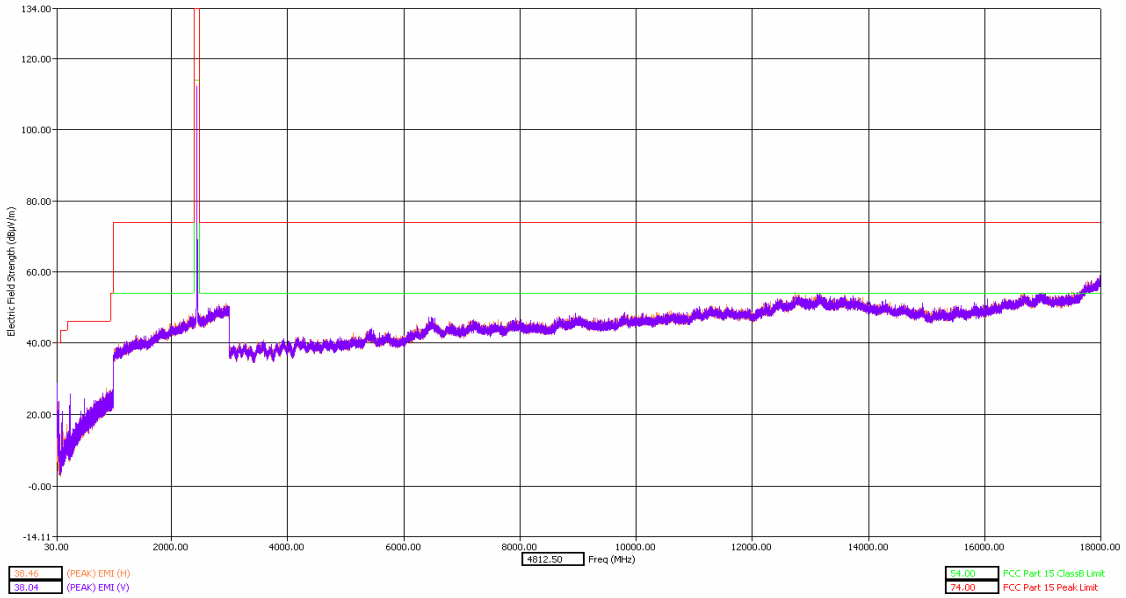
30 - 18000MHz Middle Channel Dual Polarization Y
