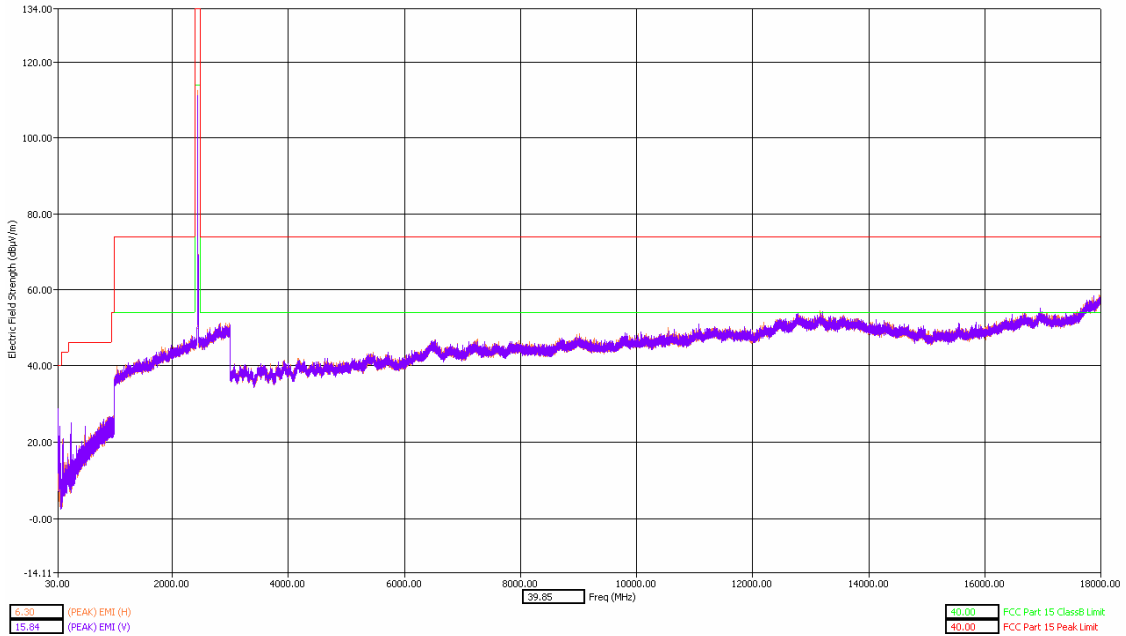
30 - 18000MHz Middle Channel Dual Polarization Z
