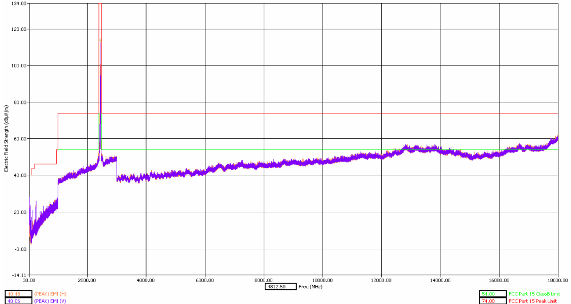
30 - 18000MHz Middle Channel Dual Polarization X
