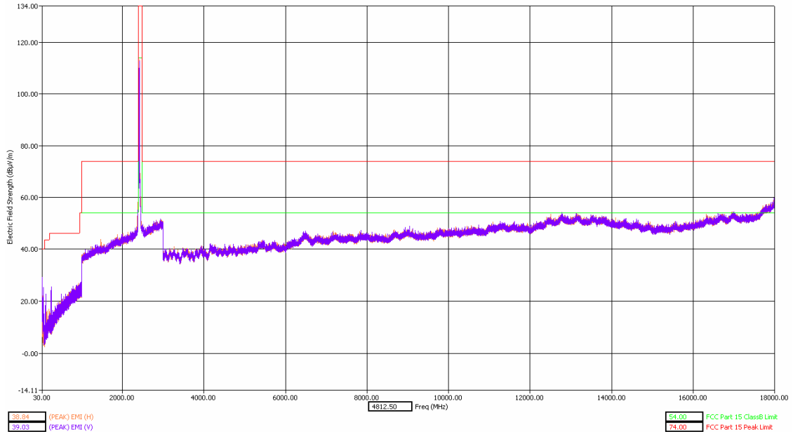
30 - 18000MHz Low Channel Dual Polarization X
