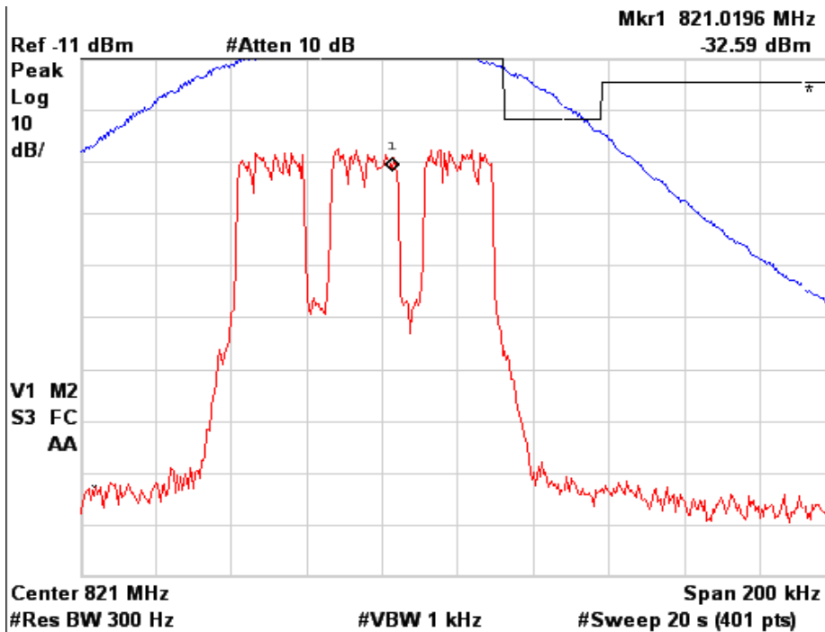
Figure 6a.2.5-4. WiDEN75 800 MHz Band, Quad-16QAM, Minimum Power, EA Emission Mask
