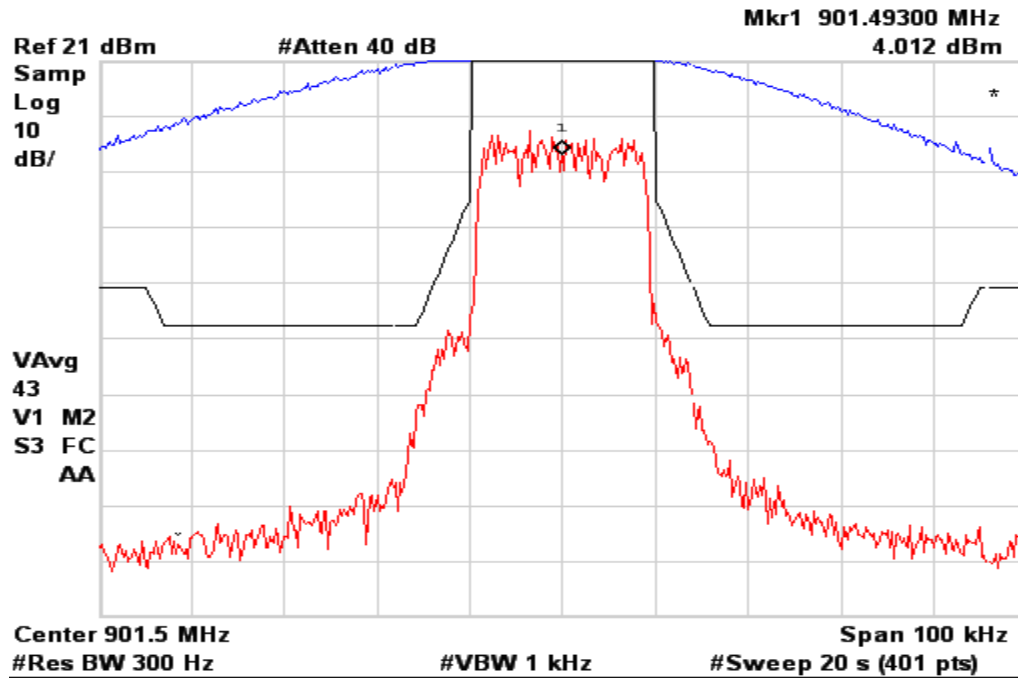
Figure 6b.2.1-3. iDEN NBPCS Band, Occupied Bandwidth, Quad-64QAM, Maximum Power.
