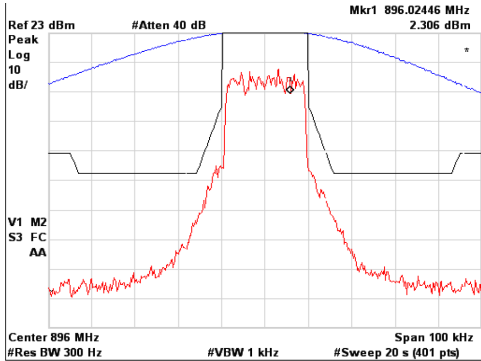
Figure 6a.2.8-5. WiDEN25 900 MHz Band, Quad-16QAM, Maximum Power, Emission Mask G
