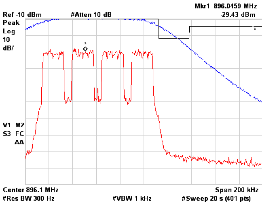
Figure 6a.2.11-6. WiDEN100 900 MHz Band, Quad-64QAM, Minimum Power, EA Emission Mask
