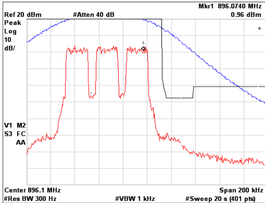
Figure 6a.2.10-3. WiDEN75 900 MHz Band, Quad-16QAM, Maximum Power, EA Emission Mask
