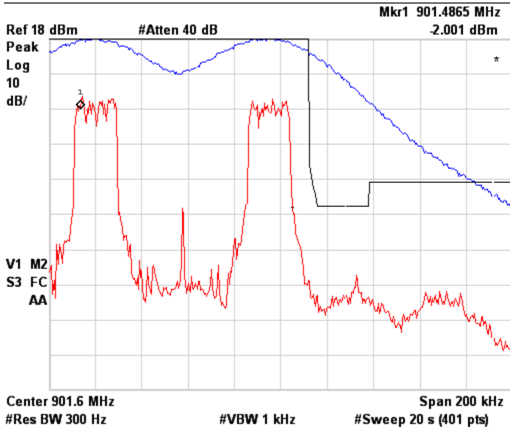
Figure 6b.2.6-2. WiDEN 50_Split NBPCS Band Occupied Bandwidth, Quad-16QAM.
