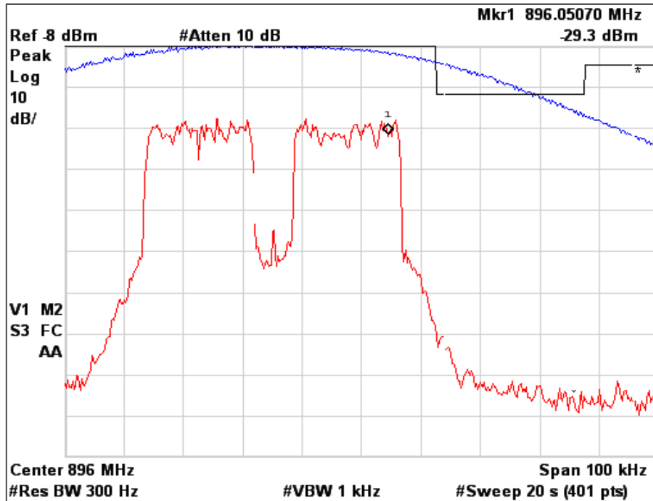
Figure 6a.2.9-4. WiDEN50 900 MHz Band, Continuous Quad-16QAM, Minimum Power, EA Emission Mask
