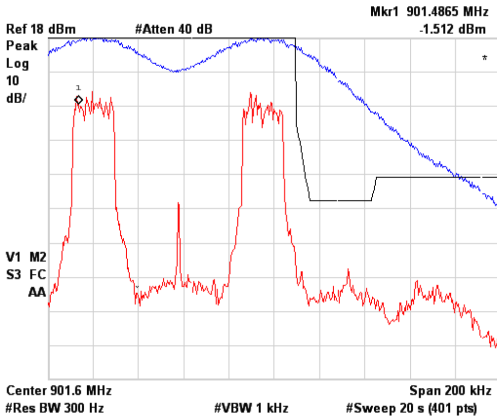
Figure 6b.2.6-3. WiDEN 50_Split NBPCS Band Occupied Bandwidth, Quad-64QAM
