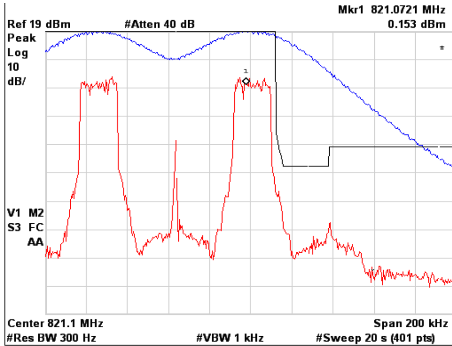
Figure 6a.2.7-3. WiDEN50 Split 800 MHz Band, Quad-16QAM, Maximum Power, EA Emission Mask
