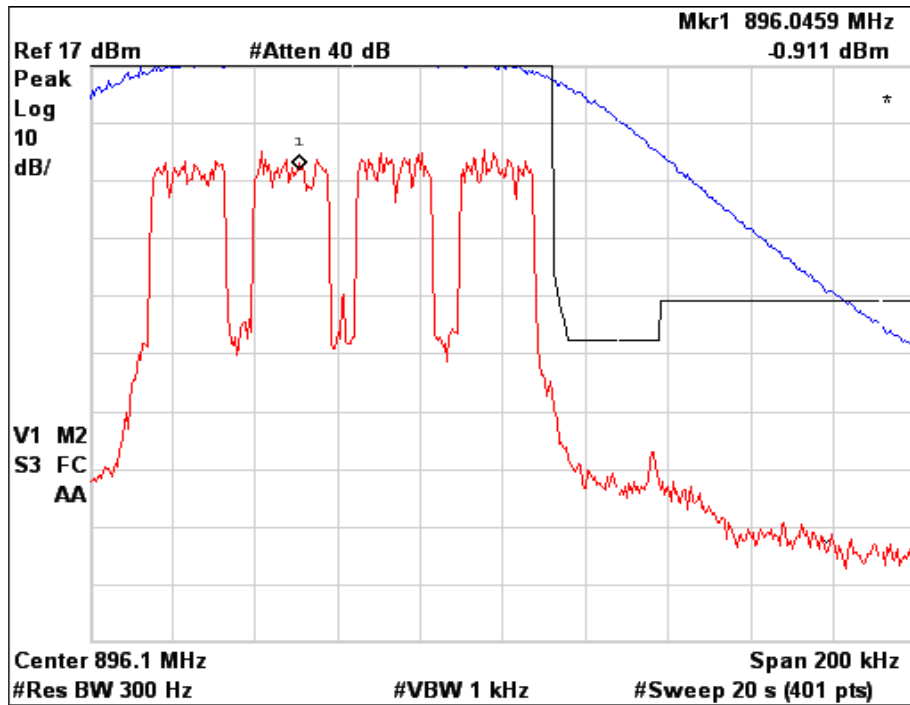
Figure 6a.2.11-5. WiDEN100 900 MHz Band, Quad-64QAM, Maximum Power, EA Emission Mask
