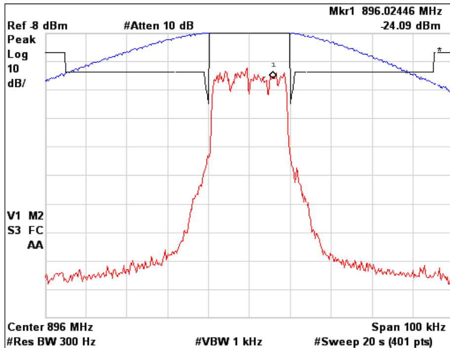
Figure 6a.2.8-10. WiDEN25 900 MHz Band, Quad-64QAM, Minimum Power, Emission Mask G
