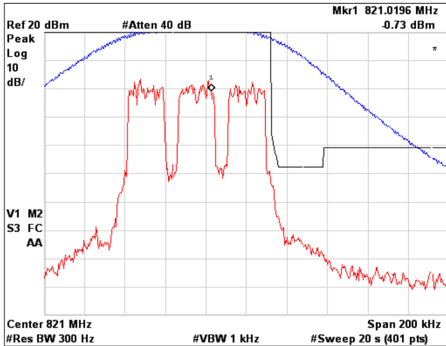
Figure 6a.2.5-5. WiDEN75 800 MHz Band, Quad-64QAM, Maximum Power, EA Emission Mask
