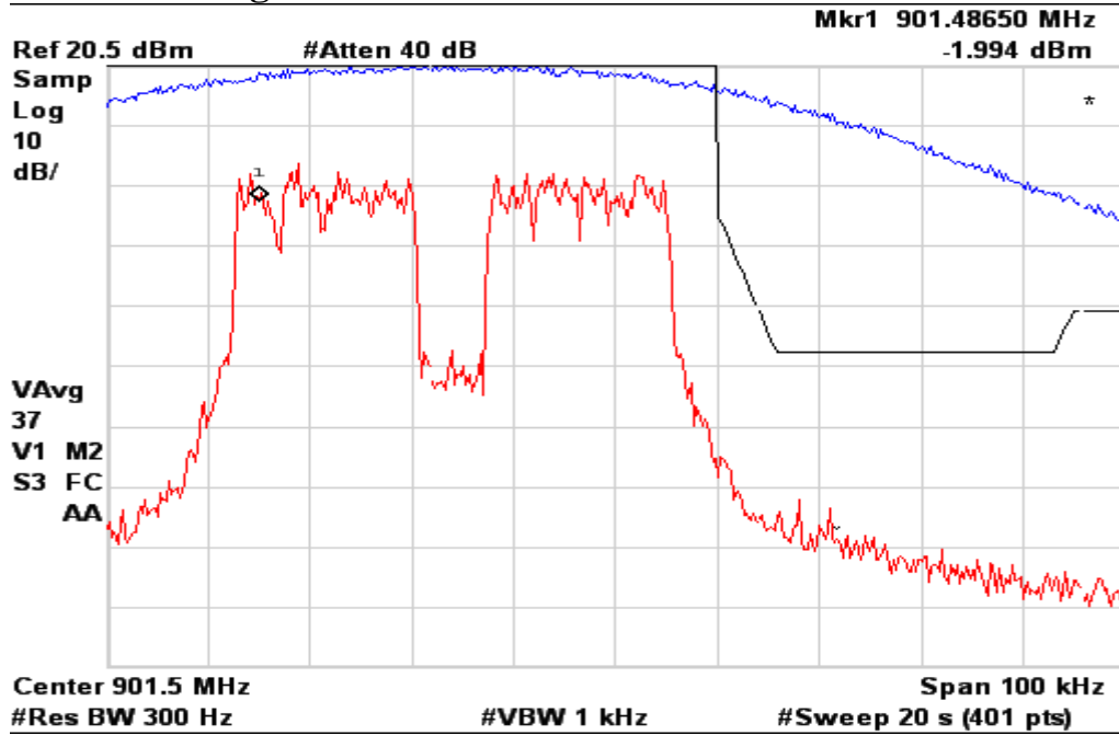
Figure 6b.2.3-1. WiDEN 50 NBPCS Band Occupied Bandwidth, Quad-QPSK.
