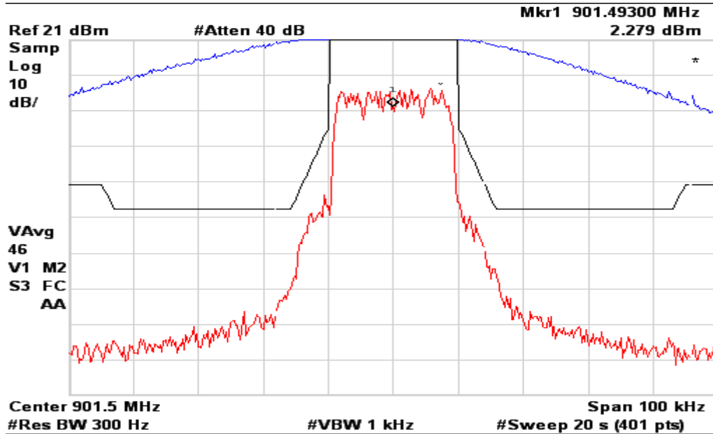
Figure 6b.2.1-1 iDEN NBPCS Band, Occupied Bandwidth, Quad-QPSK.
