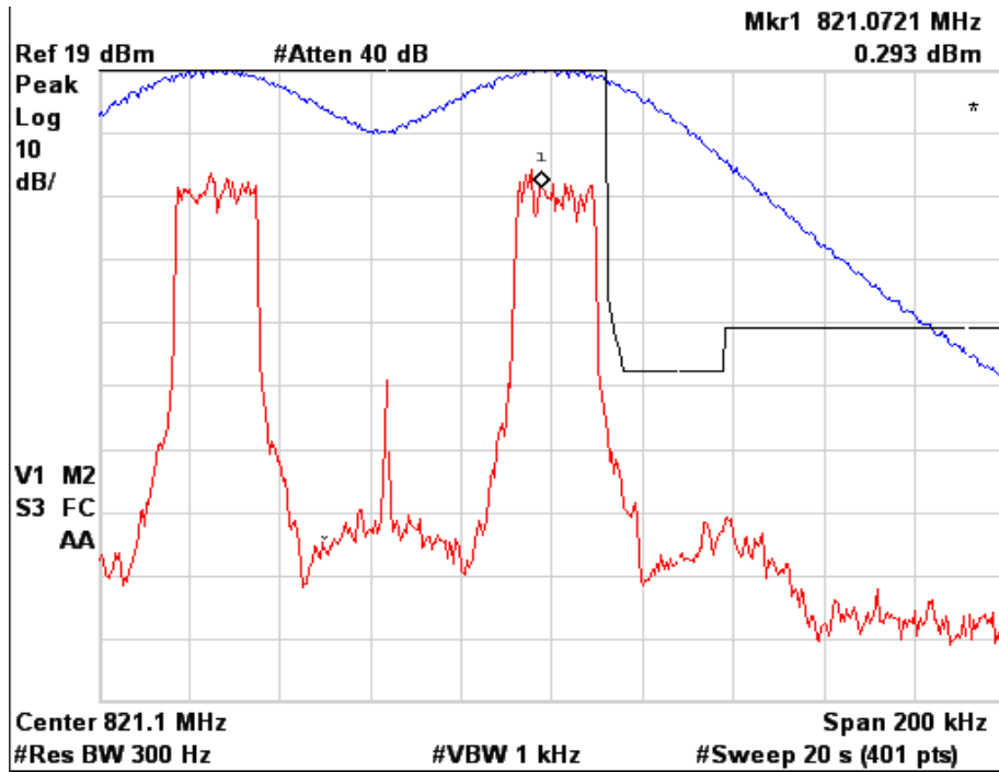
Figure 6a.2.7-5. WiDEN50 Split 800 MHz Band, Quad-64QAM, Maximum Power, EA Emission Mask
