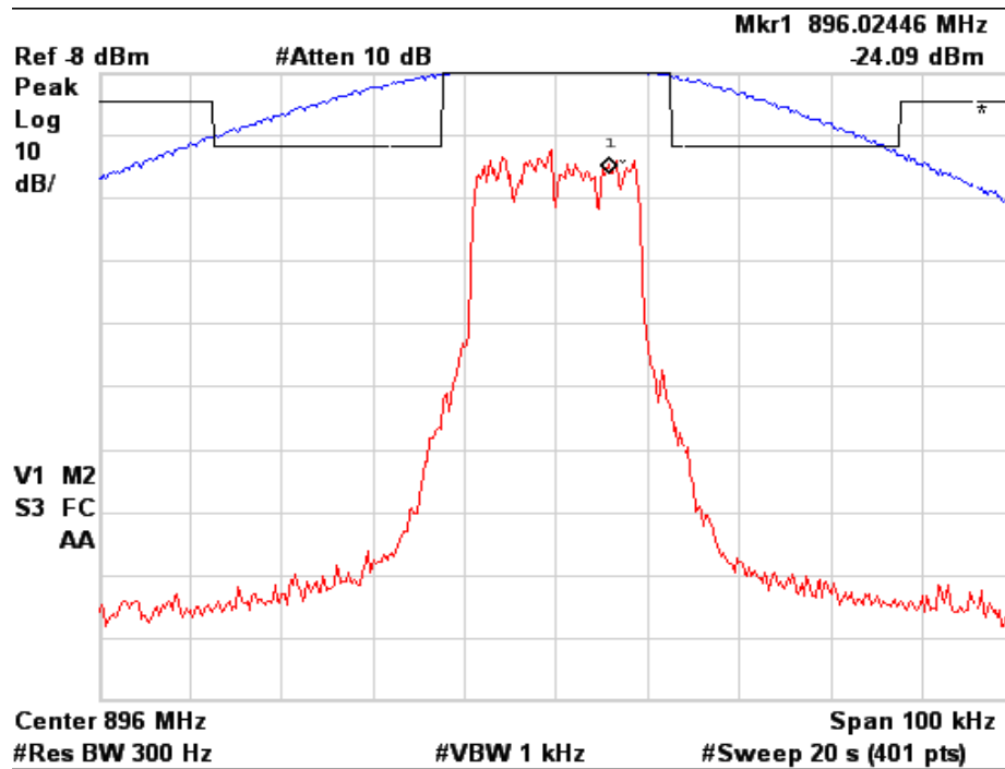
Figure 6a.2.8-12. WiDEN25 900 MHz Band, Quad-64QAM, Minimum Power, EA Emission Mask
