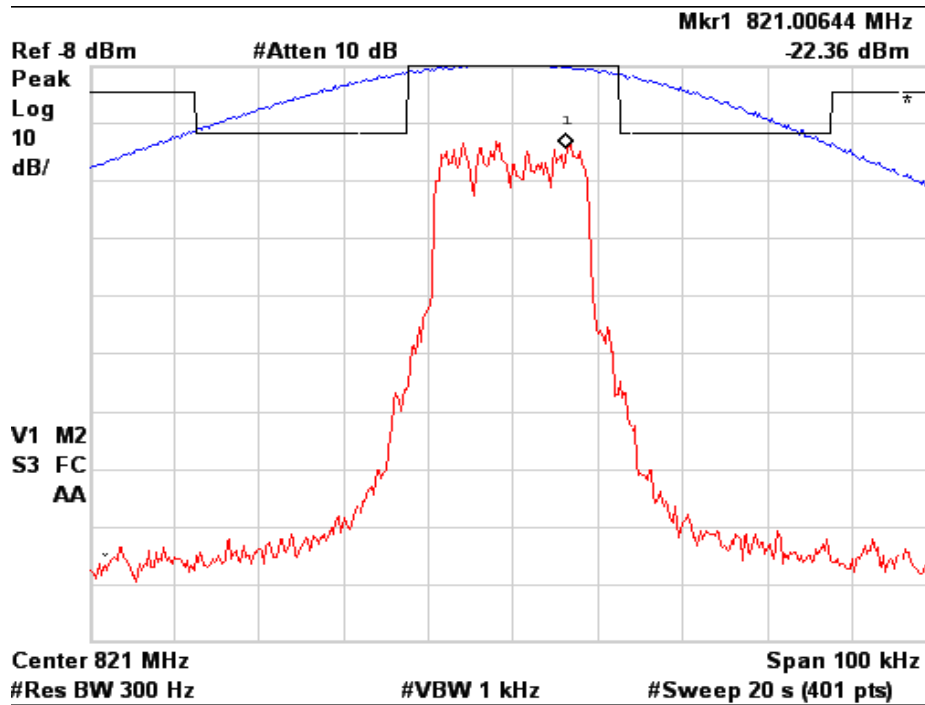
Figure 6a.2.3-8. WiDEN25 800 MHz Band, Quad-16QAM, Minimum Power, EA Emission Mask
