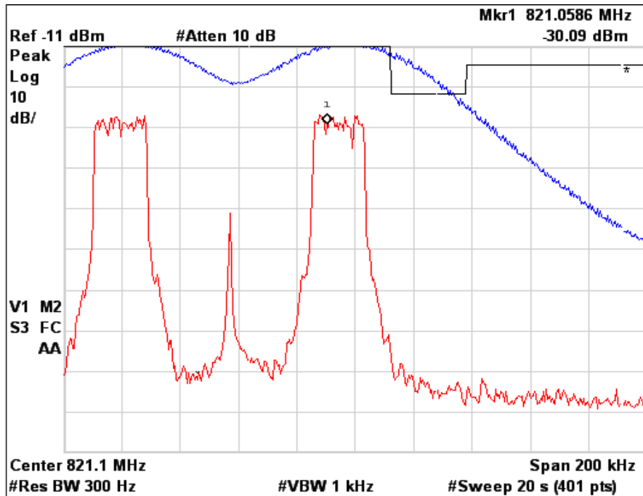
Figure 6a.2.7-6. WiDEN50 Split 800 MHz Band, Quad-64QAM, Minimum Power, EA Emission Mask
