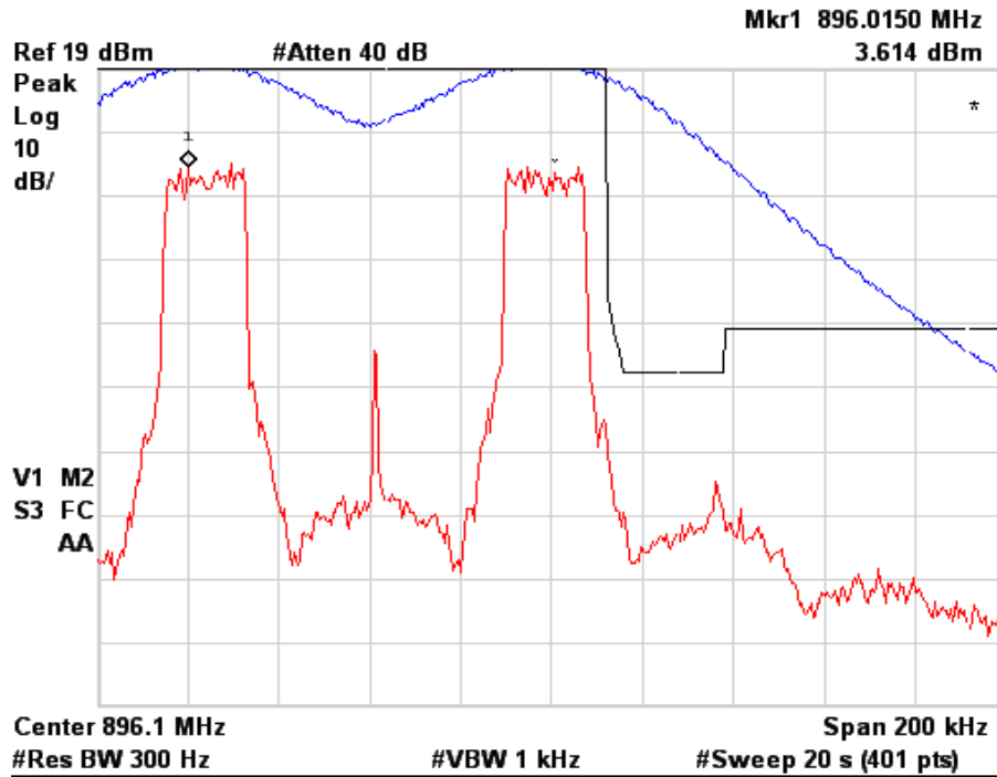
Figure 6a.2.12-3. WiDEN50 Split 900 MHz Band, Quad-16QAM, Maximum Power, EA Emission Mask
