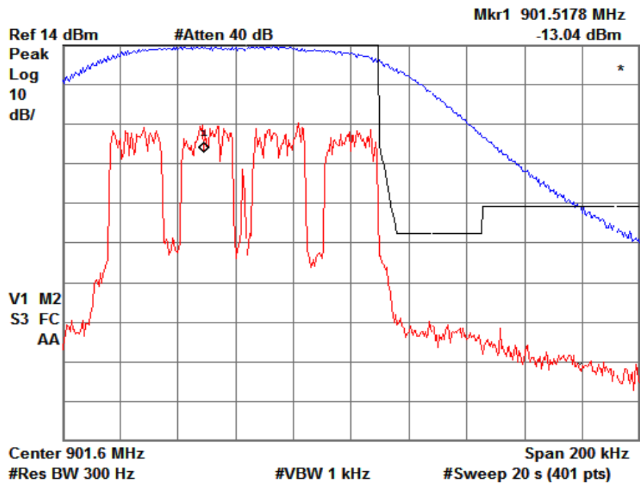
Figure 6b.2.5-3. WiDEN 100 NBPCS Band Occupied Bandwidth, Quad-64QAM.
