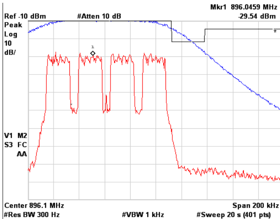
Figure 6a.2.11-2. WiDEN100 900 MHz Band, Quad-QPSK, Minimum Power, EA Emission Mask
