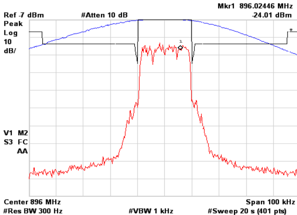
Figure 6a.2.2-10. iDEN 900 MHz Band, Quad-64QAM, Minimum Power, Emission Mask G
