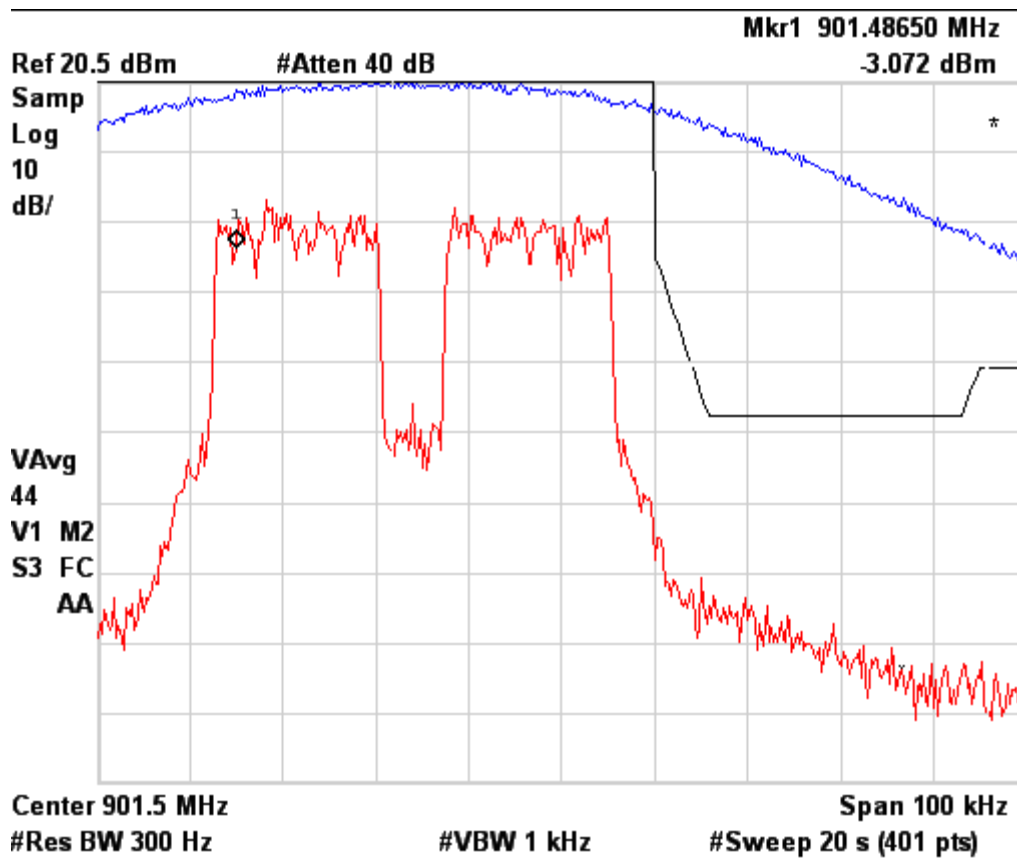
Figure 6b.2.3-3. WiDEN 50 NBPCS Band Occupied Bandwidth, Quad-64QAM.
