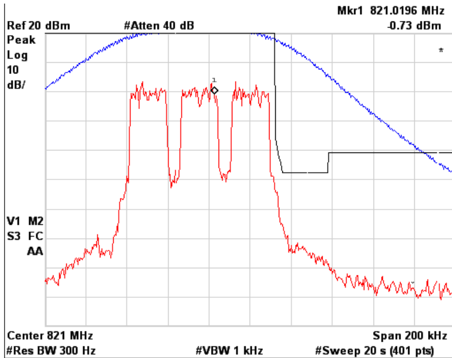
Figure 6a.2.5-1. WiDEN75 800 MHz Band, Quad-QPSK, Maximum Power, EA Emission Mask
