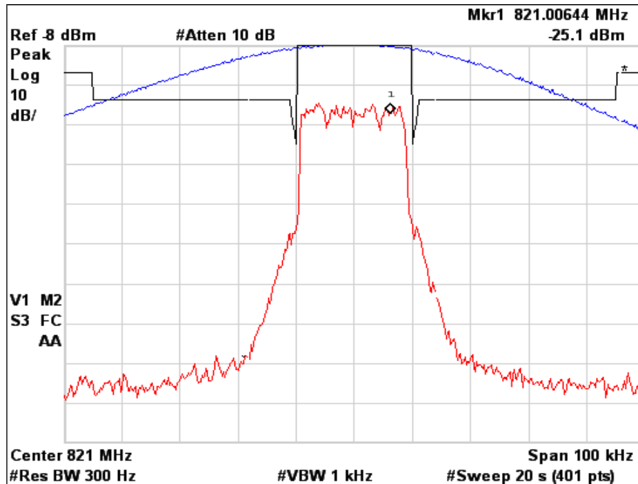
Figure 6a.2.3-10. WiDEN25 800 MHz Band, Quad-64QAM, Minimum Power, Emission Mask G
