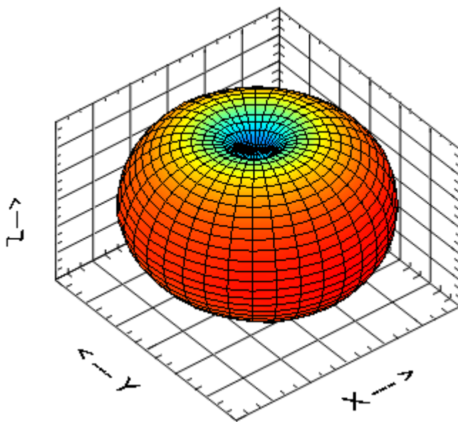
Figure 6a.6-3 Antenna pattern in the 900 MHz NBPCS frequency band.
