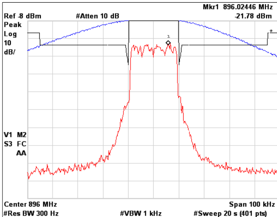
Figure 6a.2.8-2. WiDEN25 900 MHz Band, Quad-QPSK, Minimum Power, Emission Mask G
