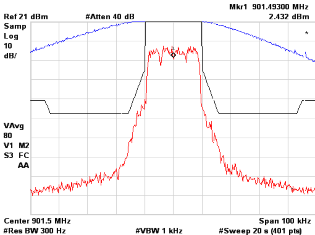
Figure 6b.2.1-2. iDEN NBPCS Band, Occupied Bandwidth, Quad-16QAM.
