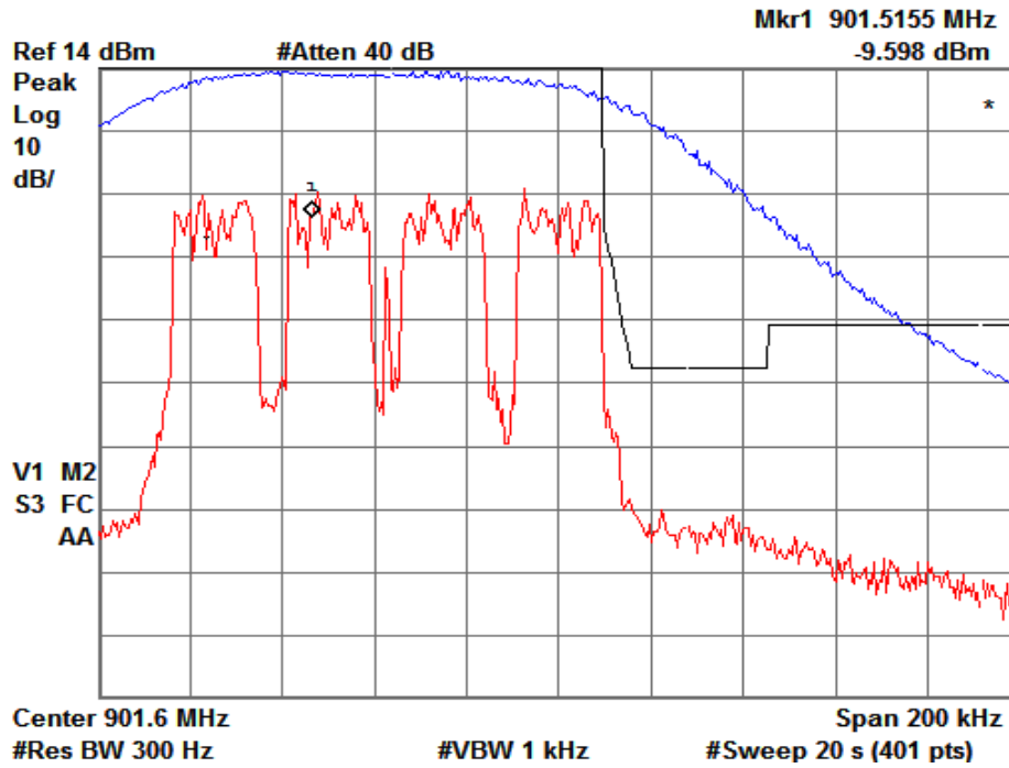
Figure 6b.2.5-1. WiDEN 100 NBPCS Band Occupied Bandwidth, Quad-QPSK.
