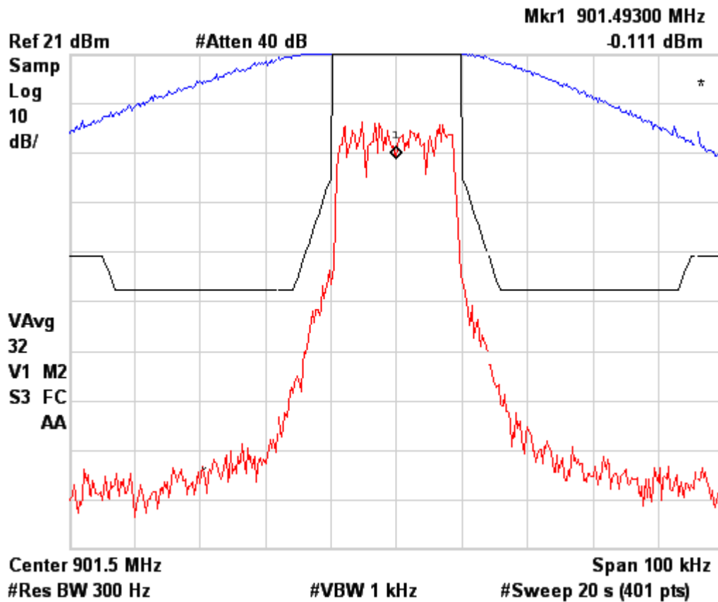
Figure 6b.2.2-3. WiDEN 25 NBPCS Band, Occupied Bandwidth, Quad-64QAM.
