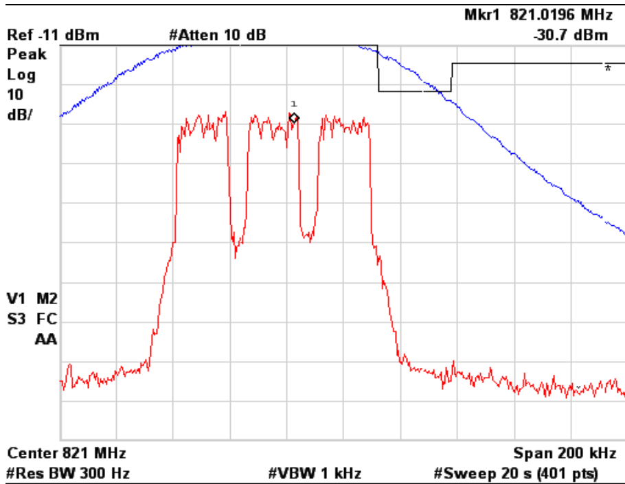
Figure 6a.2.5-6. WiDEN75 800 MHz Band, Quad-64QAM, Minimum Power, EA Emission Mask
