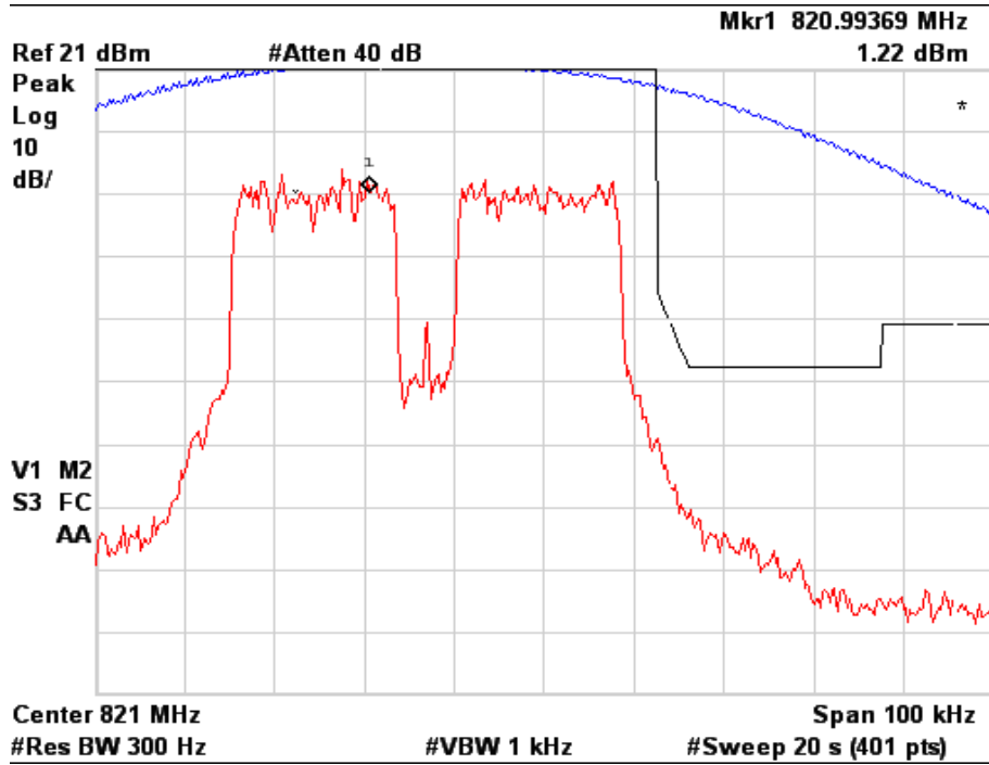
Figure 6a.2.4-3. WiDEN50 800 MHz Band, Continuous Quad-16QAM, Maximum Power, EA Emission Mask
