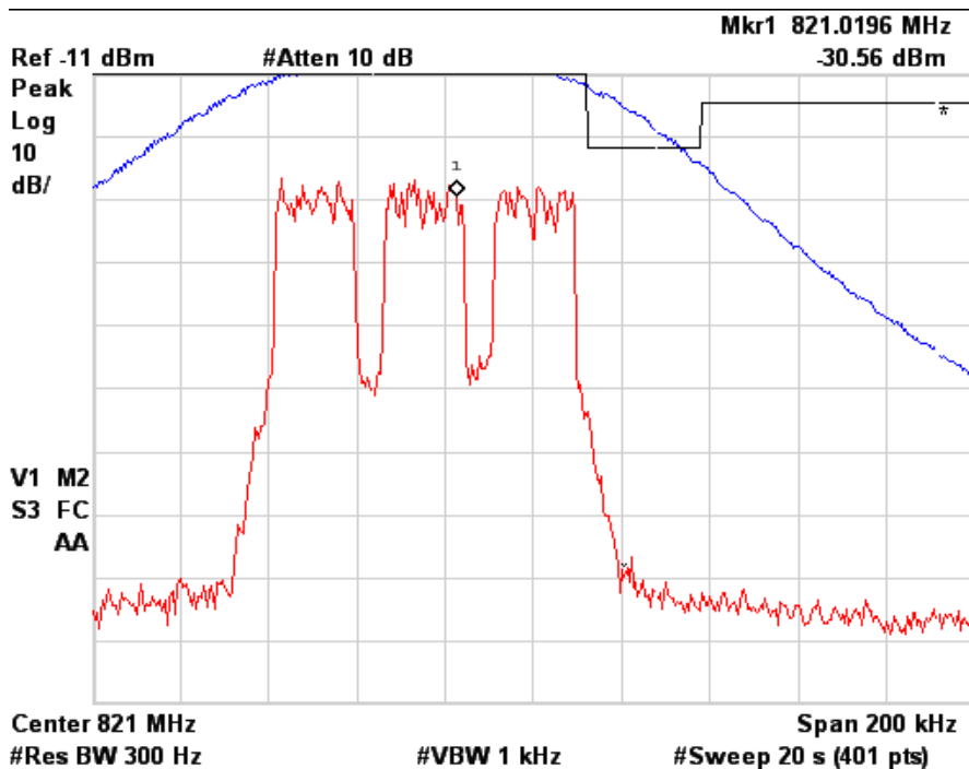
Figure 6a.2.5-2. WiDEN75 800 MHz Band, Quad-QPSK, Minimum Power, EA Emission Mask
