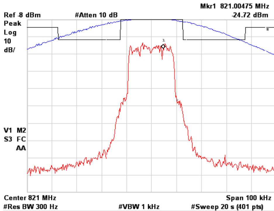
Figure 6a.2.1-4. iDEN 800 MHz Band, Quad-QPSK, Minimum Power, EA Emission Mask
