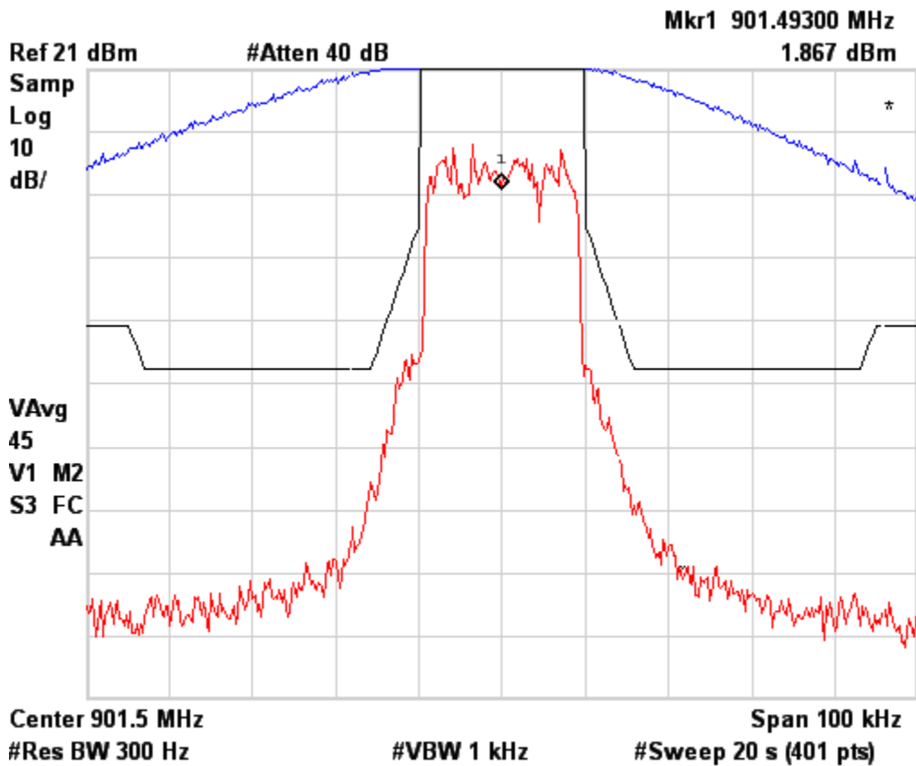
Figure 6b.2.2-2. WiDEN 25 NBPCS Band, Occupied Bandwidth, Quad-16QAM.
