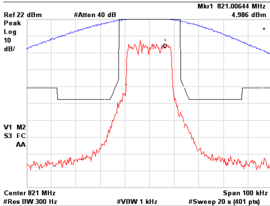
Figure 6a.2.3-7. WiDEN25 800 MHz Band, Quad-16QAM, Maximum Power, EA Emission Mask
