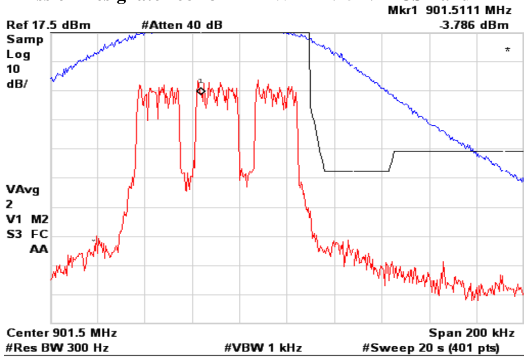
Figure 6b.2.4-1. WiDEN 75 NBPCS Band Occupied Bandwidth, Quad-QPSK.
