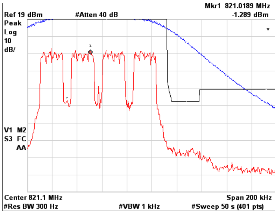
Figure 6a.2.6-5. WiDEN100 800 MHz Band, Quad-64QAM, Maximum Power, EA Emission Mask
