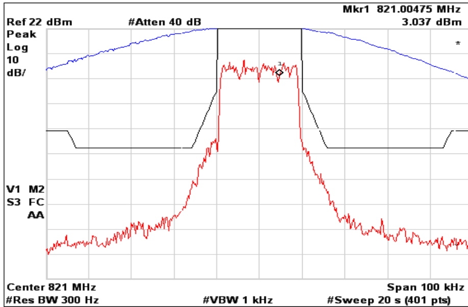
Figure 6a.2.1-1. iDEN 800 MHz Band, Quad-QPSK, Maximum Power, Emission Mask G
