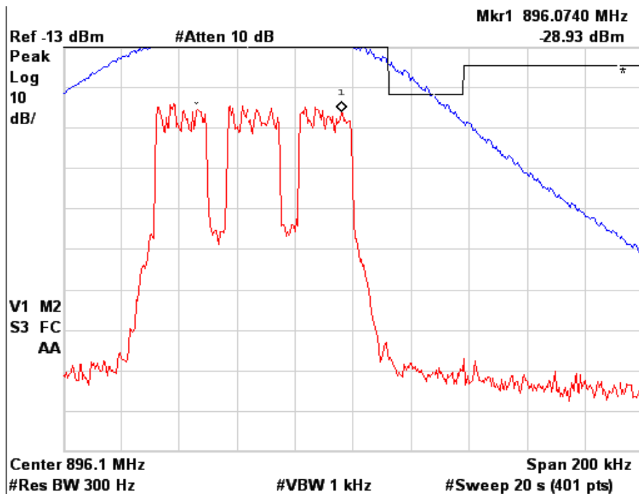
Figure 6a.2.10-2. WiDEN75 900 MHz Band, Quad-QPSK, Minimum Power, EA Emission Mask
