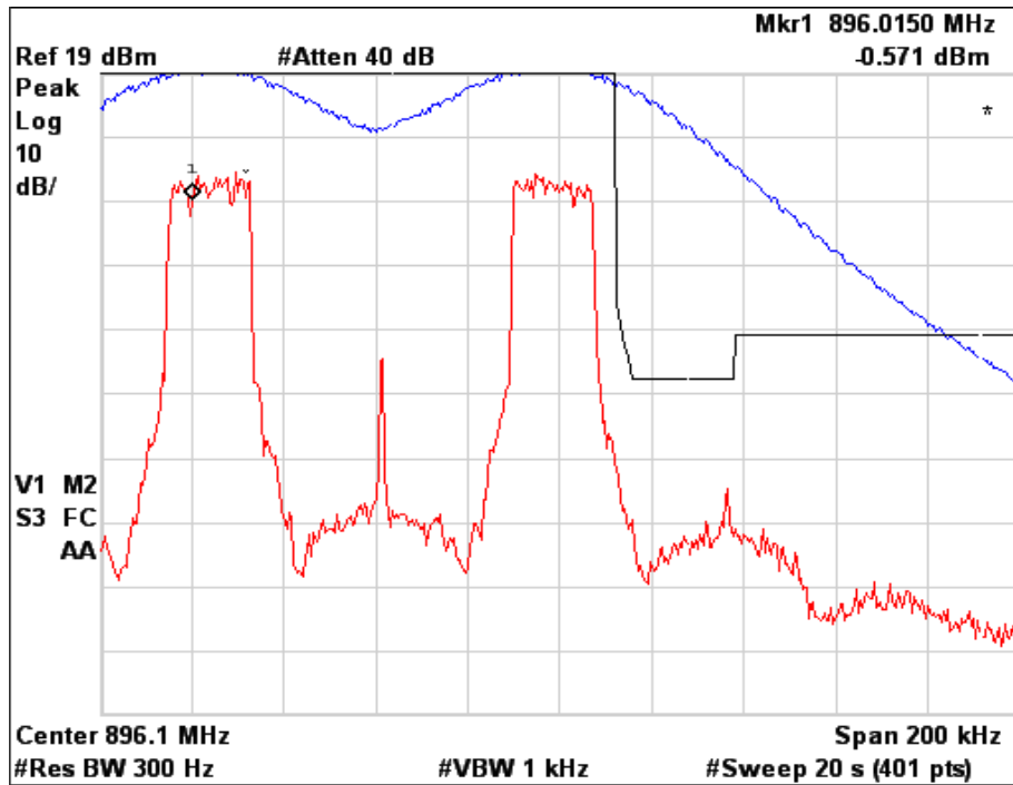
Figure 6a.2.12-5. WiDEN50 Split 900 MHz Band, Quad-64QAM, Maximum Power, EA Emission Mask
