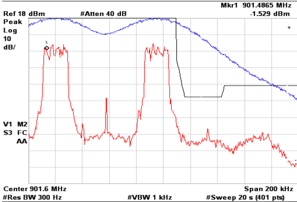
Figure 6b.2.6-1. WiDEN 50_Split NBPCS Band Occupied Bandwidth, Quad-QPSK.
