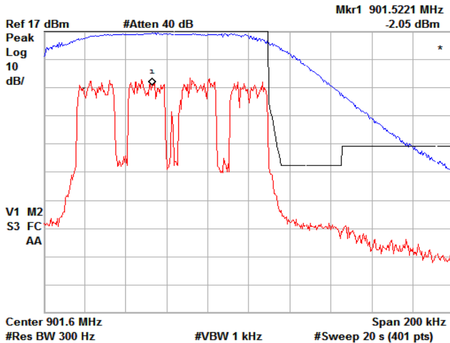
Figure 6b.2.5-2. WiDEN 100 NBPCS Band Occupied Bandwidth, Quad-16QAM.
