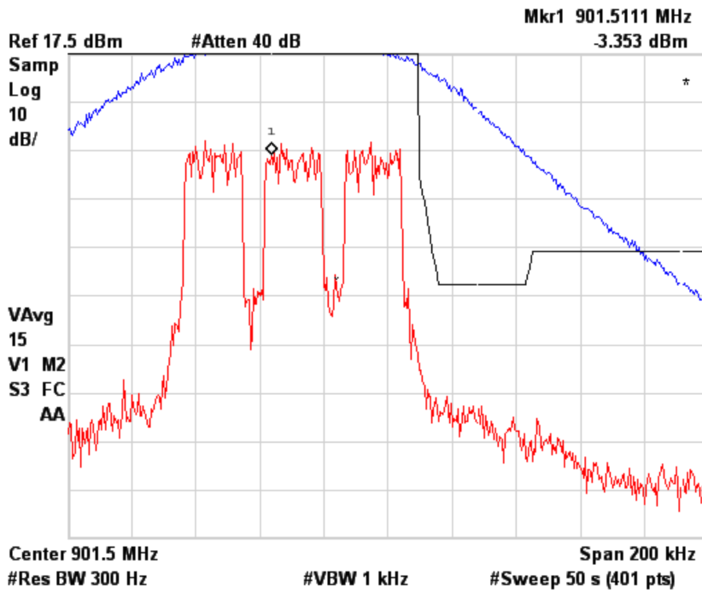
Figure 6b.2.4-3. WiDEN 75 NBPCS Band Occupied Bandwidth, Quad-64QAM.
