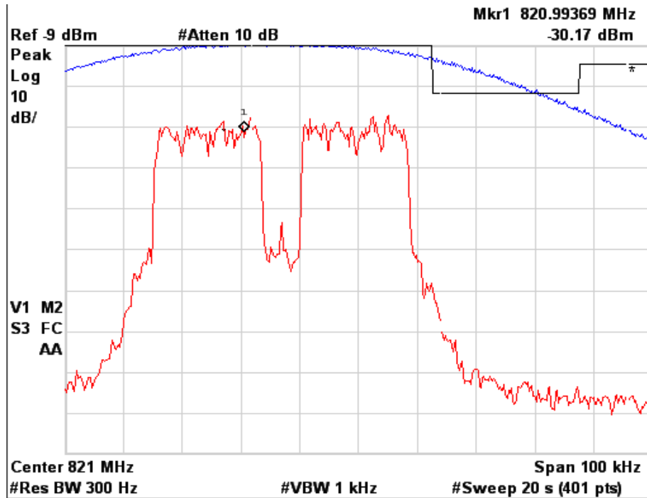
Figure 6a.2.4-4. WiDEN50 800 MHz Band, Continuous Quad-16QAM, Minimum Power, EA Emission Mask
