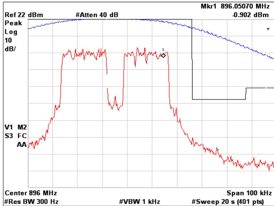
Figure 6a.2.9-5. WiDEN50 900 MHz Band, Continuous Quad-64QAM, Maximum Power, EA Emission Mask
