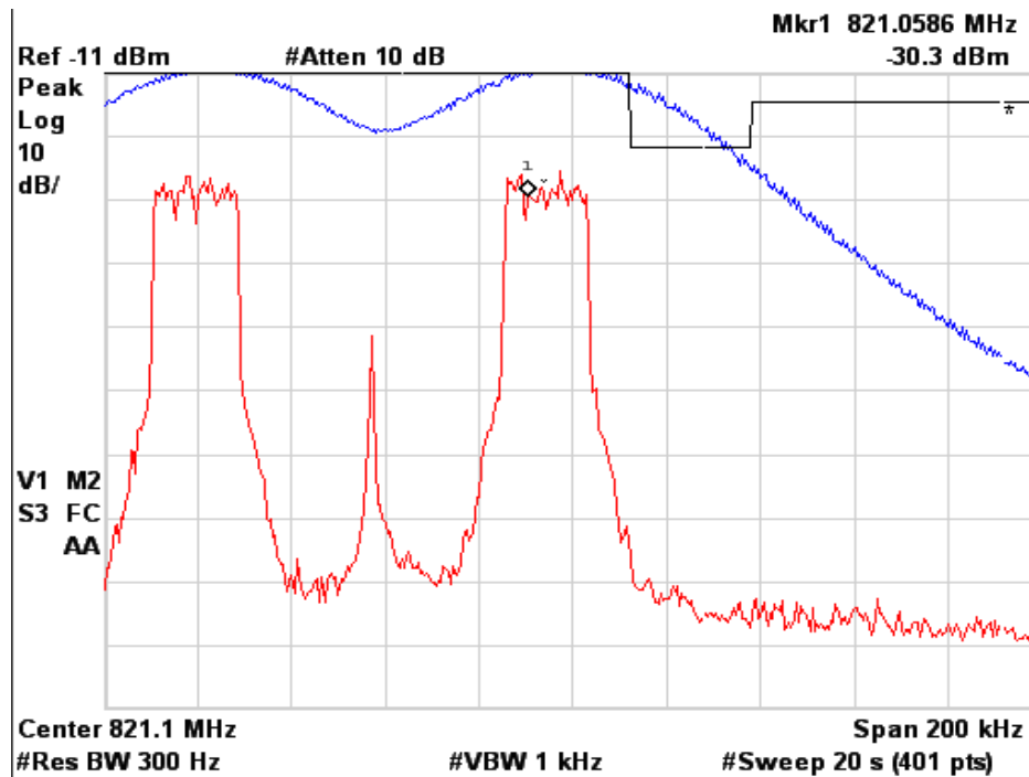
Figure 6a.2.7-4. WiDEN50 Split 800 MHz Band, Quad-16QAM, Minimum Power, EA Emission Mask
