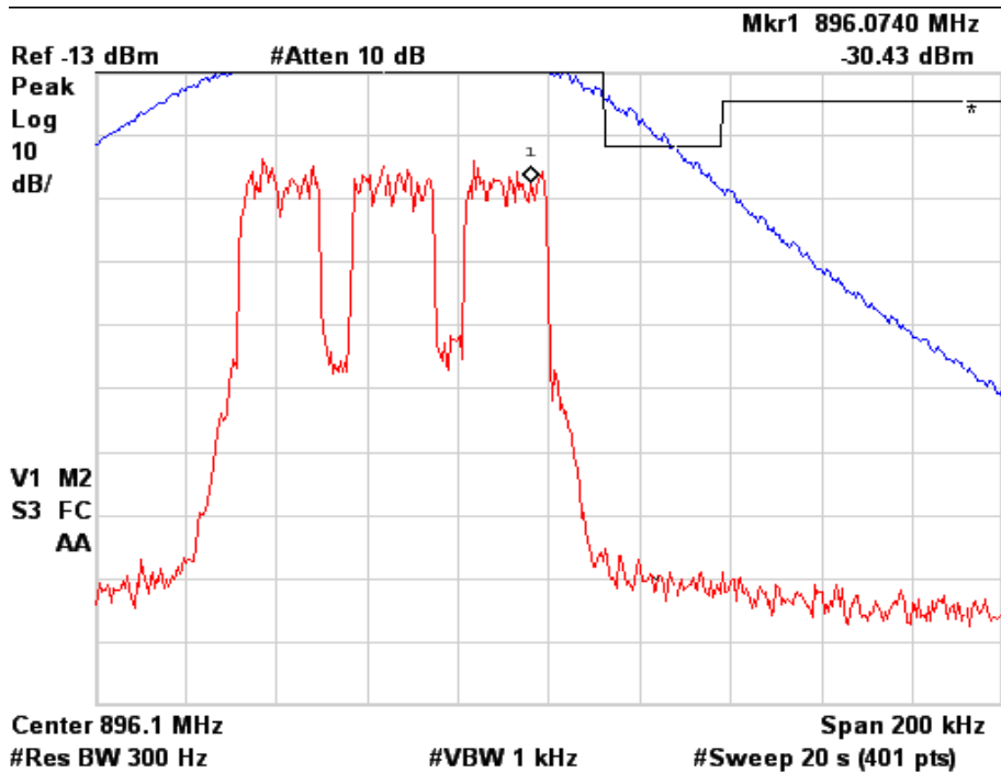
Figure 6a.2.10-6. WiDEN75 900 MHz Band, Quad-64QAM, Minimum Power, EA Emission Mask
