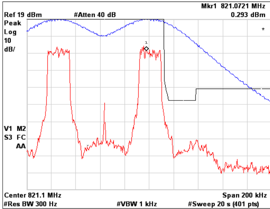
Figure 6a.2.7-1. WiDEN50 Split 800 MHz Band, Quad-QPSK, Maximum Power, EA Emission Mask
