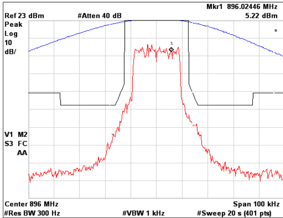
Figure 6a.2.8-11. WiDEN25 900 MHz Band, Quad-64QAM, Maximum Power, EA Emission Mask
