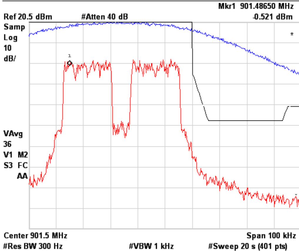
Figure 6b.2.3-2. WiDEN 50 NBPCS Band Occupied Bandwidth, Quad-16QAM.
