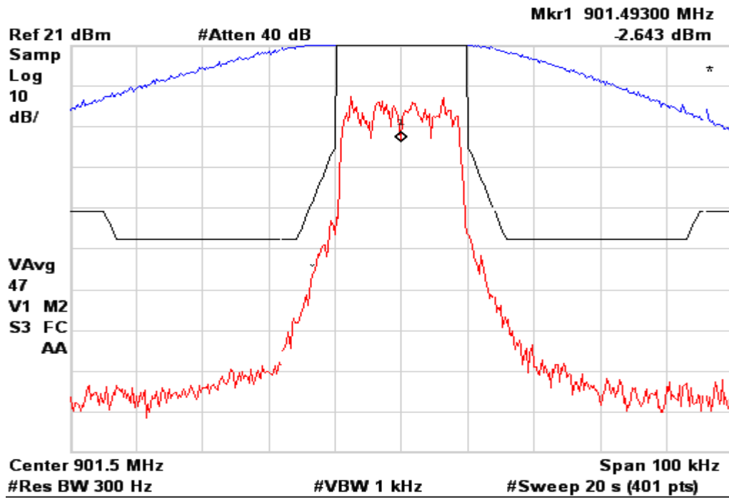
Figure 6b.2.2-1. WiDEN 25 NBPCS Band, Occupied Bandwidth, Quad-QPSK.
