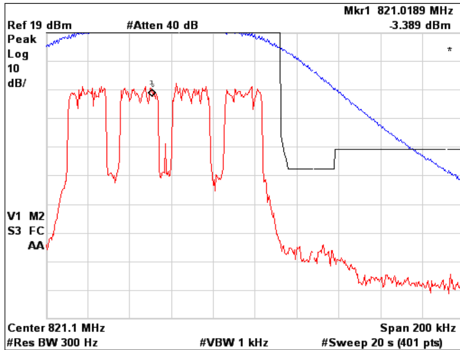
Figure 6a.2.6-3. WiDEN100 800 MHz Band, Quad-16QAM, Maximum Power, EA Emission Mask
