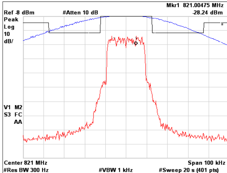
Figure 6a.2.1-12. iDEN 800 MHz Band, Quad-64QAM, Minimum Power, EA Emission Mask
