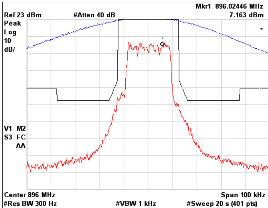
Figure 6a.2.2-7. iDEN 900 MHz Band, Quad-16QAM, Maximum Power, EA Emission Mask
