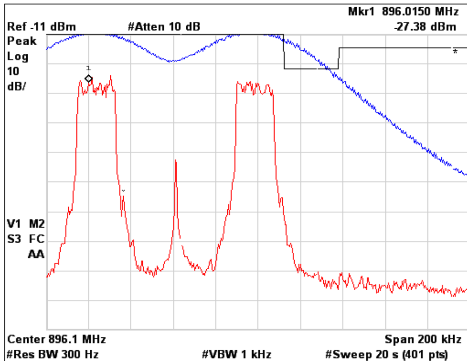
Figure 6a.2.12-2. WiDEN50 Split 900 MHz Band, Quad-QPSK, Minimum Power, EA Emission Mask
