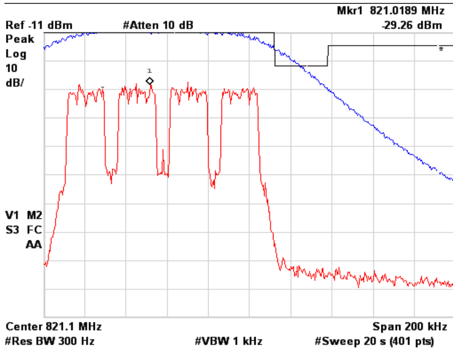
Figure 6a.2.6-6. WiDEN100 800 MHz Band, Quad-64QAM, Minimum Power, EA Emission Mask
