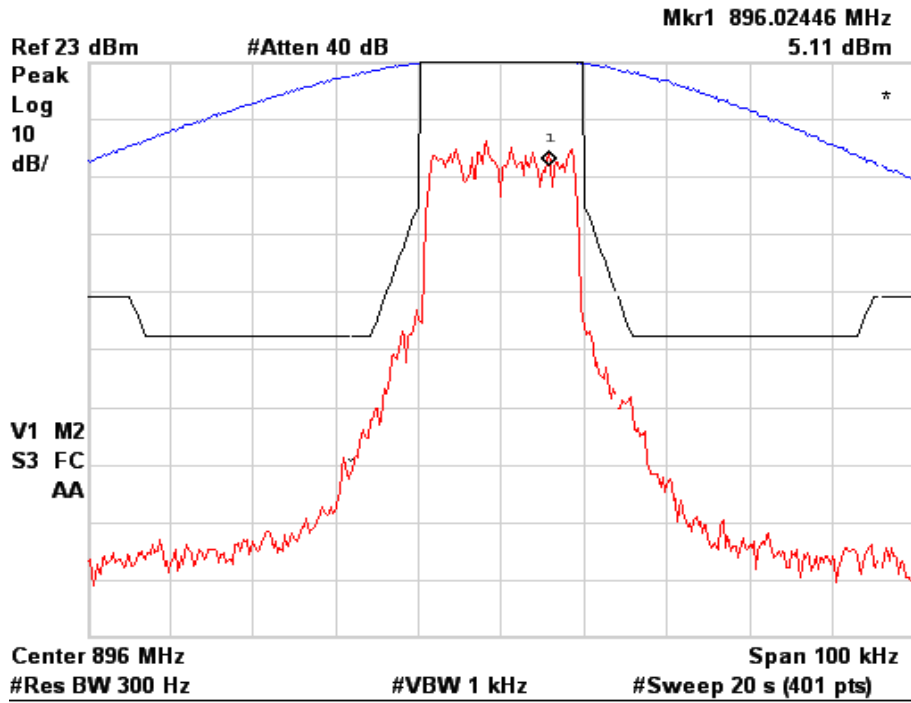
Figure 6a.2.8-9. WiDEN25 900 MHz Band, Quad-64QAM, Maximum Power, Emission Mask G
