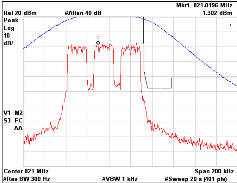
Figure 6a.2.5-3. WiDEN75 800 MHz Band, Quad-16QAM, Maximum Power, EA Emission Mask
