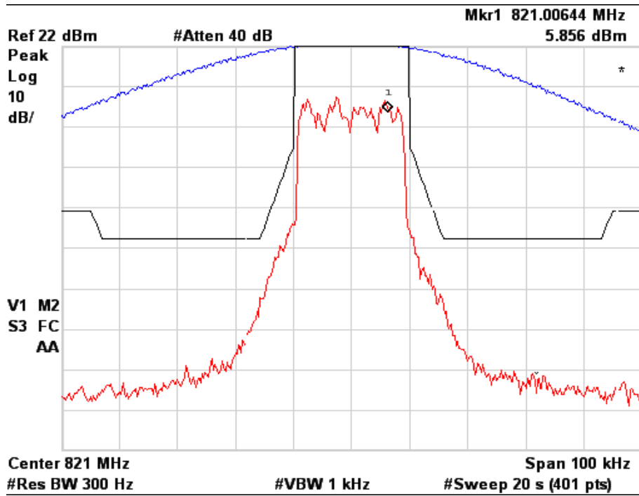
Figure 6a.2.3-1. WiDEN25 800 MHz Band, Quad-QPSK, Maximum Power, Emission Mask G
