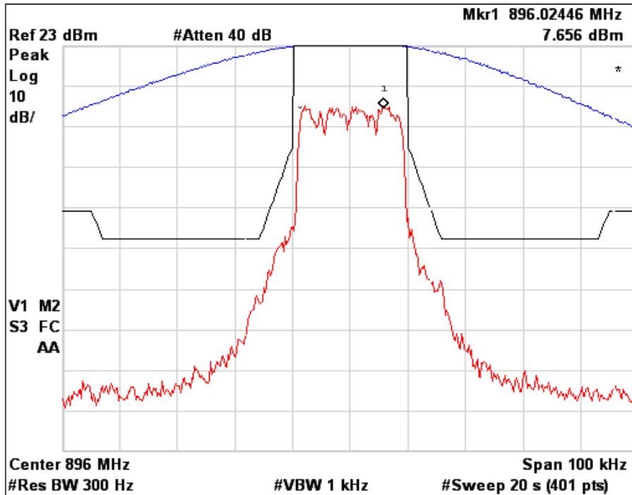
Figure 6a.2.8-1. WiDEN25 900 MHz Band, Quad-QPSK, Maximum Power, Emission Mask G
