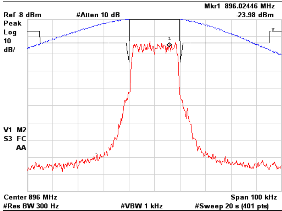
Figure 6a.2.8-6. WiDEN25 900 MHz Band, Quad-16QAM, Minimum Power, Emission Mask G
