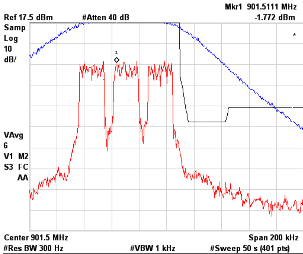
Figure 6b.2.4-2. WiDEN 75 NBPCS Band Occupied Bandwidth, Quad-16QAM.
