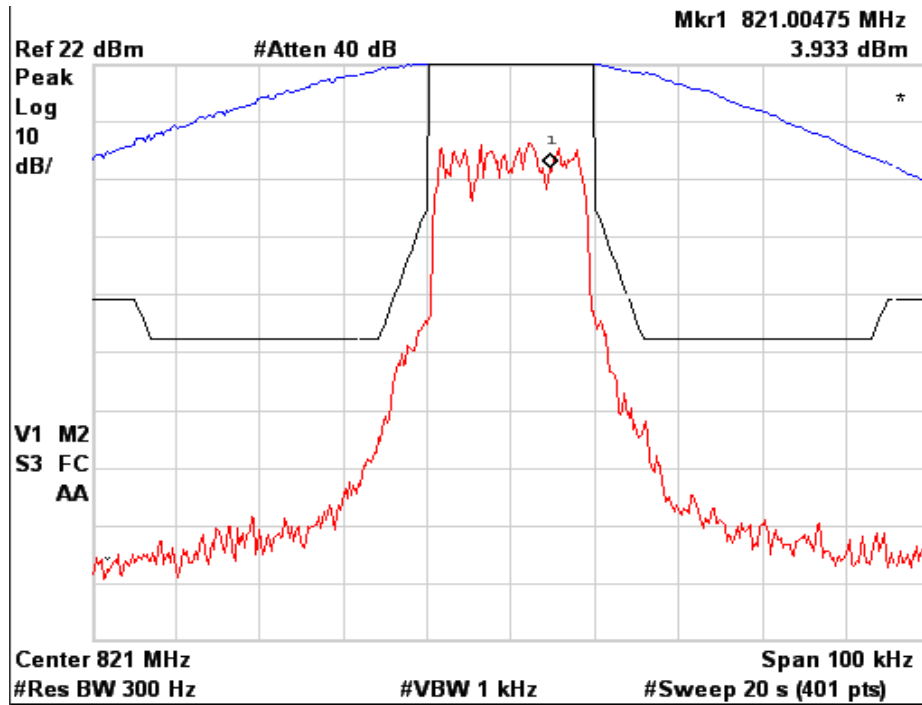
Figure 6a.2.1-9. iDEN 800 MHz Band, Quad-64QAM, Maximum Power, Emission Mask G
