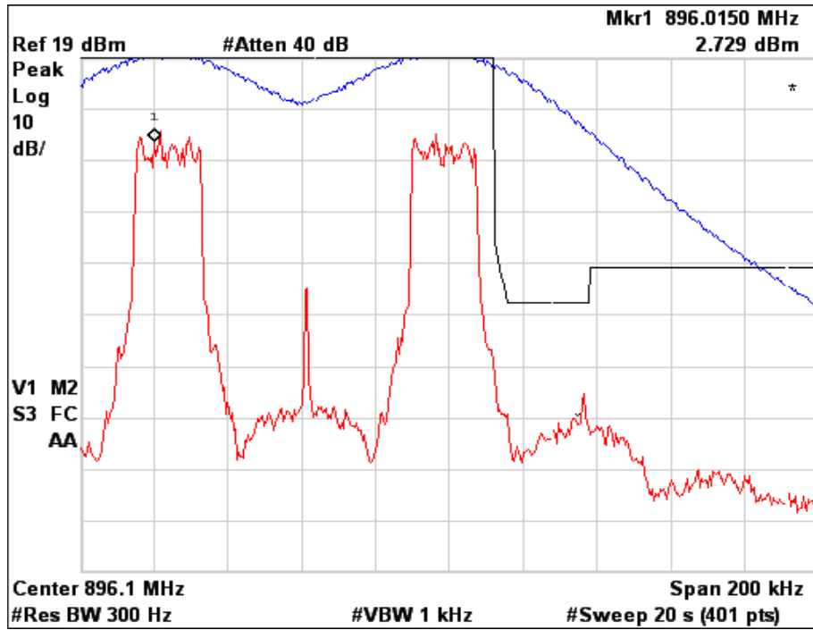
Figure 6a.2.12-1. WiDEN50 Split 900 MHz Band, Quad-QPSK, Maximum Power, EA Emission Mask
