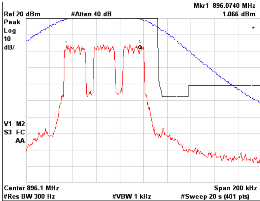
Figure 6a.2.10-5. WiDEN75 900 MHz Band, Quad-64QAM, Maximum Power, EA Emission Mask
