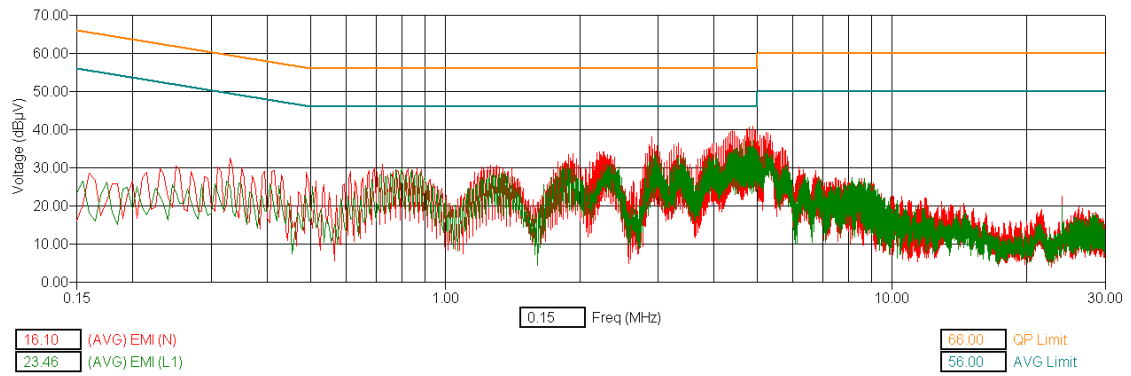
Bluetooth – Hopping - Tx Mode – Average Detector
