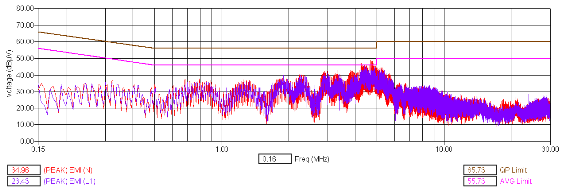
Bluetooth – Hopping - Tx Mode – Peak Detector
