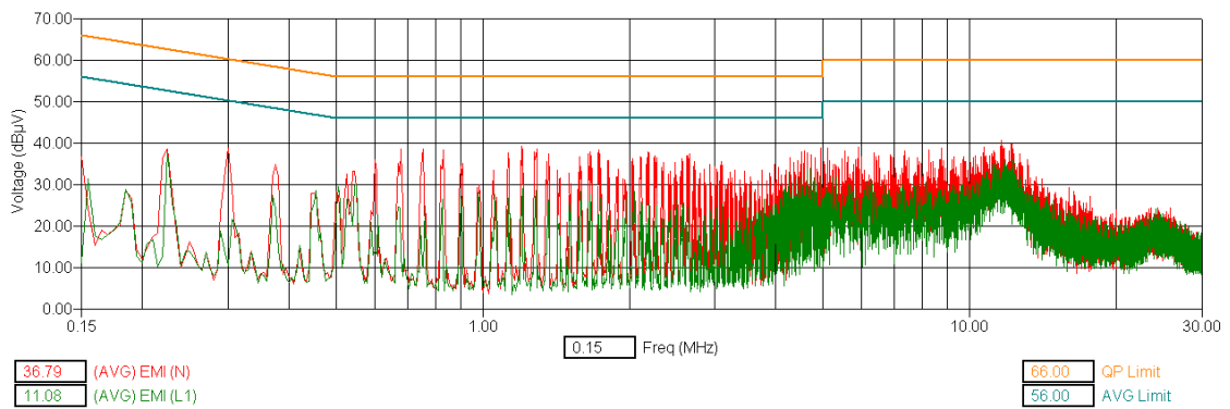
WLAN Channel 11 - Tx Mode - AVG Detector
