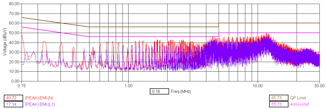
WLAN Channel 6 - Tx Mode - Peak Detector
