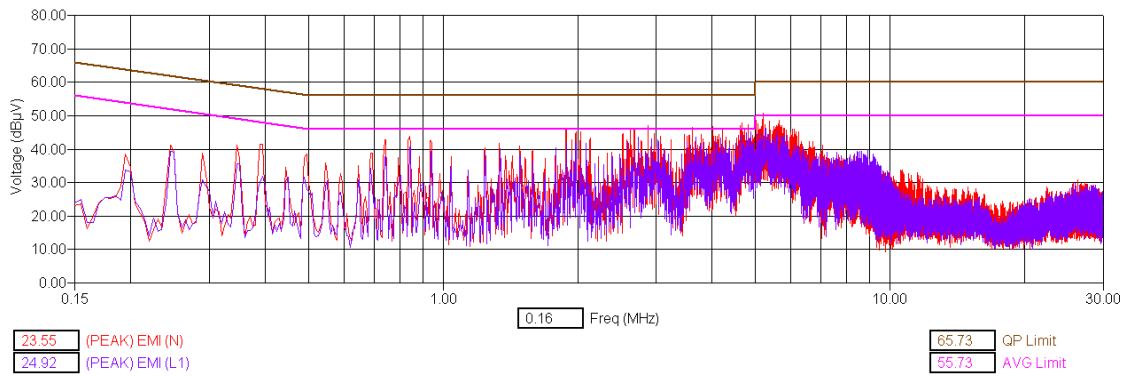
WLAN Channel 11 - Tx Mode - Peak Detector
