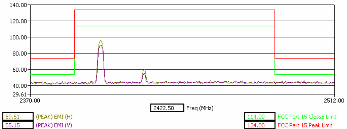
Authorized Band Emissions Low Channel Dual Polarization Y – slider closed
