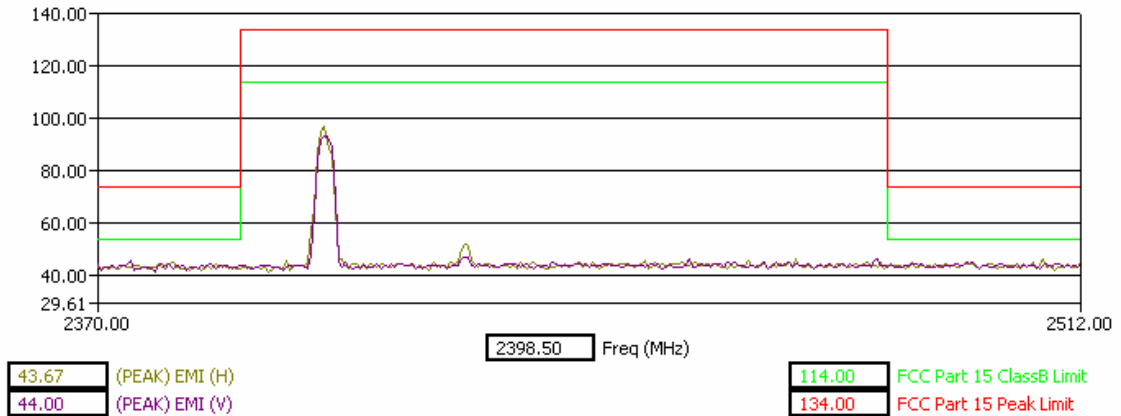
Authorized Band Emissions Low Channel Dual Polarization Z – slider closed
