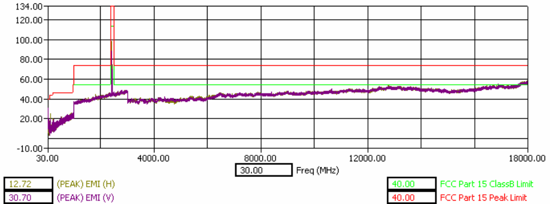
30 MHz – 18 GHz Low Channel Dual Polarization Z – slider open
