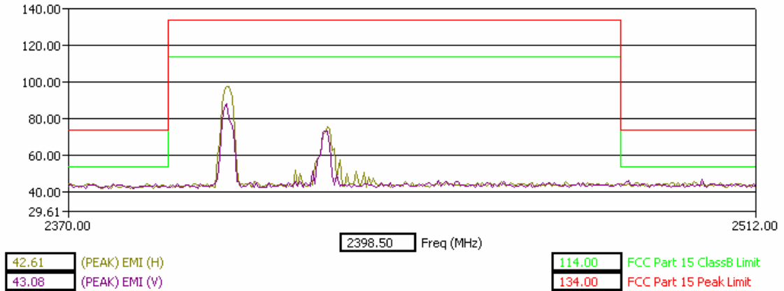
Authorized Band Emissions Low Channel Dual Polarization Z – slider open
