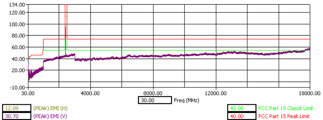
30 MHz – 18 GHz Low Channel Dual Polarization Z – slider closed
