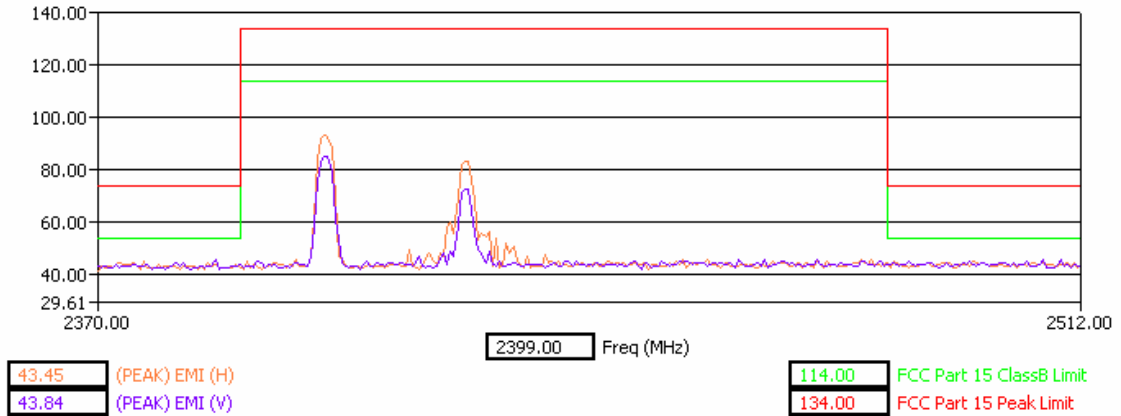
Authorized Band Emissions Low Channel Dual Polarization Y – slider open
