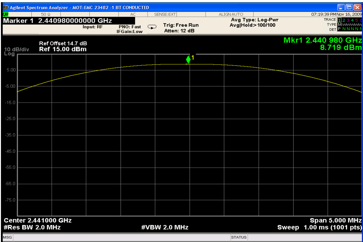
Peak Output Power – Mid Channel with EDR Disabled
