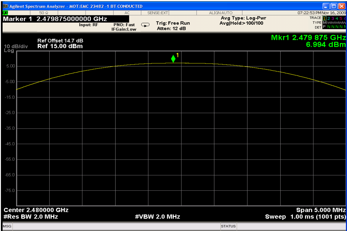
Peak Output Power – High Channel with EDR Disabled
