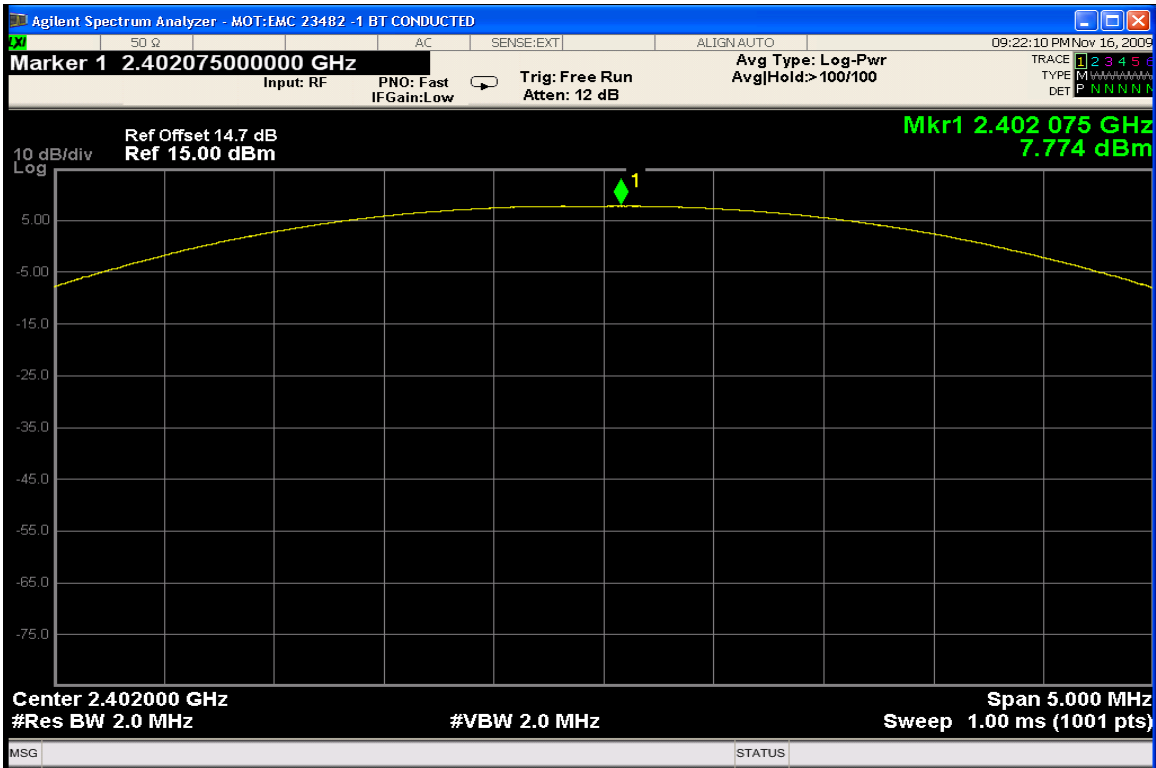
Peak Output Power – Low Channel with EDR Enabled
