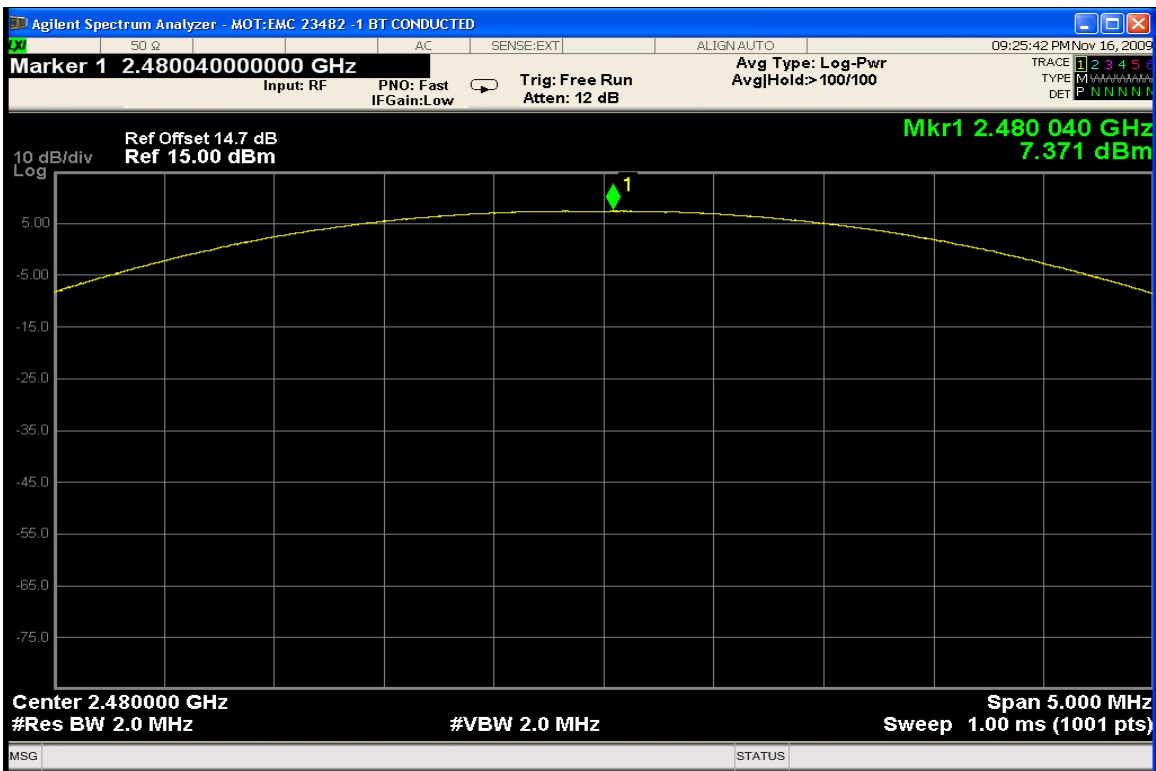
Peak Output Power – High Channel with EDR Enabled
