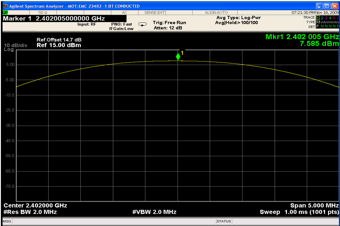
Peak Output Power – Low Channel with EDR Disabled
