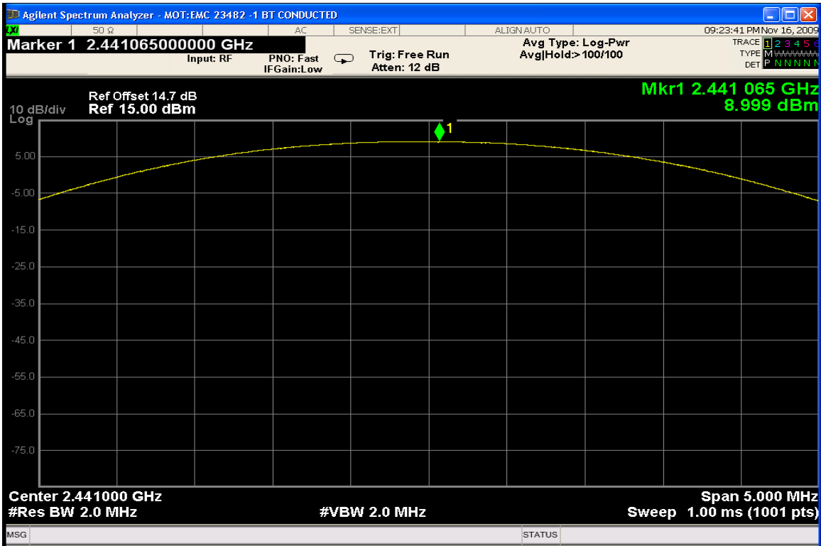
Peak Output Power – Mid Channel with EDR Enabled
