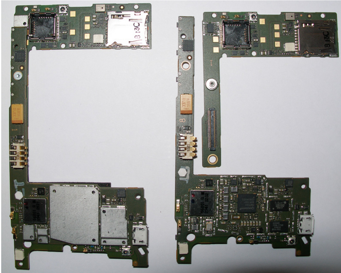
PCB Side 2 With Shields
