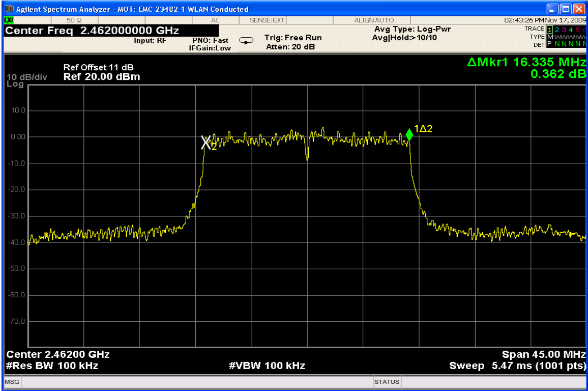
6dB Bandwidth Channel 11 @ 54Mbps
