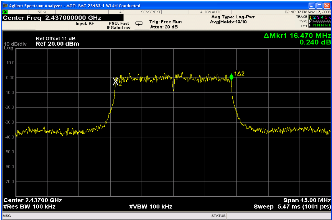
6dB Bandwidth Channel 6 @ 54Mbps
