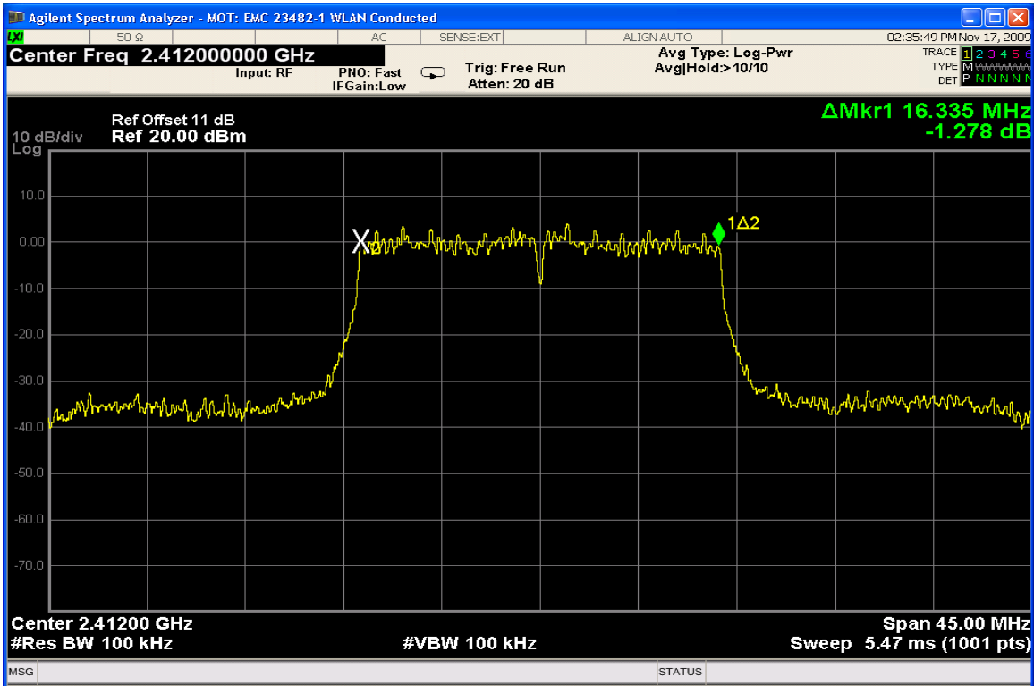
6dB Bandwidth Channel 1 @ 54Mbps
