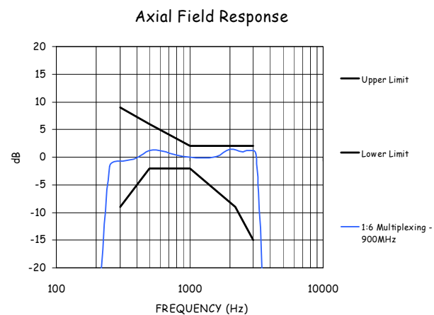
Figure 9-1-4: 900 MHz Measured Frequency Response (1:6).
