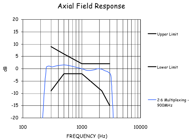
Figure 9-1-3: 900 MHz Measured Frequency Response (2:6).
