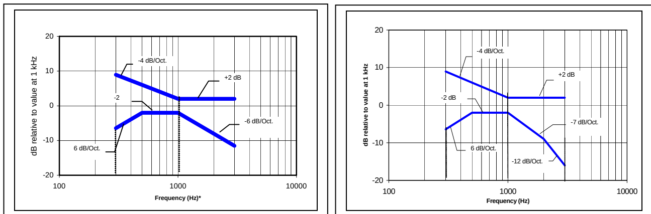
B – Mask for WDs with a field that exceeds -15 dB (A/m) at 1kHz
