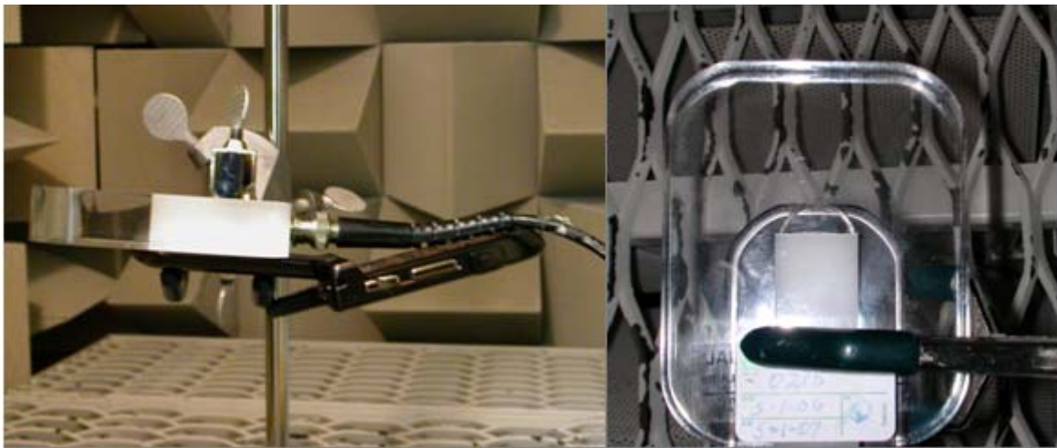
Figure 7-1 – Test holder
