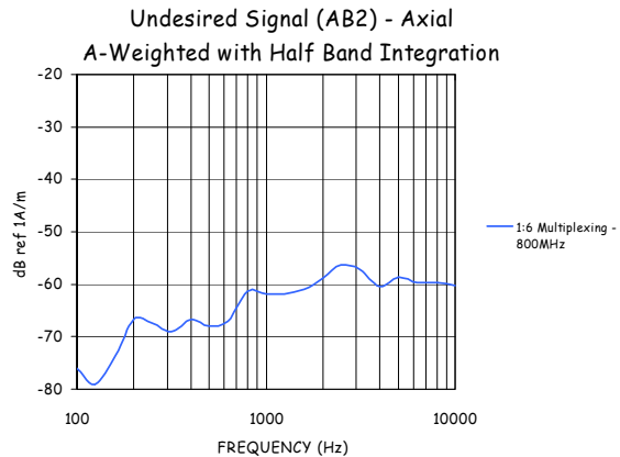
Figure 9-2-2: 800 MHz Undesired Signal (1:6).
