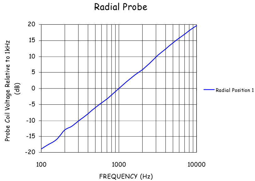
Figure 6-1-2 - Radial Probe sensitivity at 1000 Hz: -60.5 dB V/(A/m)
