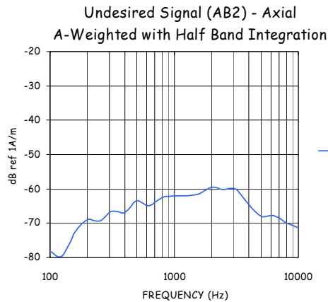
Figure 9-2-1: 800 MHz Undesired Signal (2:6).
