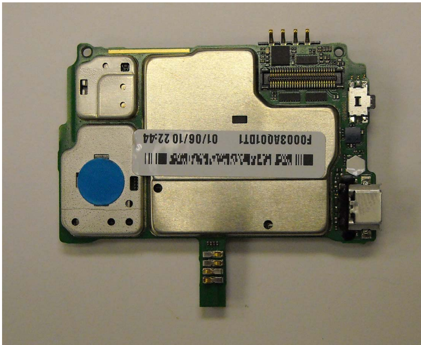
Photograph 9-5: Front side view of PC Board, Shields in place.
