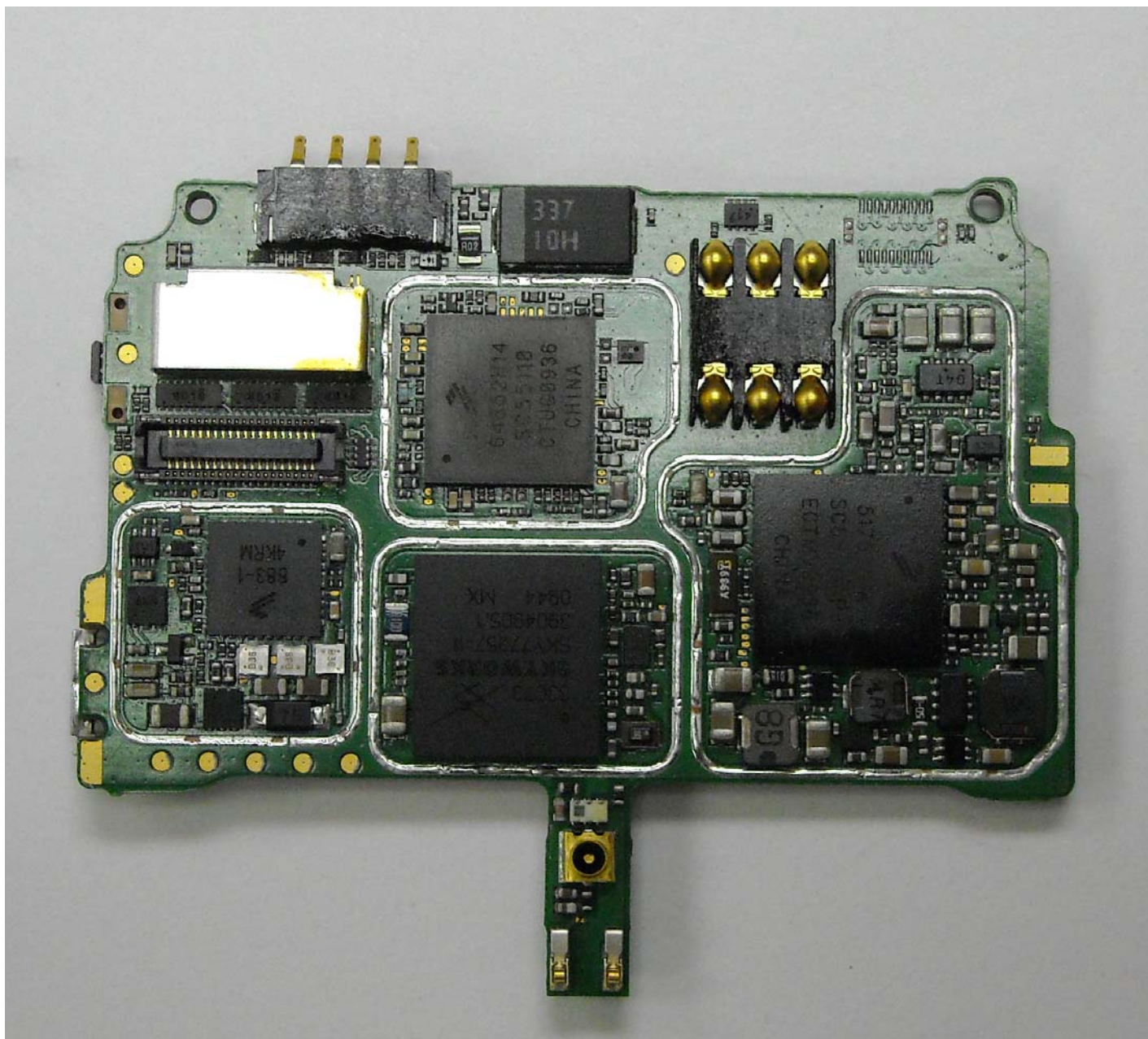
Photograph 9-4: Back side view of PC Board, Shields removed.
