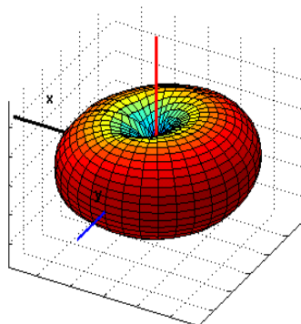
Figure 6b.6-1 Antenna pattern in the 900 MHz ISM frequency band.
