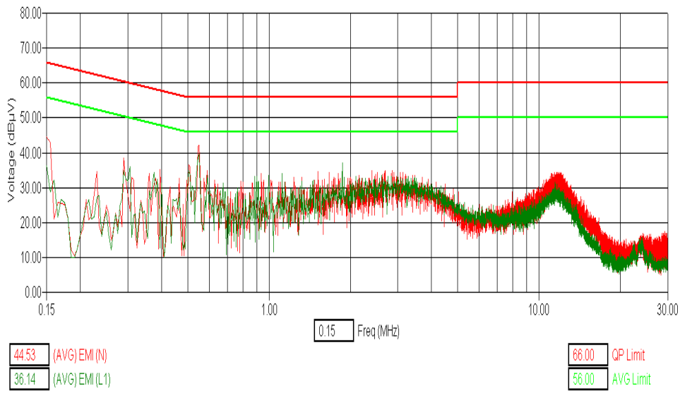
Bluetooth – Hopping - Tx Mode – AVG Detector
