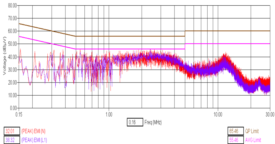
Bluetooth – Hopping - Tx Mode – Peak Detector
