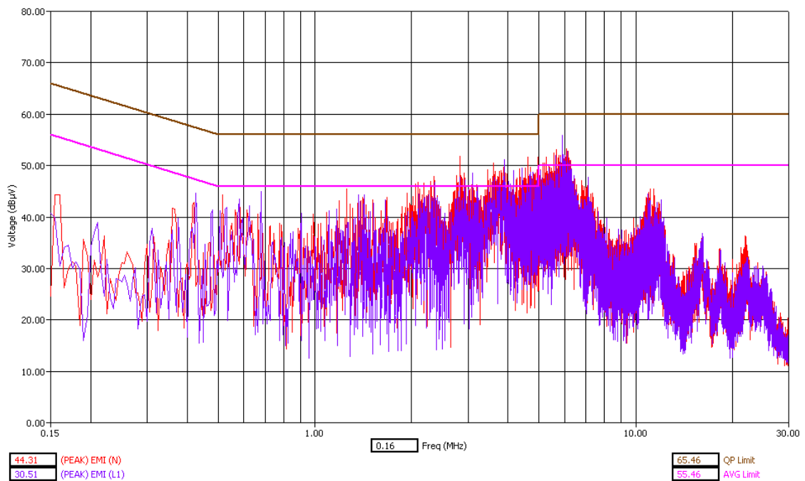
WLAN Channel 6 - Tx Mode - Peak Detector
