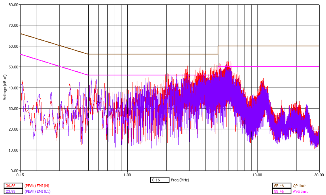
WLAN Channel 11 - Tx Mode - Peak Detector
