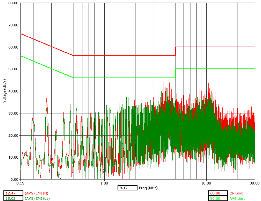
WLAN Channel 6 - Tx Mode - AVG Detector
