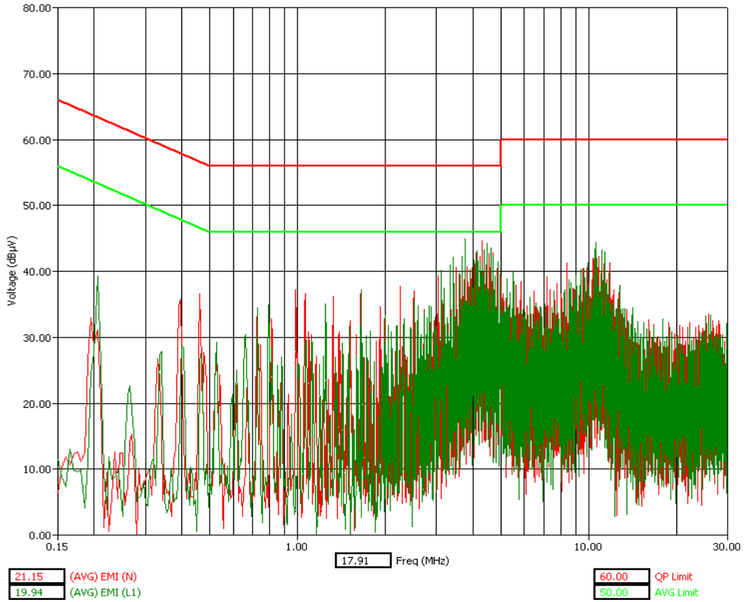
WLAN Channel 1 - Tx Mode - AVG Detector
