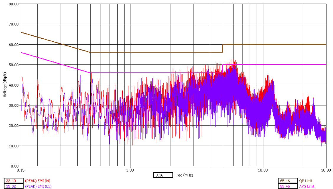
WLAN Channel 6 - Tx Mode - Peak Detector
