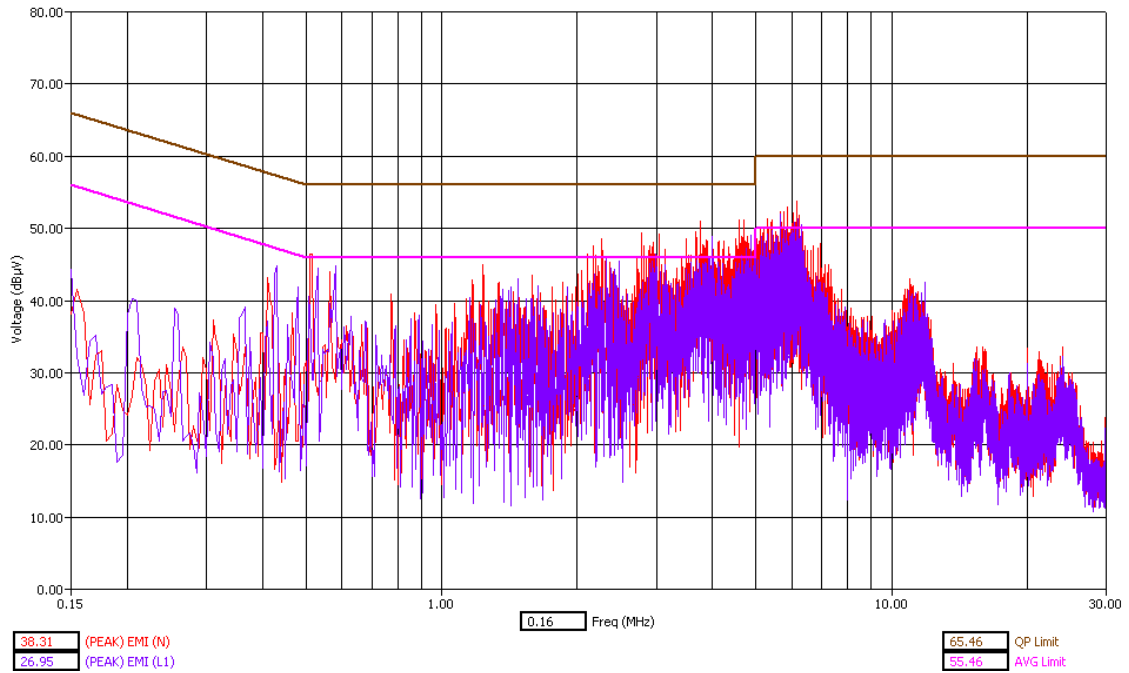
WLAN Channel 1 - Tx Mode - Peak Detector
