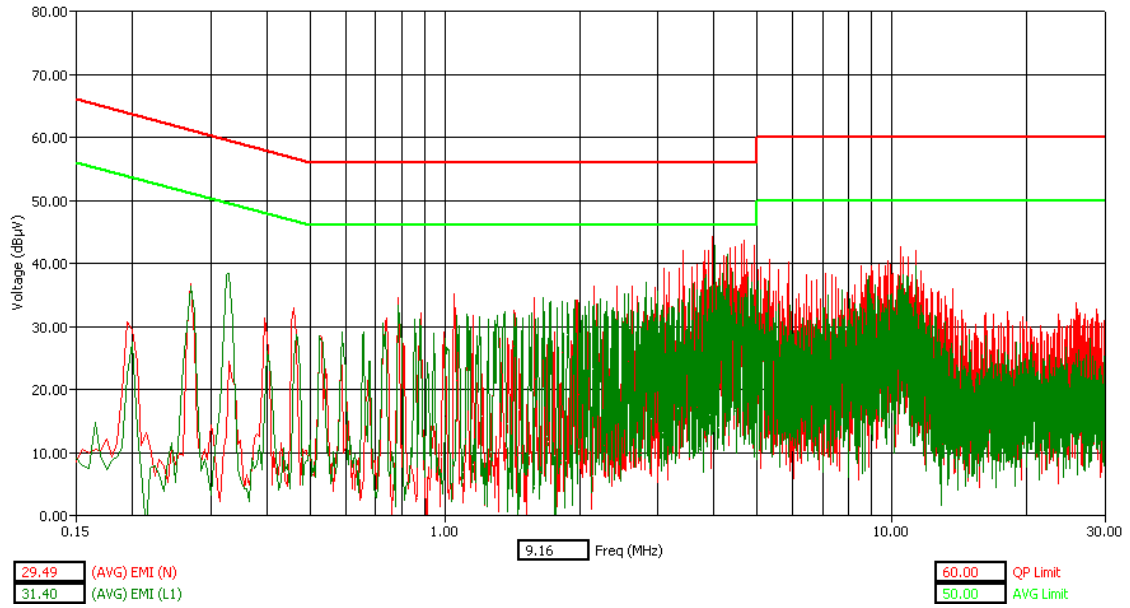
WLAN Channel 1 - Tx Mode - AVG Detector
