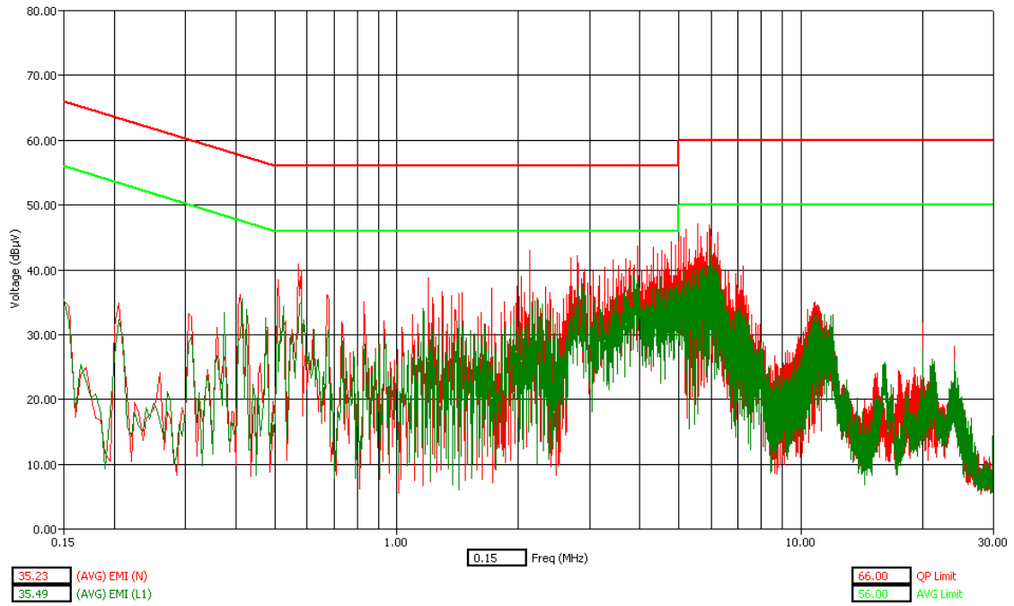
WLAN Channel 11 - Tx Mode - AVG Detector
