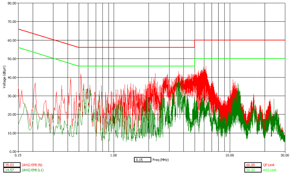
WLAN Channel 6 - Tx Mode - AVG Detector
