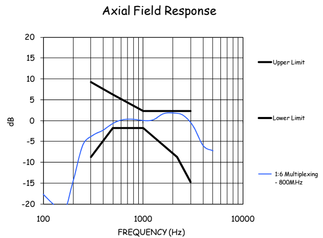
Figure 9-1-2: 800 MHz Measured Frequency Response (1:6).
