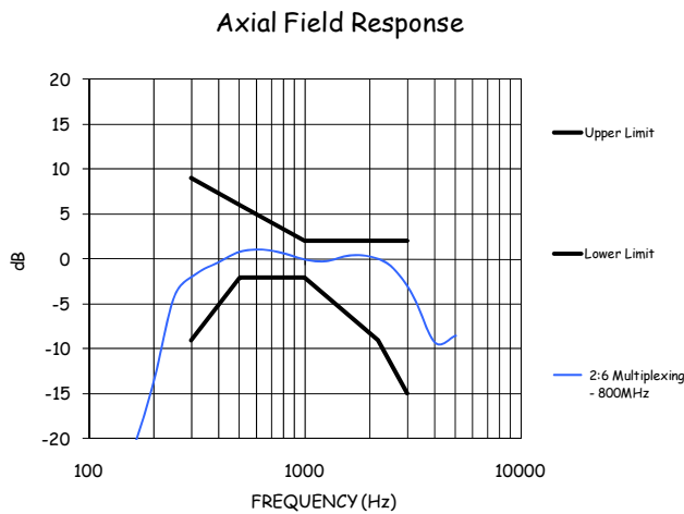
Figure 9-1-1: 800 MHz Measured Frequency Response (2:6).
