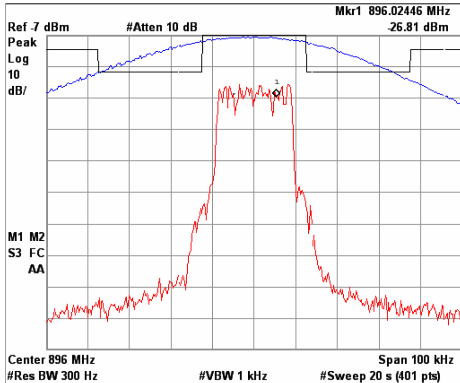
Figure 6a.2.2-12. iDEN 900 MHz Band, Quad-64QAM, Minimum Power, EA Emission Mask
