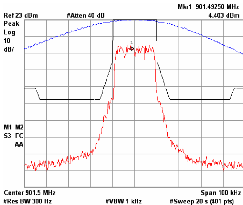
Figure 6b.2.1-2. iDEN NBPCS Band, Occupied Bandwidth, Quad-16QAM, Maximum Power.
