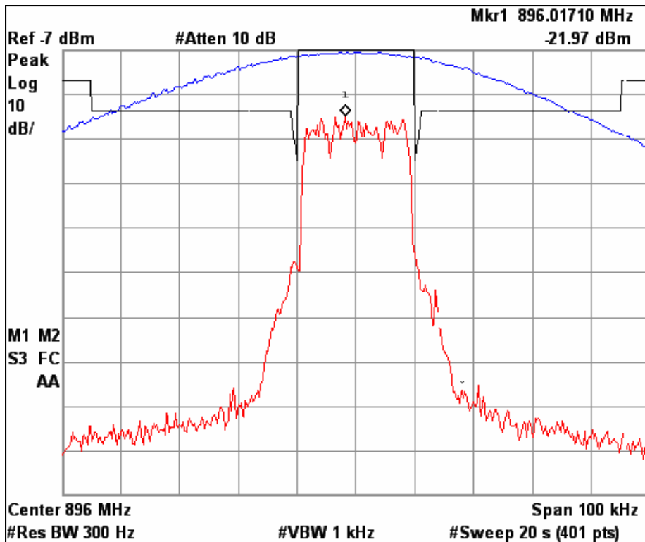
Figure 6a.2.2-10. iDEN 900 MHz Band, Quad-64QAM, Minimum Power, Emission Mask G
