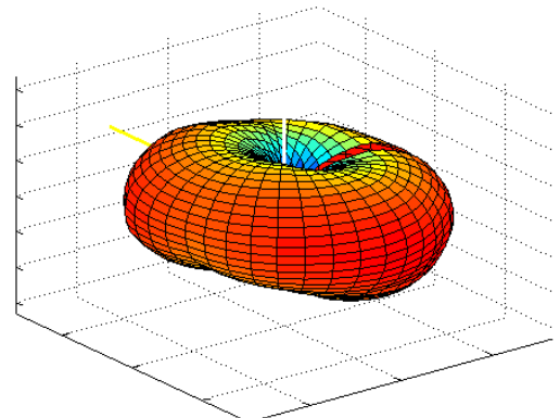
Figure 6a.6-3 Antenna pattern in the 900 MHz SMR frequency band (Flip Closed).
