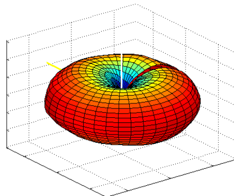
Figure 6a.6-2 Antenna pattern in the 800 MHz SMR frequency band (Flip Closed).
