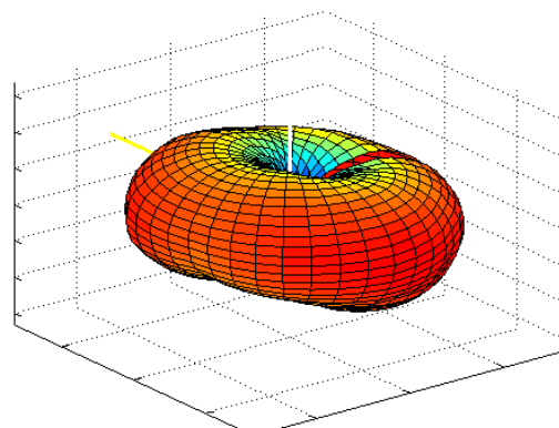
Figure 6a.6-6 Antenna pattern in the 900 MHz NBPCS frequency band (Flip Closed).
