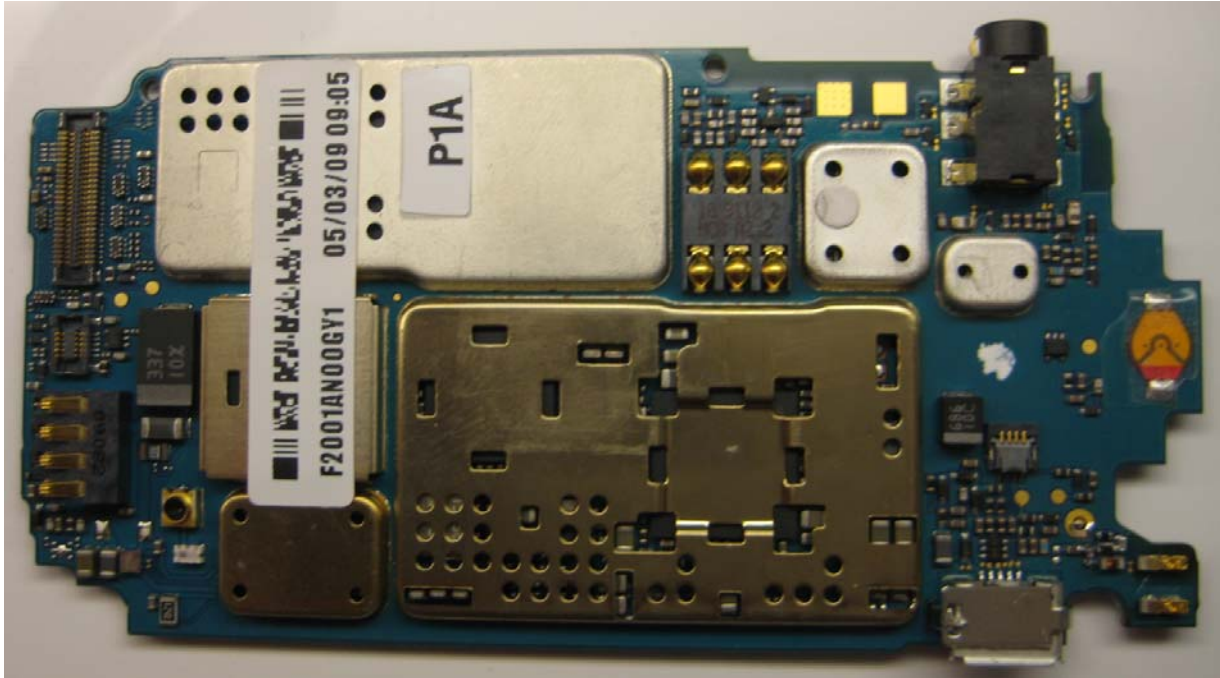
Photograph 9-1: Component side view of radio product PC Board, Shields in place.
