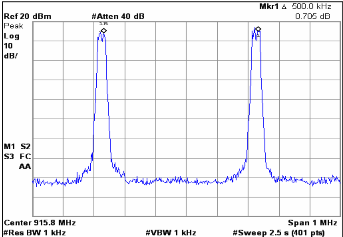
Figure 6b.2.1.1. Plot of MOTotalk ISM Band adjacent channel separation within a hop set.
