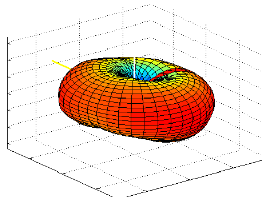
Figure 6b.5-2 Antenna pattern in the 800 MHz SMR frequency band (Flip Closed).
