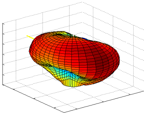
Figure 6b.5-1 Antenna pattern in the 800 MHz SMR frequency band (Flip Open).
