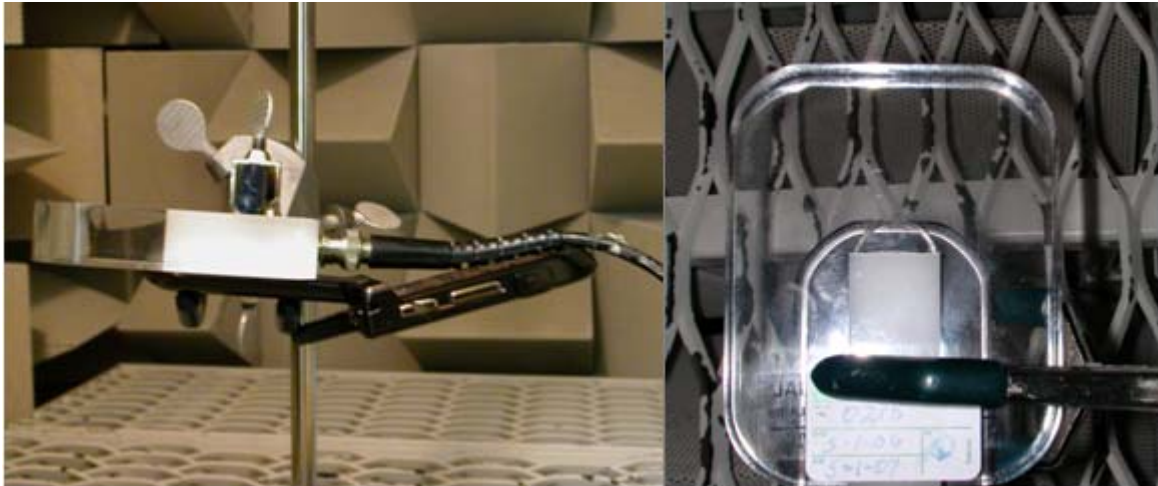
Figure 7-1 – Test holder
