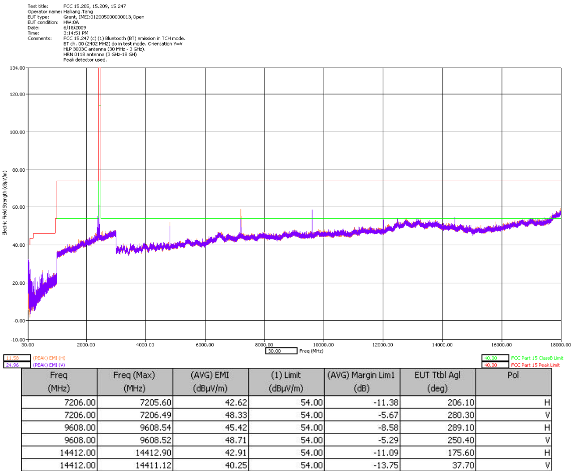
30 MHz – 18 GHz Low Channel Dual Polarization Y
