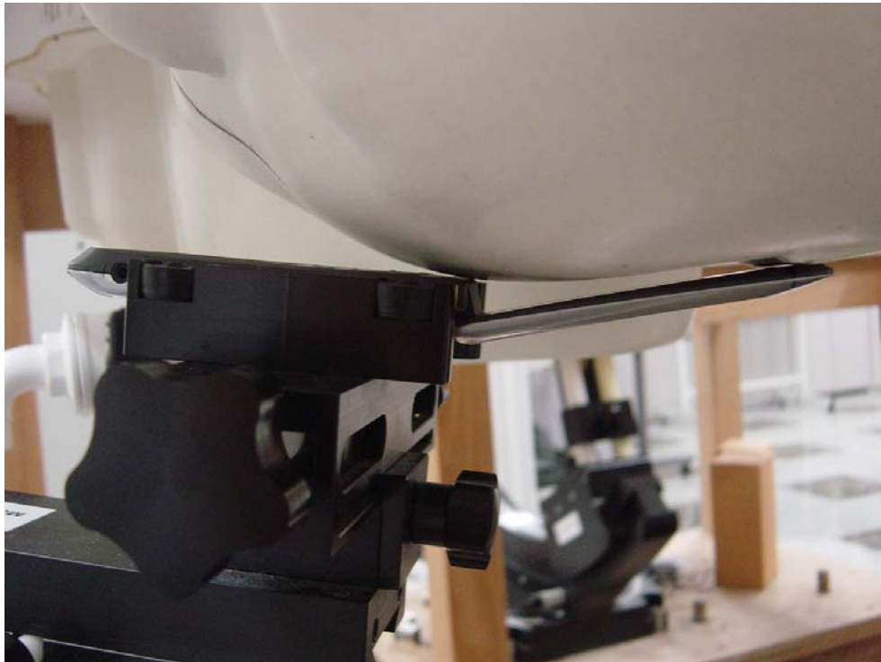
Figure 5: Phone Against the Head Phantom (Cheek Touch)
