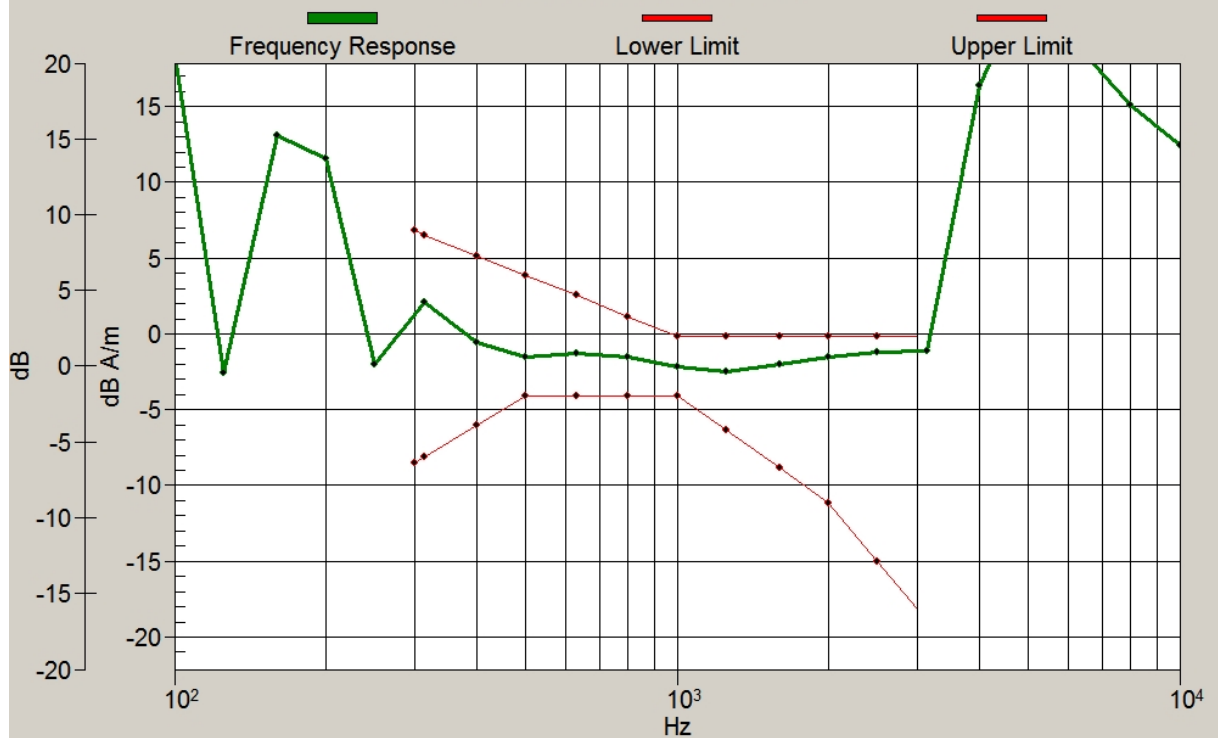
Graph 3: GSM 850 Frequency Response with Battery 2 GSM 850 Frequency Response with SNN5813A Loc: -2, 1.1, 3.7 mm Diff: 1.03dB
