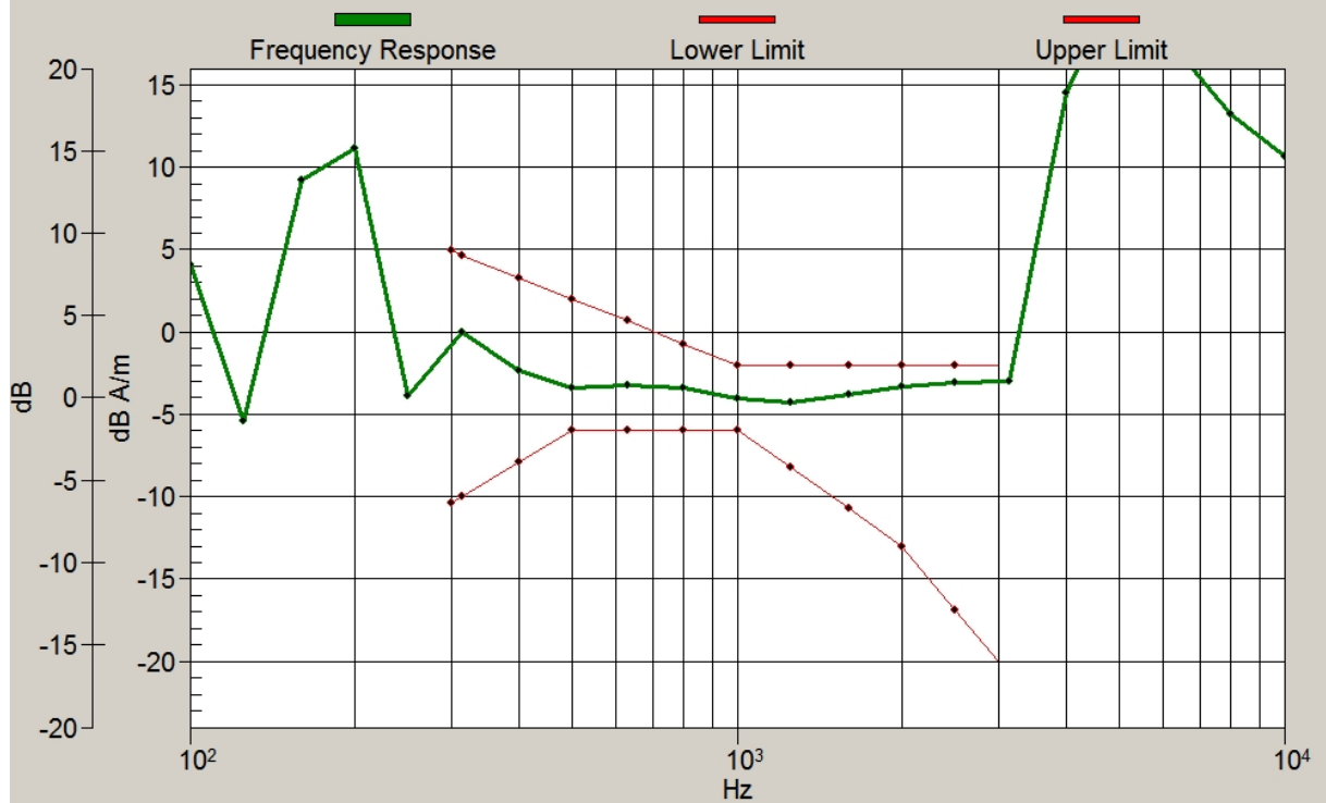
Graph 2: GSM 850 Frequency Response GSM 850 Frequency Response with SNN5804B Loc: -2.7, 4.3, 3.7 mm Diff: 1.03dB
