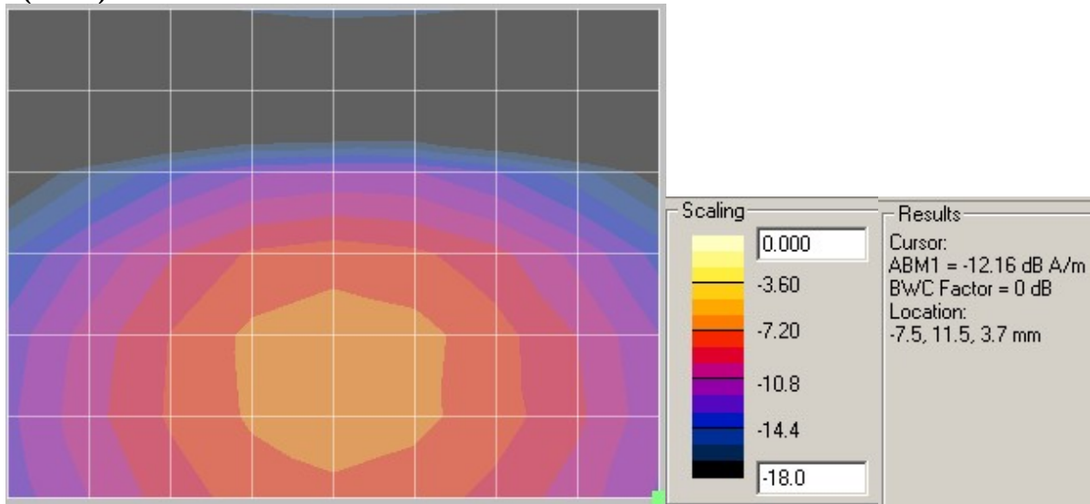
Y(Radial) ABM1
