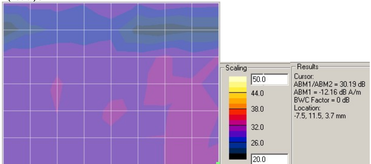
Y(Radial) SNR
