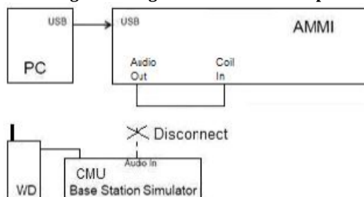
Figure 2: Signal Verification Setup
