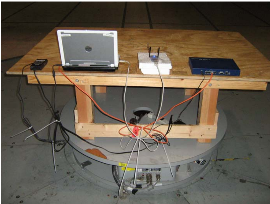
Radiated Emissions Test Setup – Back View
