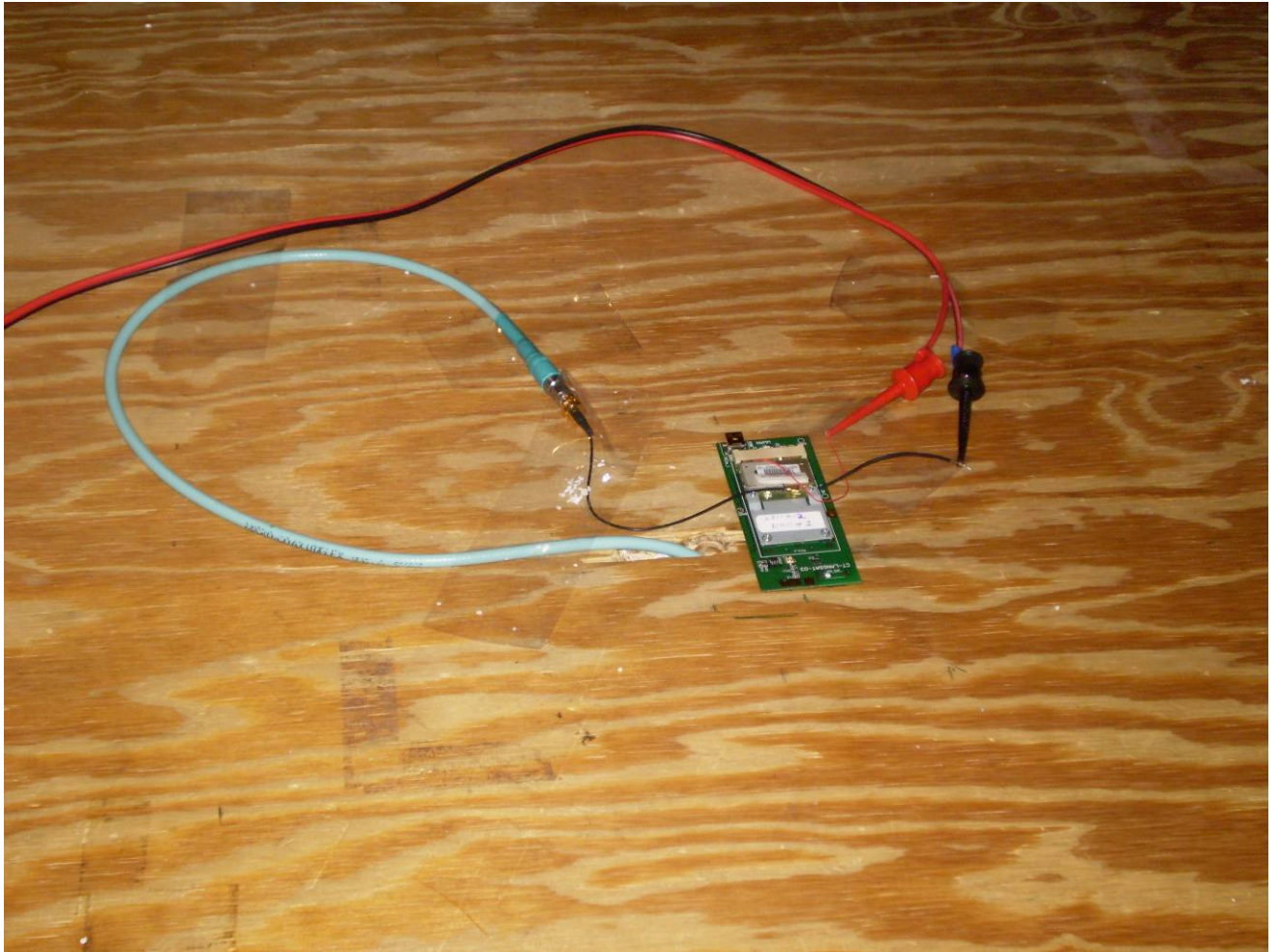
Radiated Emissions
