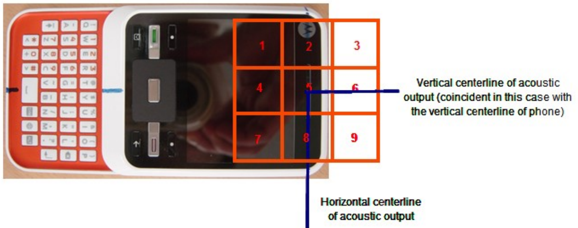
Figure 5. Phone Open - Orientation and Measurement Plane for RF Emissions Testing
