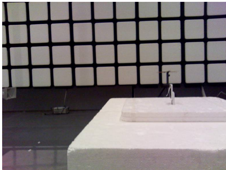
23101-1, IHDP56KH1 setup in semi-anechoic chamber – right view (18 GHz – 26.5 GHz)
