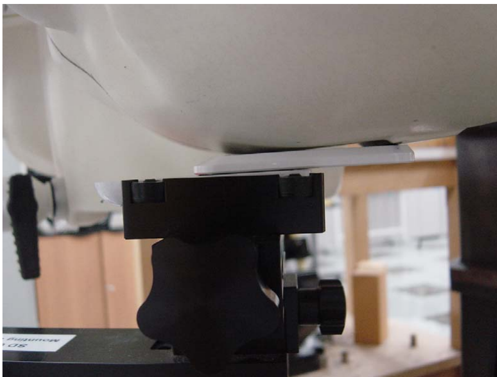
Figure 6: Phone Against the Head Phantom (Cheek Touch – Slider Up)
