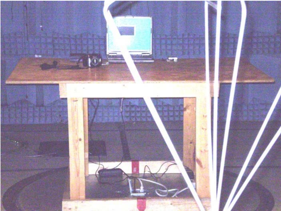
EMC Report #23101 Part 15, PC Peripheral
