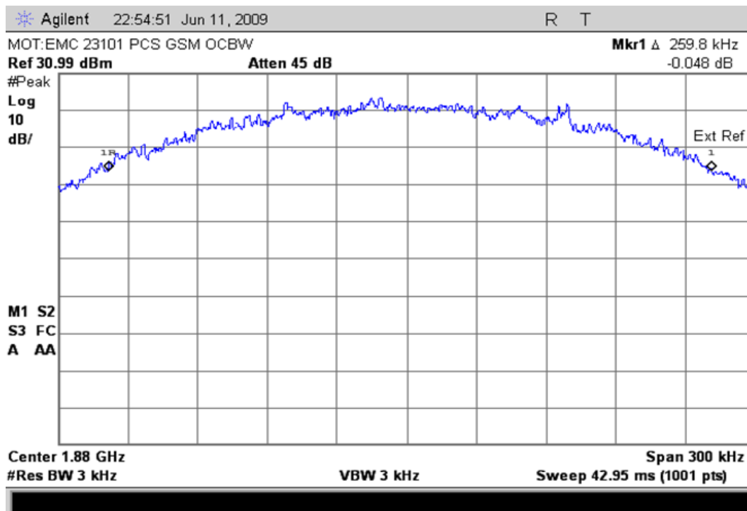
GSM 1900 – Occupied Bandwidth – Channel 661 (1880.00MHz)
