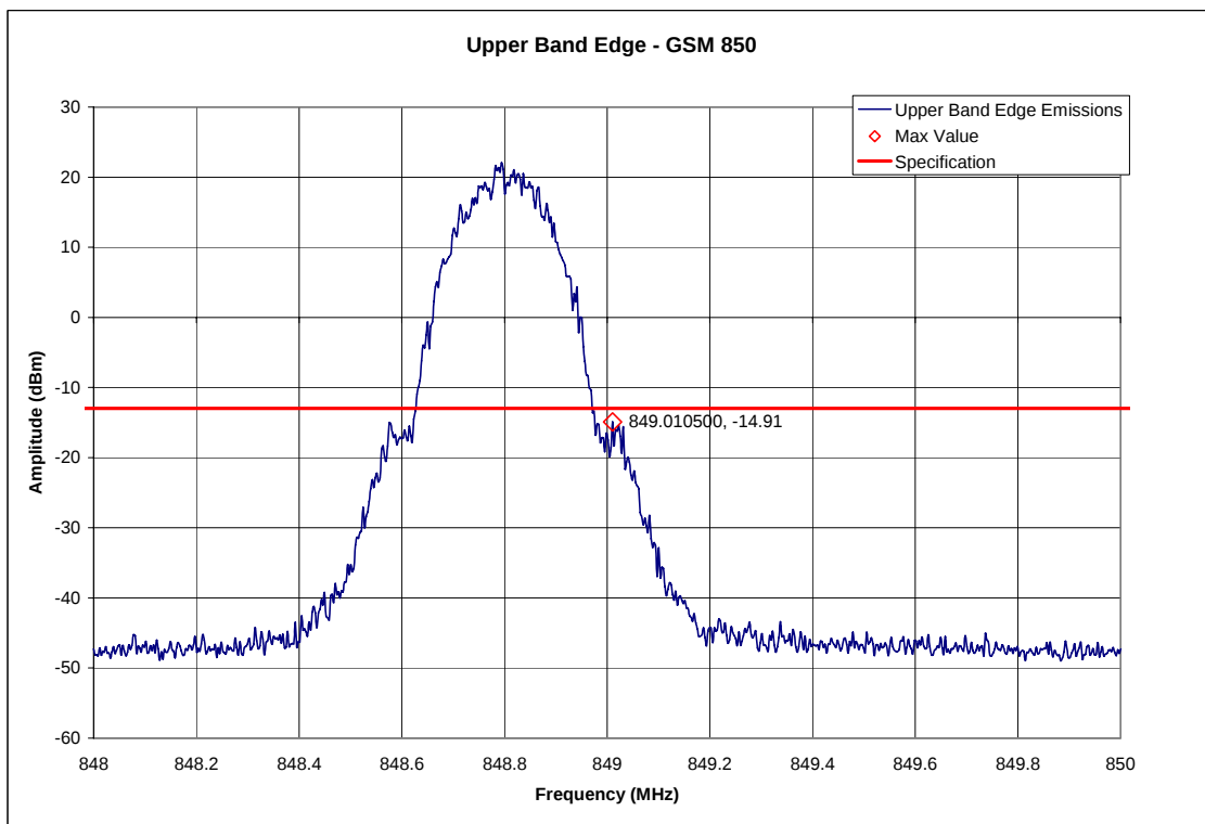
GSM 850 – Upper Band Edge – Channel 251 (848.8 MHz)
