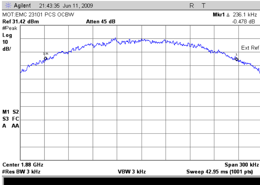
GSM 1900 EDGE – Occupied Bandwidth – Channel 661 (1880.00MHz)
