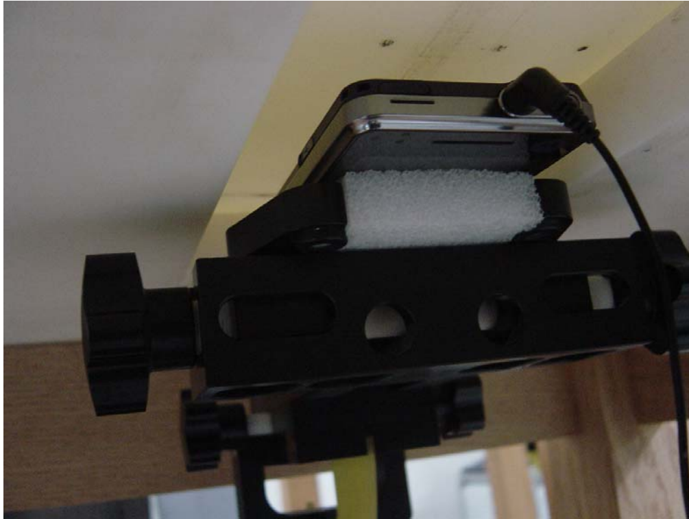
Figure 5: Back of Phone Against the Flat Phantom (15 mm separation)
