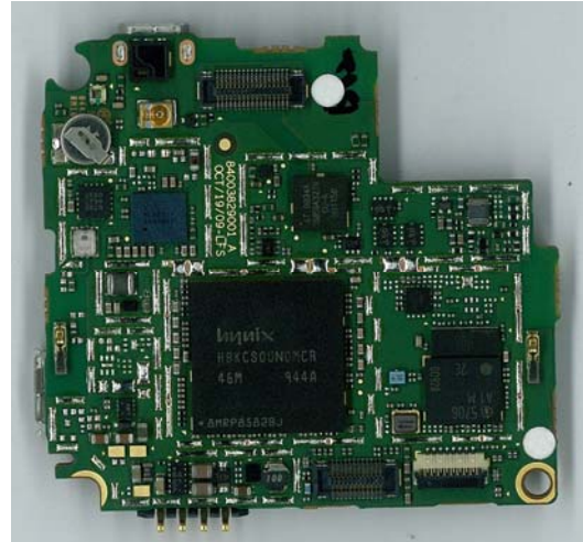
Main Board Top Without shields
