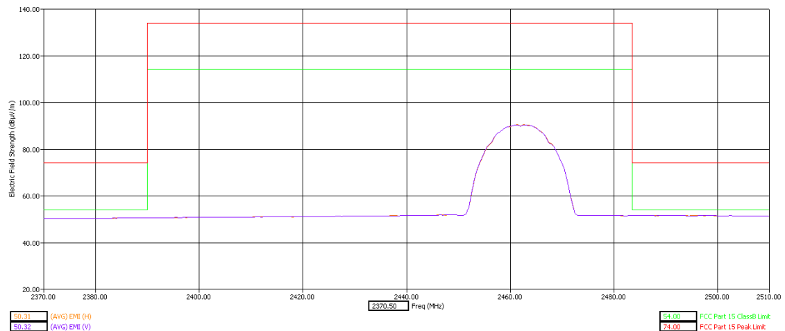
High Band Edge X Orientation – slider closed
