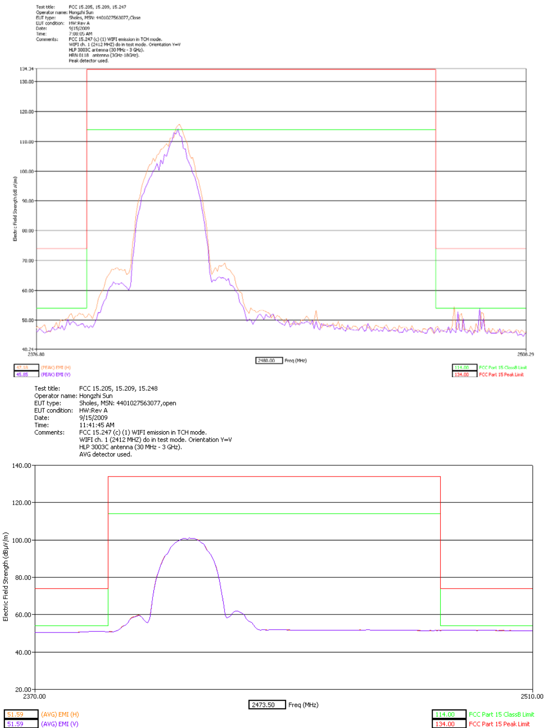
Low Band Edge Y Orientation – slider closed
