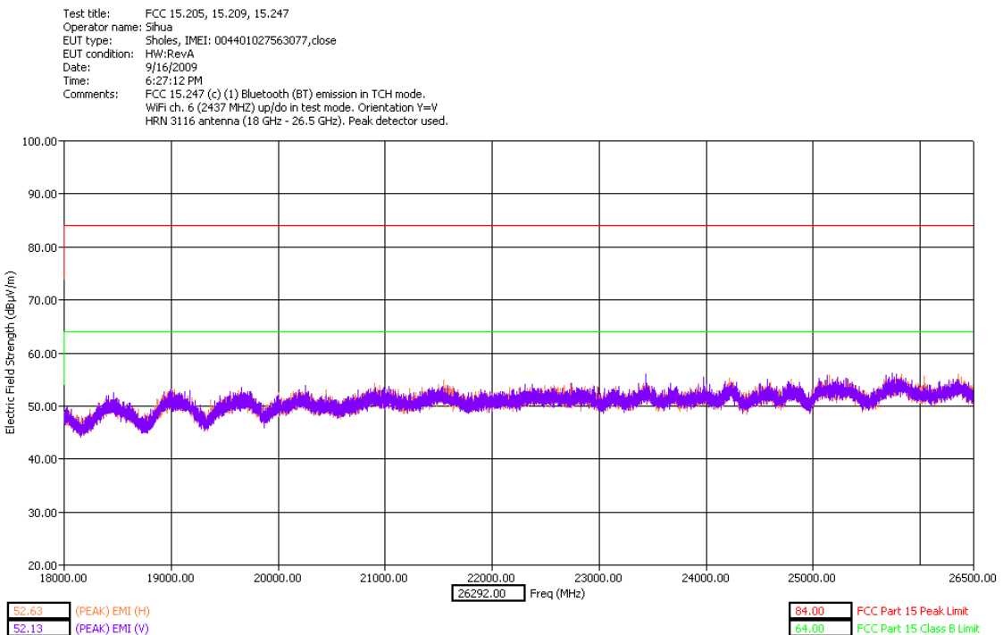
18 – 26.5 GHz Middle Channel Dual Polarization Y – slider closed
