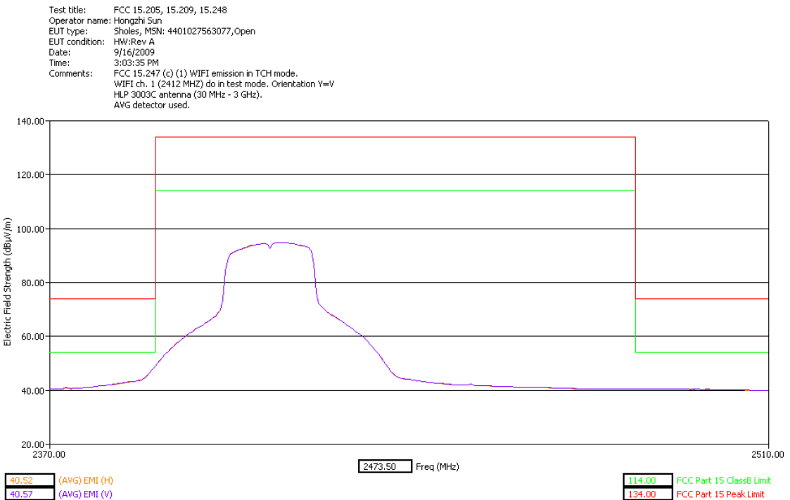
Low Band Edge Y Orientation – slider open
