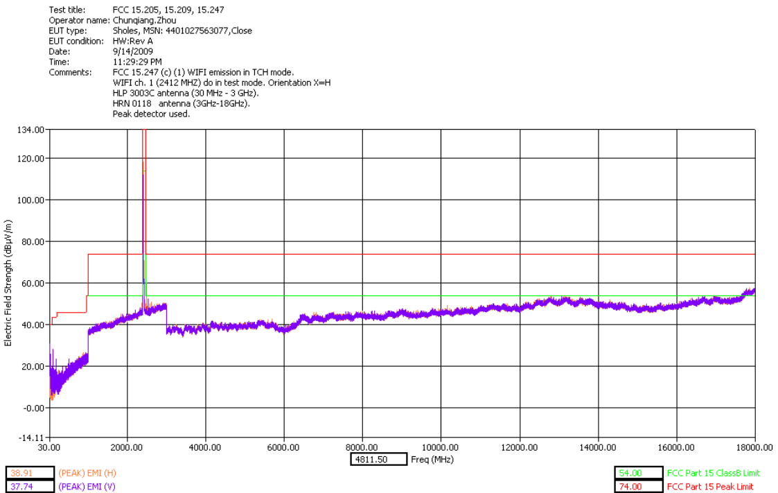
30 - 18000MHz Low Channel Dual Polarization X - slider closed
