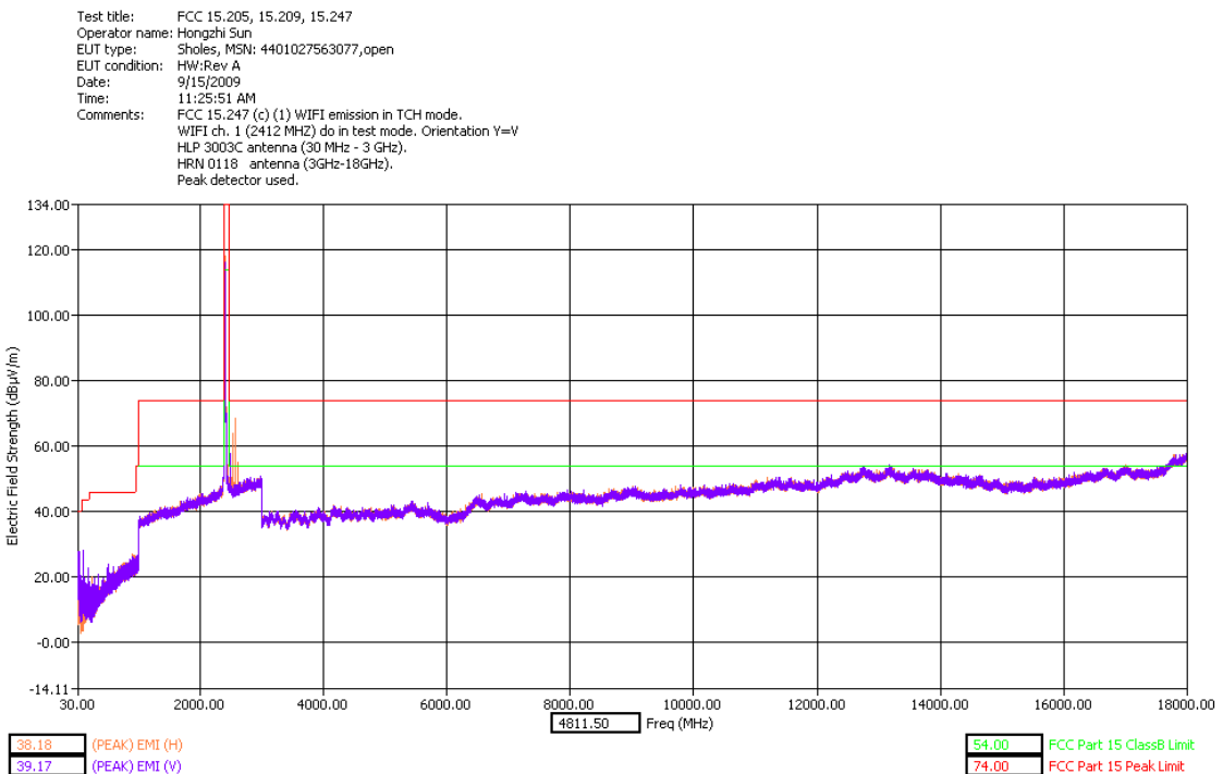
30 - 18000MHz Low Channel Dual Polarization Y - slider open
