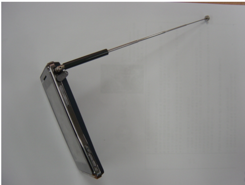
Figure 14: Phone with DMB Antenna Position 4 Extended
