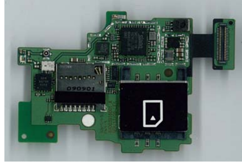
Daughter Board Top Without Shields
