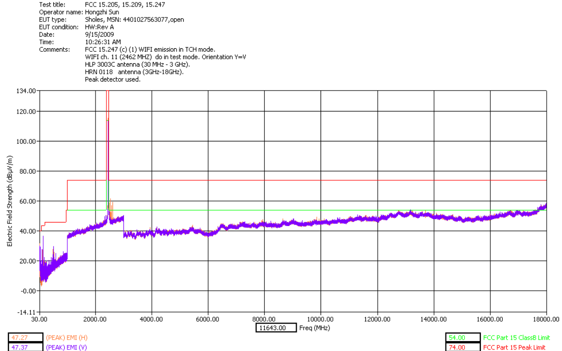
30 - 18000MHz High Channel Dual Polarization Y - slider open
