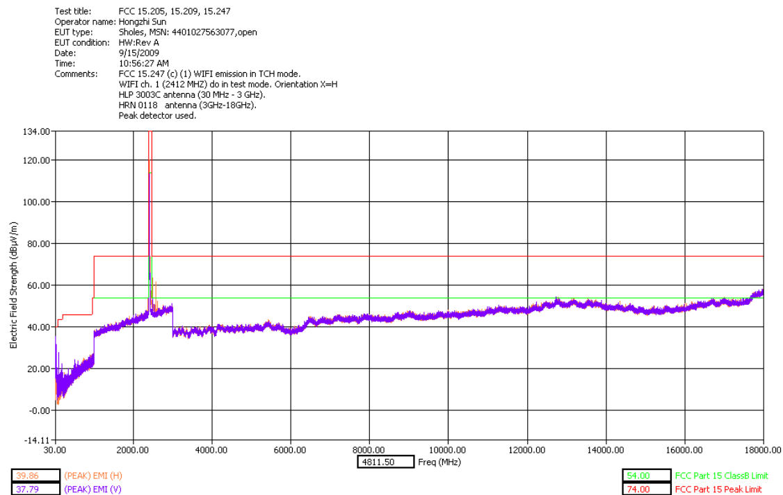
30 - 18000MHz Low Channel Dual Polarization X - slider open
