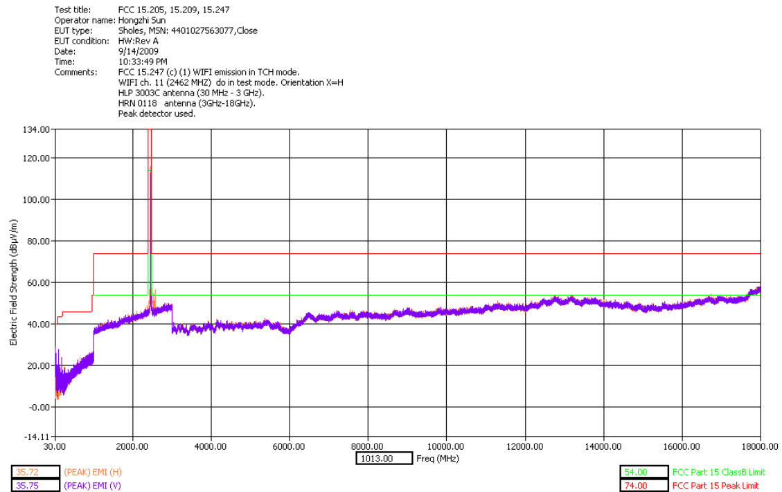
30 - 18000MHz High Channel Dual Polarization X - slider closed
