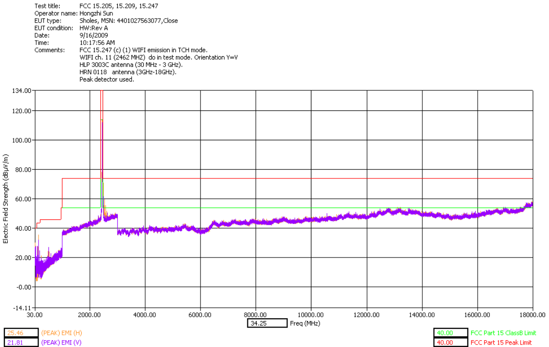
30 - 18000MHz High Channel Dual Polarization Y - slider closed
