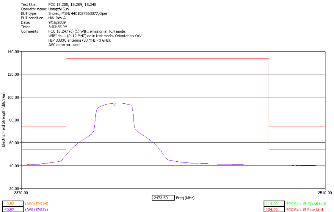
Low Band Edge Y Orientation – slider closed
