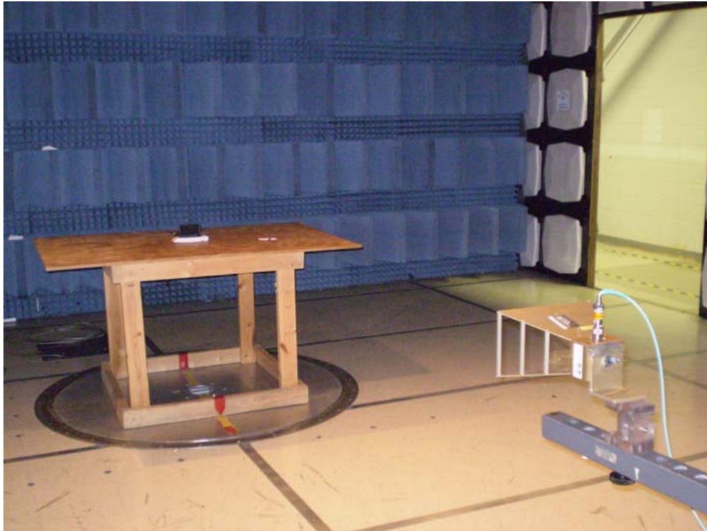
EMC Report #23164 Tx Radiated
