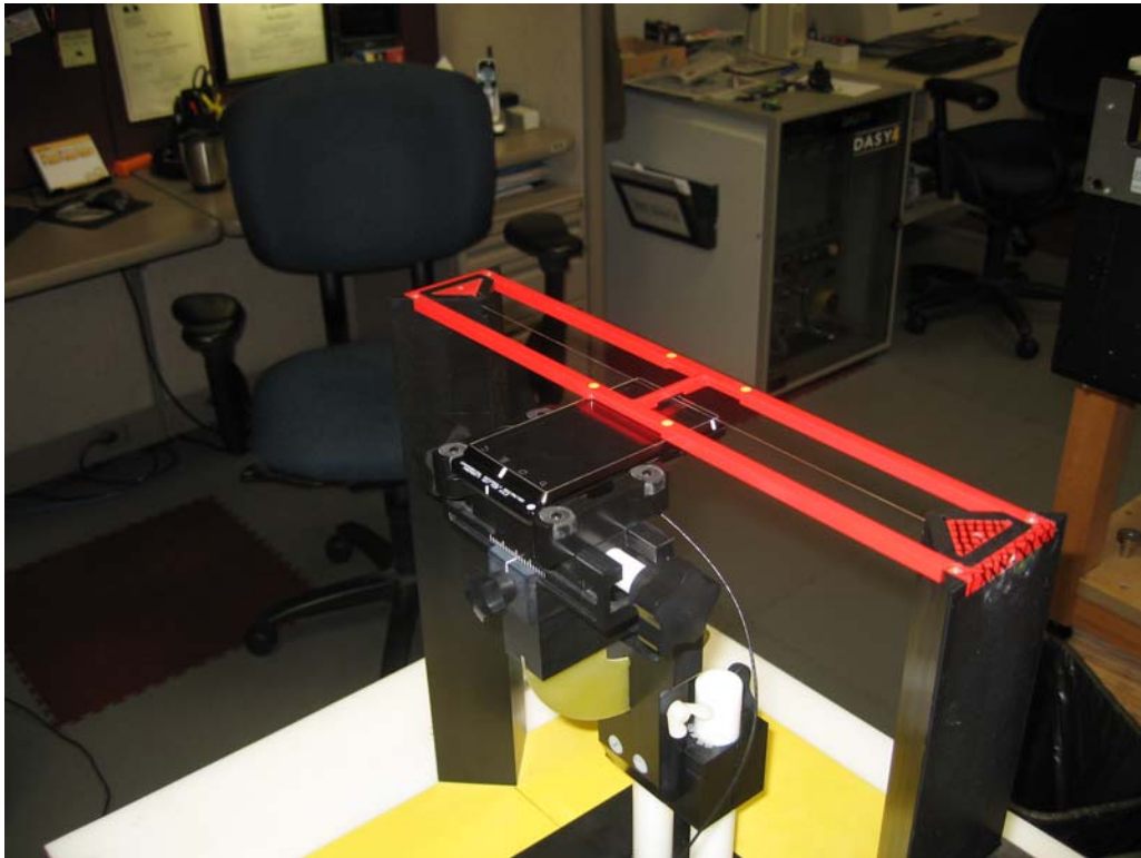
Figure 5. Positioning and Measurement for Telecoil Emissions
