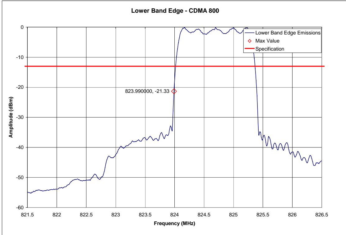
DMA 800 – Lower Band Edge – Channel 1013 (824.702MHz)
